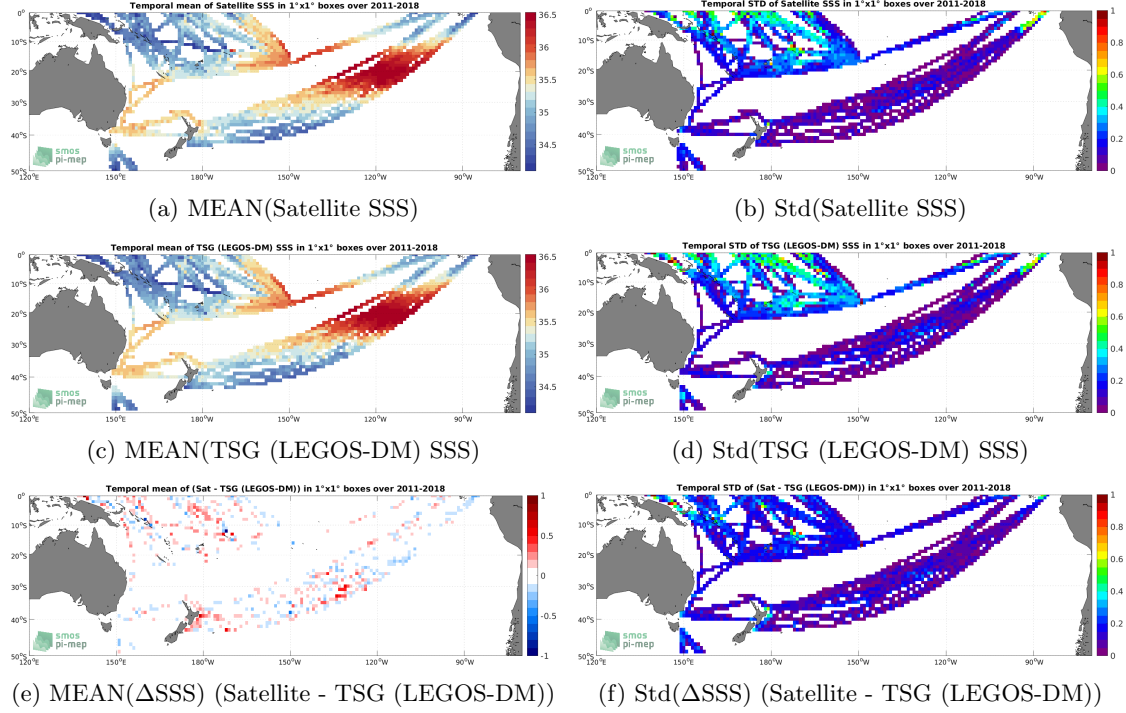
Figure 6: Temporal mean (left) and Std (right) of SSS from SMOS and SMAP SSS L4 OI v1 - 7 Days (LOPS) (top), TSG (LEGOS-DM) (middle), and of \Delta\text{SSS} (Satellite - TSG (LEGOS-DM)). Only match-up pairs are used to generate these maps.
