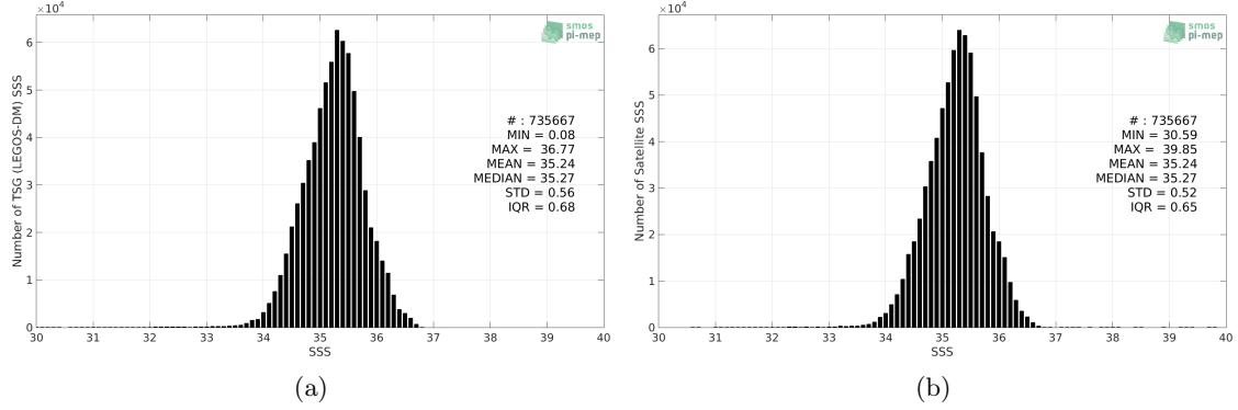
Figure 2: Histograms of SSS from TSG (LEGOS-DM) (a) and SMOS and SMAP SSS L4 OI v1 - 7 Days (LOPS) (b) considering all match-up pairs per bins of 0.1 over the South Pacific Ocean Pi-MEP region and for the full satellite product period.
