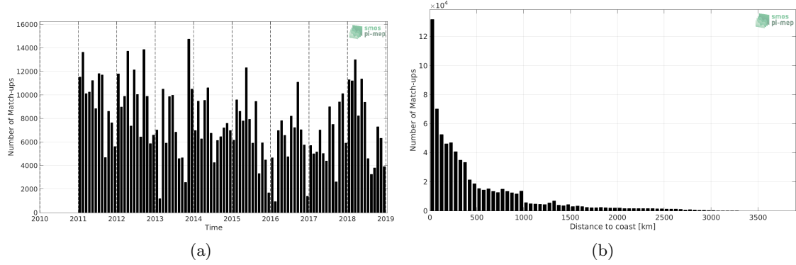
Figure 1: Number of match-ups between TSG (LEGOS-DM) and SMOS and SMAP SSS L4 OI v1 - 7 Days (LOPS) SSS as a function of time (a) and as function of the distance to coast (b) over the South Pacific Ocean Pi-MEP region and for the full satellite product period.
