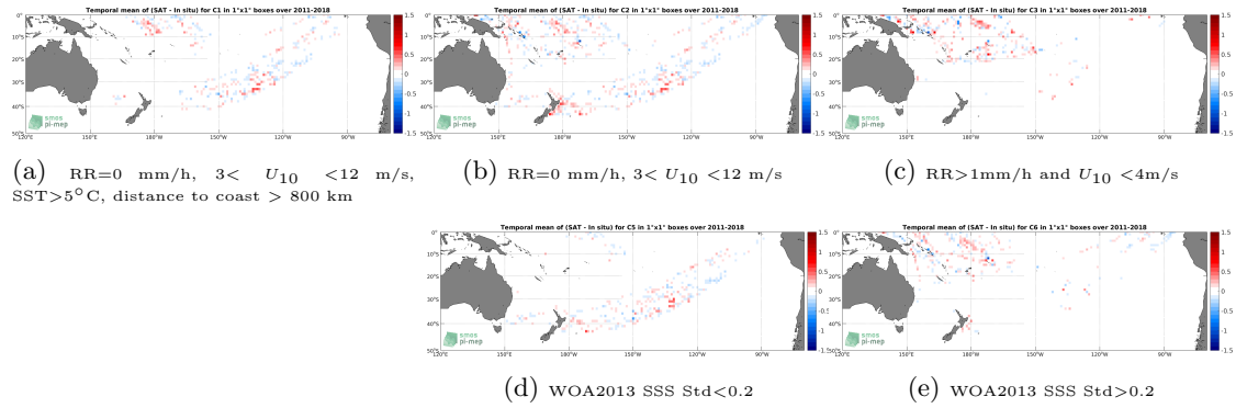
Figure 12: Temporal mean gridded over spatial boxes of size 1^\circ \times 1^\circ of \Delta SSS (SMOS and SMAP SSS L4 OI v1 - 7 Days (LOPS) - TSG (LEGOS-DM)) for 5 different subdatasets corresponding to: RR=0 mm/h, 3 < U_{10} < 12 m/s, SST > 5^\circ\text{C} , distance to coast > 800 km (a), RR=0 mm/h, 3 < U_{10} < 12 m/s (b), RR > 1 mm/h and U_{10} < 4 m/s (c), WOA2013 SSS Std < 0.2 (d), WOA2013 SSS Std > 0.2 (e).
