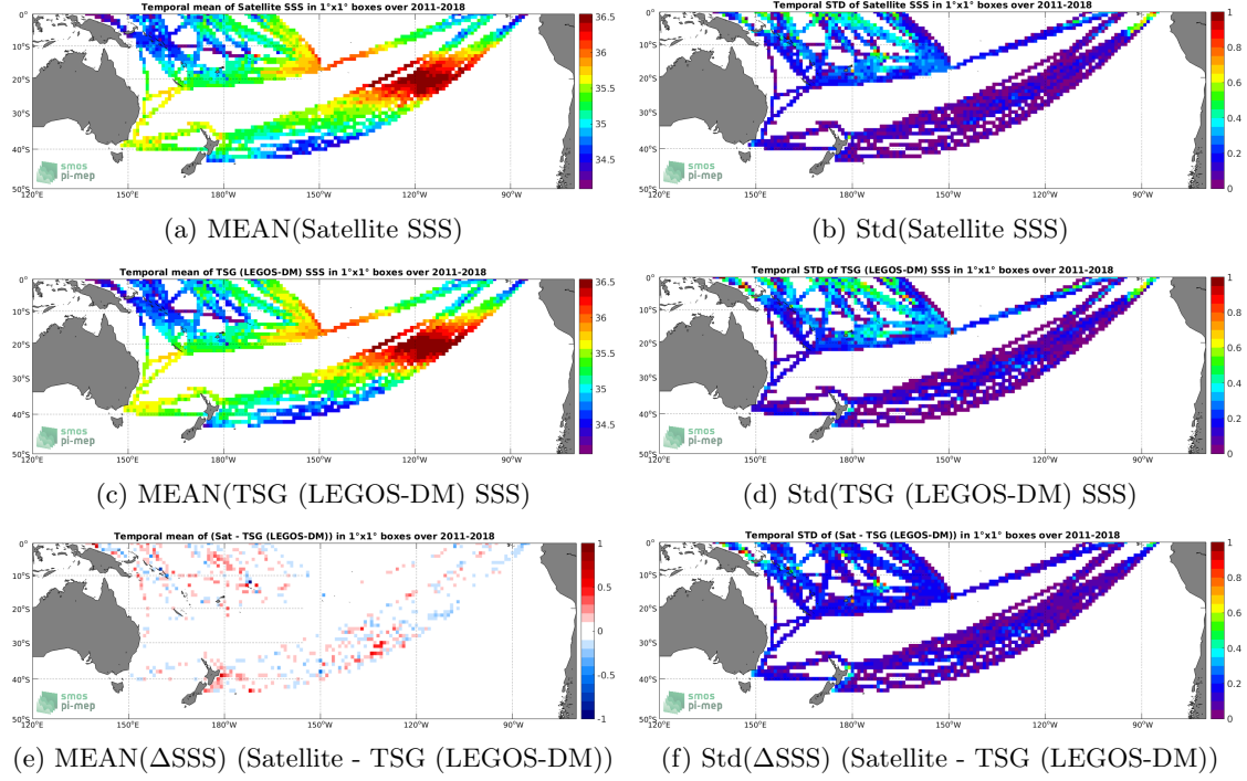
Figure 6: Temporal mean (left) and Std (right) of SSS from SMOS and SMAP SSS L4 OI v1 - 7 Days (LOPS) (top), TSG (LEGOS-DM) (middle), and of \Delta SSS (Satellite - TSG (LEGOS-DM)). Only match-up pairs are used to generate these maps.
