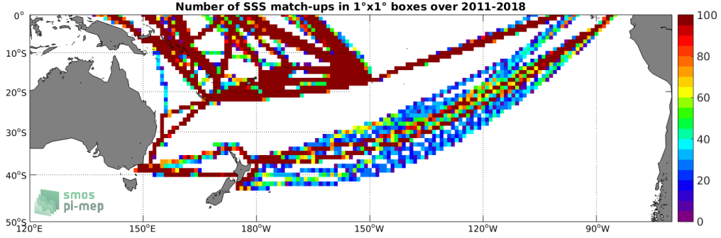
Figure 4: Number of SSS match-ups between TSG (LEGOS-DM) SSS and the SMOS and SMAP SSS L4 OI v1 - 7 Days (LOPS) SSS product for the South Pacific Ocean Pi-MEP region over 1^\circ \times 1^\circ boxes and for the full satellite product period.
