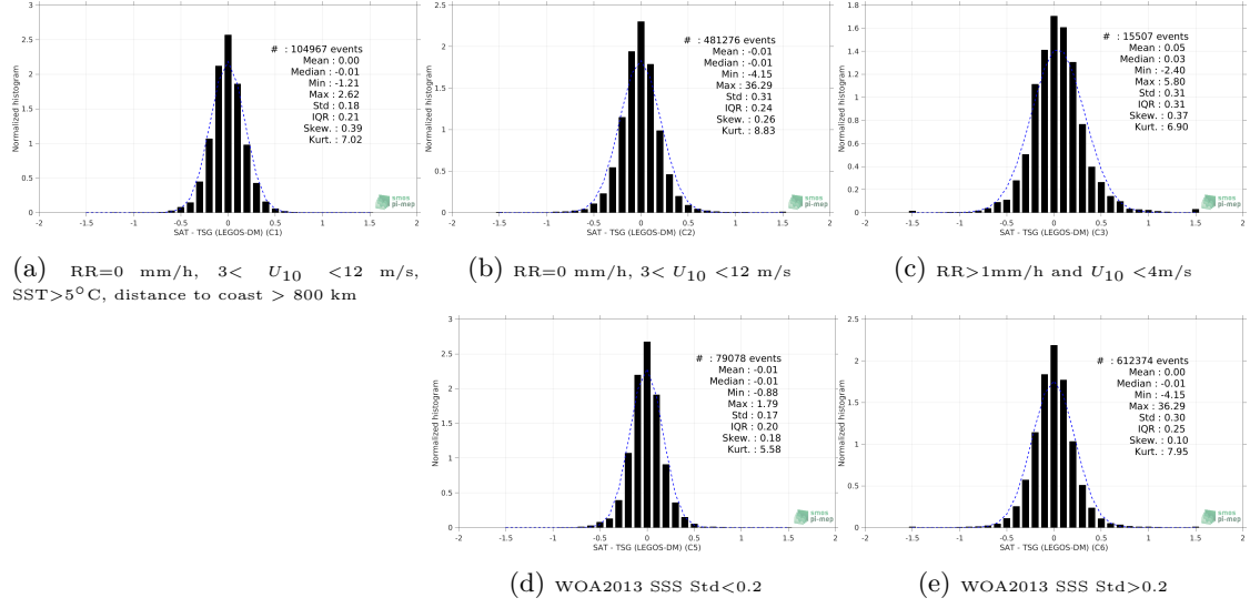
Figure 13: Normalized histogram of \Delta SSS (SMOS and SMAP SSS L4 OI v1 - 7 Days (LOPS) - TSG (LEGOS-DM)) for 5 different subdatasets corresponding to: RR=0 mm/h, 3 < U_{10} < 12 m/s, SST > 5^\circ\text{C} , distance to coast > 800 km (a), RR=0 mm/h, 3 < U_{10} < 12 m/s (b), RR > 1 mm/h and U_{10} < 4 m/s (c), WOA2013 SSS Std < 0.2 (d), WOA2013 SSS Std > 0.2 (e).
