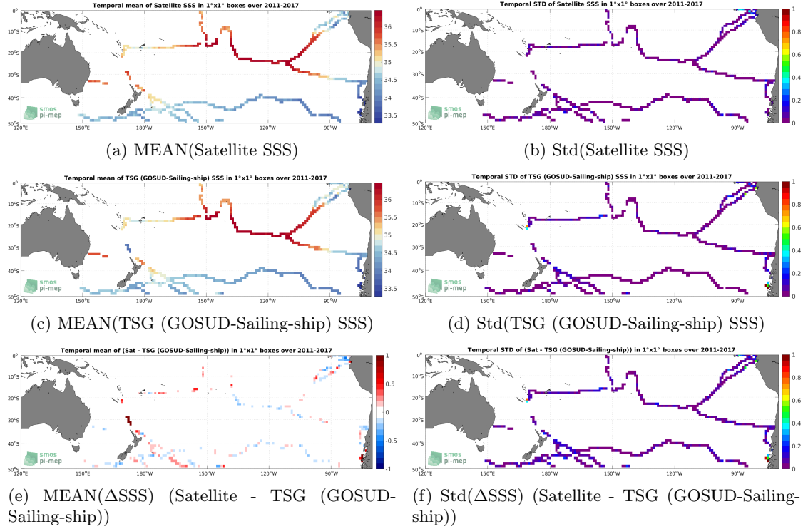
Figure 6: Temporal mean (left) and Std (right) of SSS from SMOS and SMAP SSS L4 OI v1 - 7 Days (LOPS) (top), TSG (GOSUD-Sailing-ship) (middle), and of \Delta SSS (Satellite - TSG (GOSUD-Sailing-ship)). Only match-up pairs are used to generate these maps.
