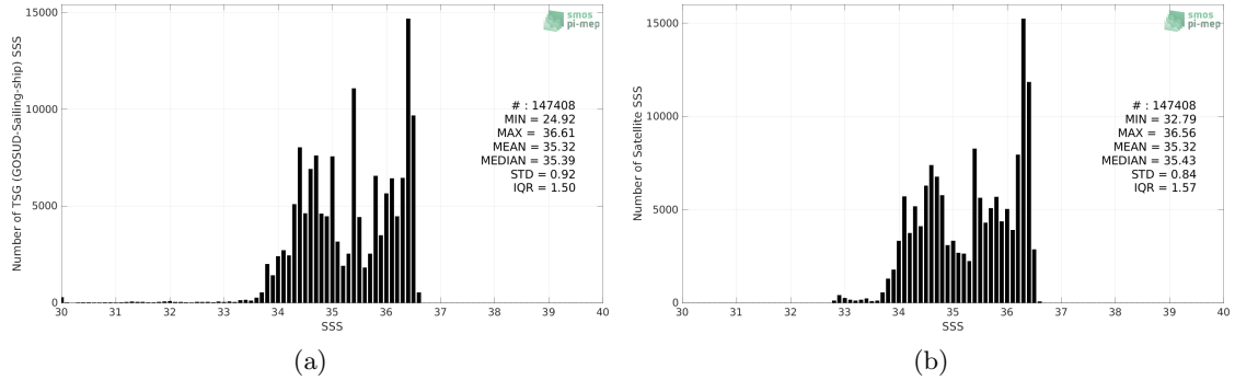
Figure 2: Histograms of SSS from TSG (GOSUD-Sailing-ship) (a) and SMOS and SMAP SSS L4 OI v1 - 7 Days (LOPS) (b) considering all match-up pairs per bins of 0.1 over the South Pacific Ocean Pi-MEP region and for the full satellite product period.
