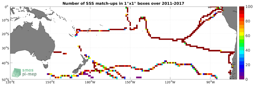
Figure 4: Number of SSS match-ups between TSG (GOSUD-Sailing-ship) SSS and the SMOS and SMAP SSS L4 OI v1 - 7 Days (LOPS) SSS product for the South Pacific Ocean Pi-MEP region over 1^\circ \times 1^\circ boxes and for the full satellite product period.
