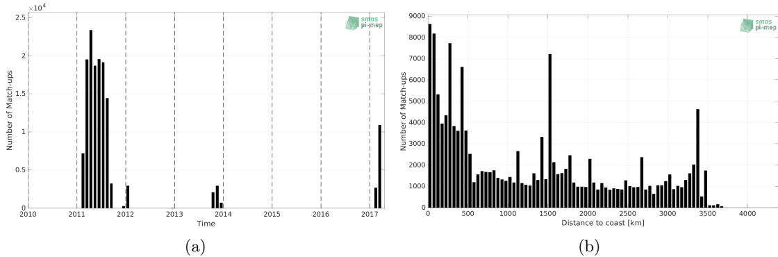
Figure 1: Number of match-ups between TSG (GOSUD-Sailing-ship) and SMOS and SMAP SSS L4 OI v1 - 7 Days (LOPS) SSS as a function of time (a) and as function of the distance to coast (b) over the South Pacific Ocean Pi-MEP region and for the full satellite product period.
