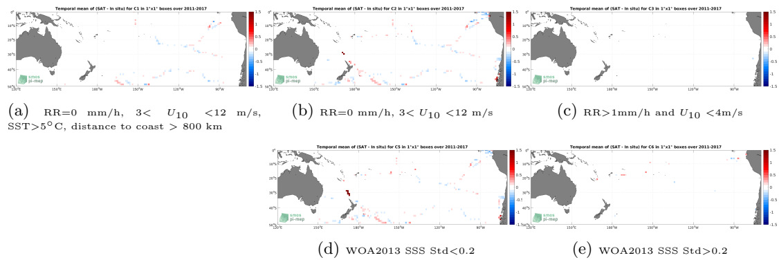
Figure 12: Temporal mean gridded over spatial boxes of size 1^\circ \times 1^\circ of \Delta SSS (SMOS and SMAP SSS L4 OI v1 - 7 Days (LOPS) - TSG (GOSUD-Sailing-ship)) for 5 different subdatasets corresponding to:RR=0 mm/h, 3 < U_{10} < 12 m/s, SST >5^\circ C, distance to coast > 800 km (a), RR=0 mm/h, 3 < U_{10} < 12 m/s (b), RR >1 mm/h and U_{10} < 4 m/s (c), WOA2013 SSS Std <0.2 (d), WOA2013 SSS Std >0.2 (e).
