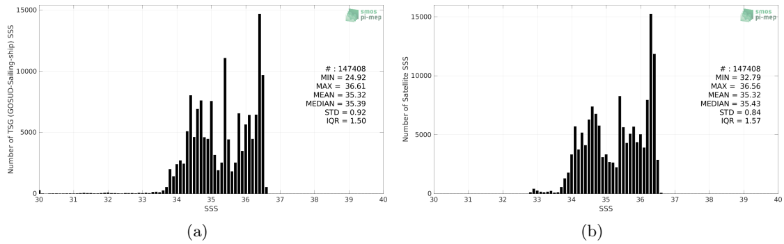
Figure 2: Histograms of SSS from TSG (GOSUD-Sailing-ship) (a) and SMOS and SMAP SSS L4 OI v1 - 7 Days (LOPS) (b) considering all match-up pairs per bins of 0.1 over the South Pacific Ocean Pi-MEP region and for the full satellite product period.
