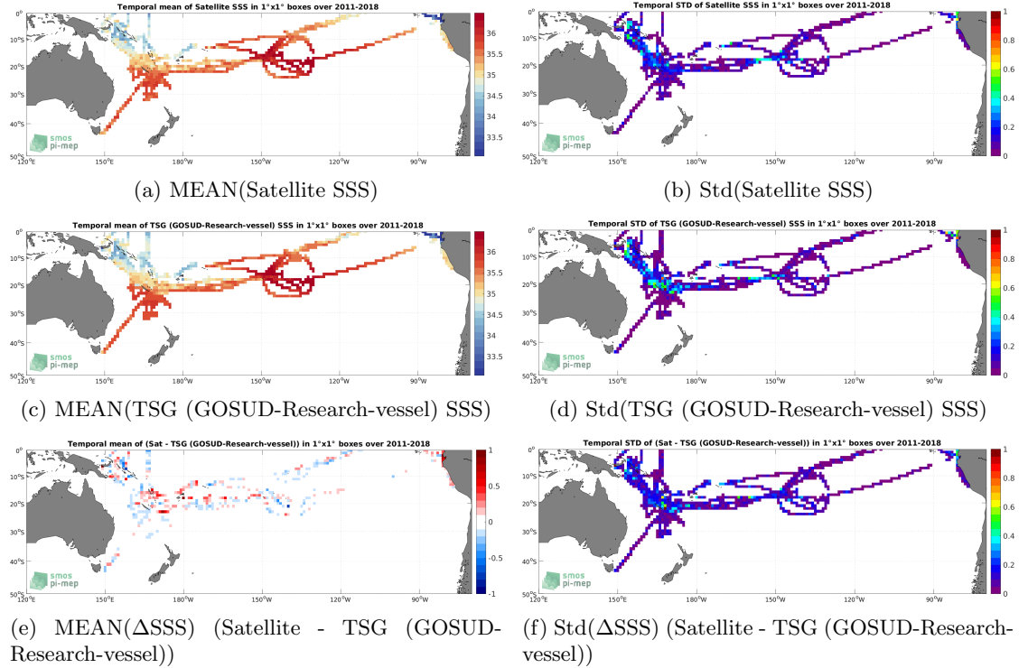
Figure 6: Temporal mean (left) and Std (right) of SSS from SMOS and SMAP SSS L4 OI v1 - 7 Days (LOPS) (top), TSG (GOSUD-Research-vessel) (middle), and of \Delta SSS (Satellite - TSG (GOSUD-Research-vessel)). Only match-up pairs are used to generate these maps.
