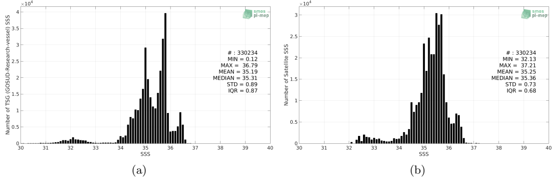
Figure 2: Histograms of SSS from TSG (GOSUD-Research-vessel) (a) and SMOS and SMAP SSS L4 OI v1 - 7 Days (LOPS) (b) considering all match-up pairs per bins of 0.1 over the South Pacific Ocean Pi-MEP region and for the full satellite product period.
