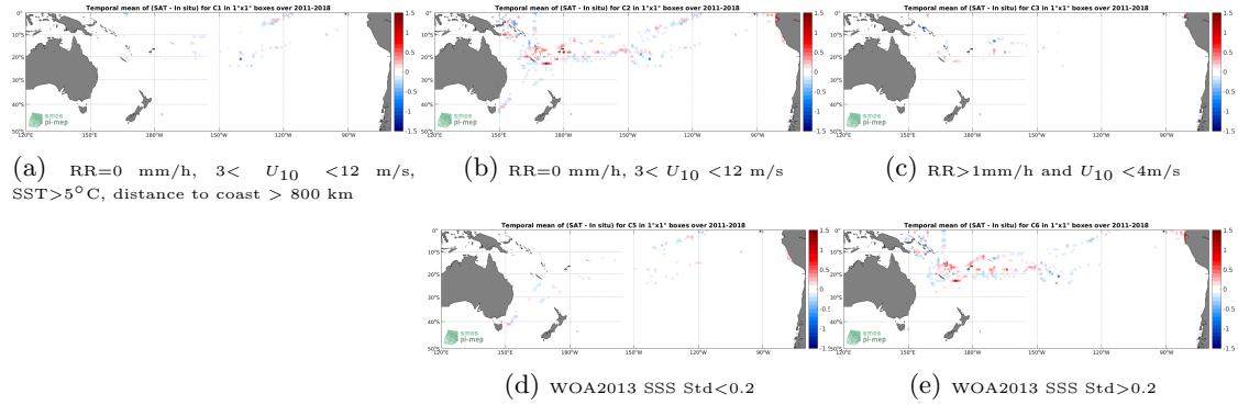
Figure 12: Temporal mean gridded over spatial boxes of size 1^\circ \times 1^\circ of \Delta SSS (SMOS and SMAP SSS L4 OI v1 - 7 Days (LOPS) - TSG (GOSUD-Research-vessel)) for 5 different subdatasets corresponding to: RR=0 mm/h, 3 < U_{10} < 12 m/s, SST >5^\circ\text{C} , distance to coast > 800 km (a), RR=0 mm/h, 3 < U_{10} < 12 m/s (b), RR>1\text{mm/h} and U_{10} < 4\text{m/s} (c), WOA2013 SSS Std <0.2 (d), WOA2013 SSS Std >0.2 (e).
