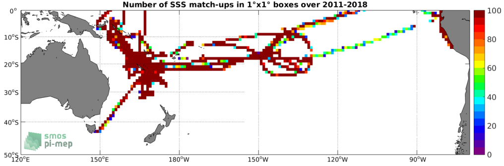
Figure 4: Number of SSS match-ups between TSG (GOSUD-Research-vessel) SSS and the SMOS and SMAP SSS L4 OI v1 - 7 Days (LOPS) SSS product for the South Pacific Ocean Pi-MEP region over 1^\circ \times 1^\circ boxes and for the full satellite product period.
