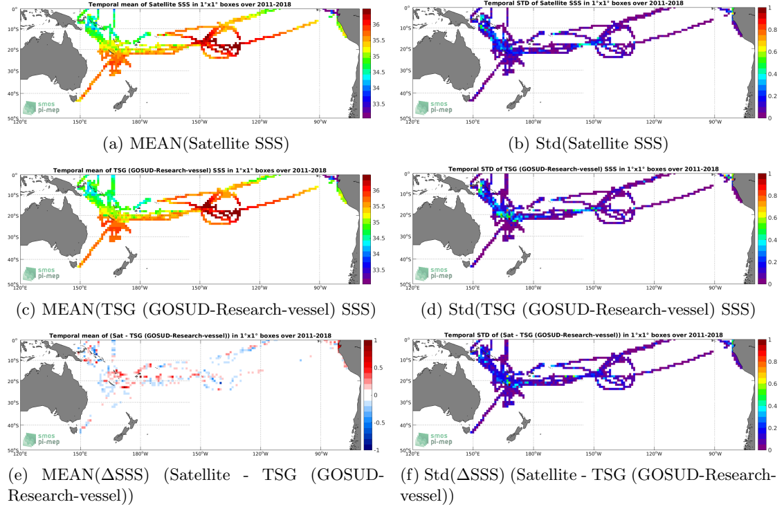
Figure 6: Temporal mean (left) and Std (right) of SSS from SMOS and SMAP SSS L4 OI v1 - 7 Days (LOPS) (top), TSG (GOSUD-Research-vessel) (middle), and of \Delta SSS (Satellite - TSG (GOSUD-Research-vessel)). Only match-up pairs are used to generate these maps.
