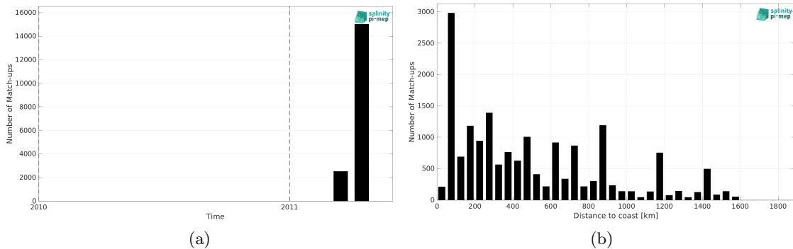
Figure 1: Number of match-ups between TSG (CSIC-UTM) and SMOS and SMAP SSS L4 OI v1 - 7 Days (LOPS) SSS as a function of time (a) and as function of the distance to coast (b) over the South Pacific Ocean Pi-MEP region and for the full satellite product period.
