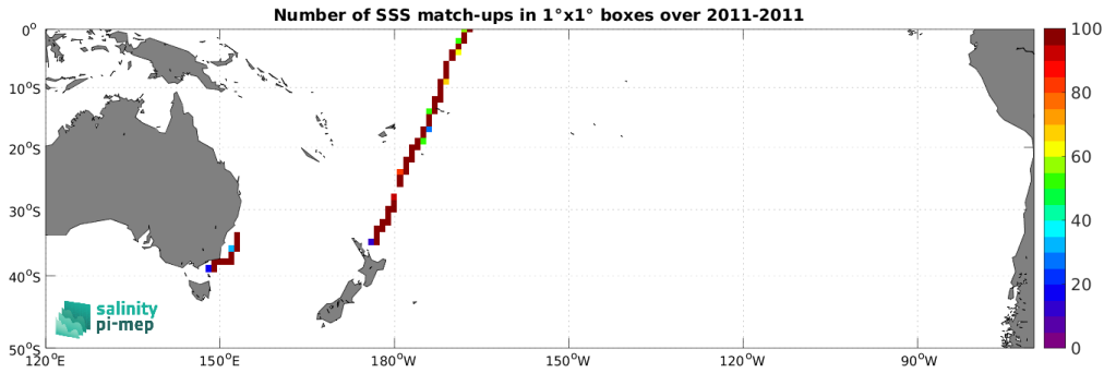
Figure 4: Number of SSS match-ups between TSG (CSIC-UTM) SSS and the SMOS and SMAP SSS L4 OI v1 - 7 Days (LOPS) SSS product for the South Pacific Ocean Pi-MEP region over 1^\circ \times 1^\circ boxes and for the full satellite product period.
