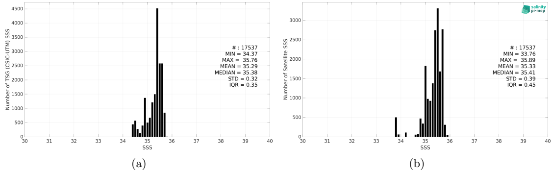
Figure 2: Histograms of SSS from TSG (CSIC-UTM) (a) and SMOS and SMAP SSS L4 OI v1 - 7 Days (LOPS) (b) considering all match-up pairs per bins of 0.1 over the South Pacific Ocean Pi-MEP region and for the full satellite product period.
