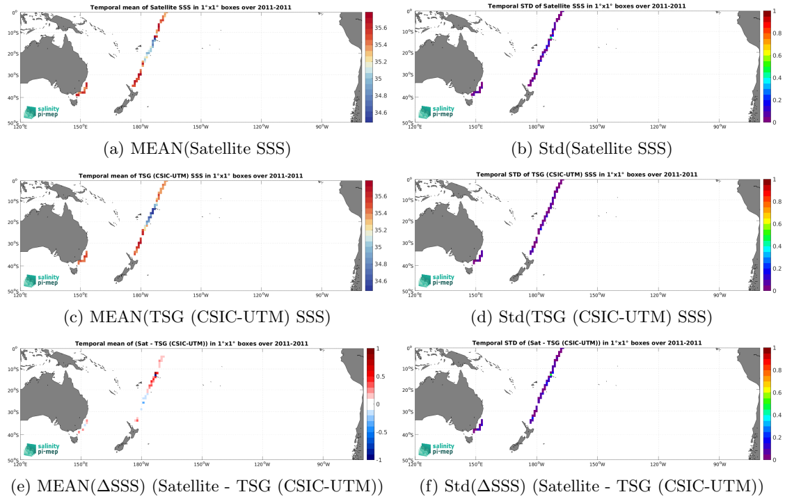
Figure 6: Temporal mean (left) and Std (right) of SSS from SMOS and SMAP SSS L4 OI v1 - 7 Days (LOPS) (top), TSG (CSIC-UTM) (middle), and of \Delta SSS (Satellite - TSG (CSIC-UTM)). Only match-up pairs are used to generate these maps.
