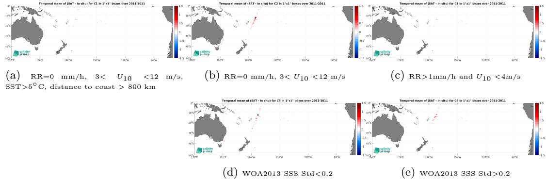
Figure 12: Temporal mean gridded over spatial boxes of size 1^{\circ}\times 1^{\circ} of \Delta\text{SSS} (SMOS and SMAP SSS L4 OI v1 - 7 Days (LOPS) - TSG (CSIC-UTM)) for 5 different subdatasets corresponding to:RR=0 mm/h, 3 < U_{10} < 12 m/s, SST > 5^{\circ}\text{C} , distance to coast > 800 km (a), RR=0 mm/h, 3 < U_{10} < 12 m/s (b), RR > 1 mm/h and U_{10} < 4 m/s (c), WOA2013 SSS Std < 0.2 (d), WOA2013 SSS Std > 0.2 (e).
