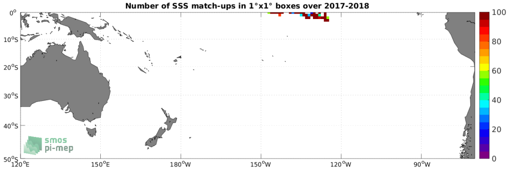
Figure 4: Number of SSS match-ups between Saildrone SSS and the SMOS and SMAP SSS L4 OI v1 - 7 Days (LOPS) SSS product for the South Pacific Ocean Pi-MEP region over 1^\circ \times 1^\circ boxes and for the full satellite product period.
