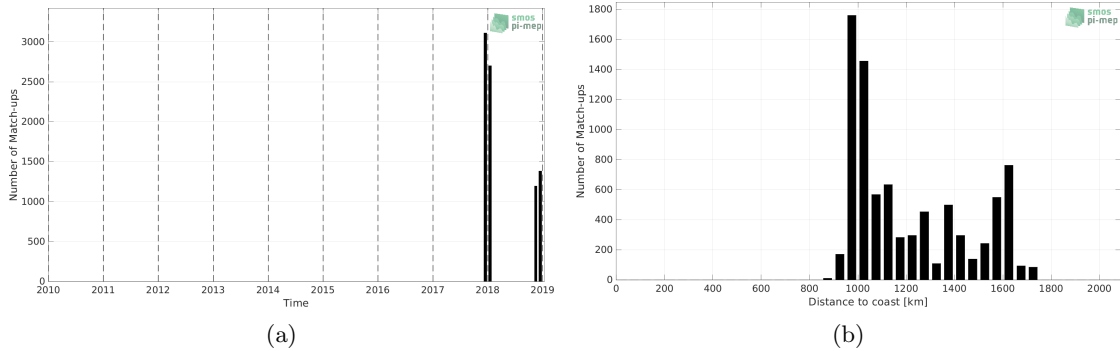
Figure 1: Number of match-ups between Saildrone and SMOS and SMAP SSS L4 OI v1 - 7 Days (LOPS) SSS as a function of time (a) and as function of the distance to coast (b) over the South Pacific Ocean Pi-MEP region and for the full satellite product period.
