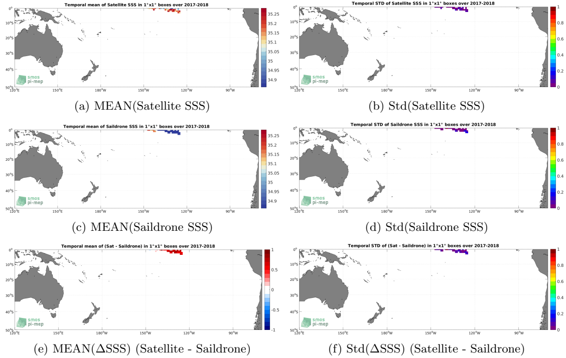
Figure 6: Temporal mean (left) and Std (right) of SSS from SMOS and SMAP SSS L4 OI v1 - 7 Days (LOPS) (top), Saildrone (middle), and of \Delta SSS (Satellite - Saildrone). Only match-up pairs are used to generate these maps.
