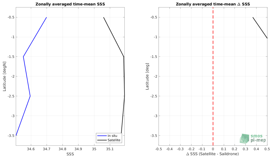
Figure 8: Left panel: Zonal mean SSS from SMOS and SMAP SSS L4 OI v1 - 7 Days (LOPS) satellite product (black) and from Sairdrone (blue). Right panel: Zonal mean of \Delta SSS (Satellite - Sairdrone) for all the collected Pi-MEP match-up pairs estimated over the full satellite product period.
