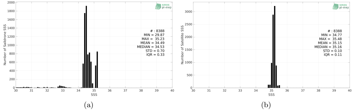
Figure 2: Histograms of SSS from Saildrone (a) and SMOS and SMAP SSS L4 OI v1 - 7 Days (LOPS) (b) considering all match-up pairs per bins of 0.1 over the South Pacific Ocean Pi-MEP region and for the full satellite product period.
