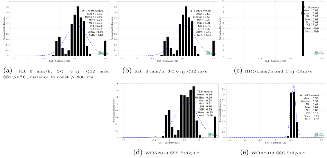
Figure 13: Normalized histogram of \Delta SSS (SMOS and SMAP SSS L4 OI v1 - 7 Days (LOPS) - Saildrone) for 5 different subdatasets corresponding to: RR=0 mm/h, 3 < U_{10} < 12 m/s, SST > 5°C, distance to coast > 800 km (a), RR=0 mm/h, 3 < U_{10} < 12 m/s (b), RR > 1mm/h and U_{10} < 4 m/s (c), WOA2013 SSS Std < 0.2 (d), WOA2013 SSS Std > 0.2 (e).
