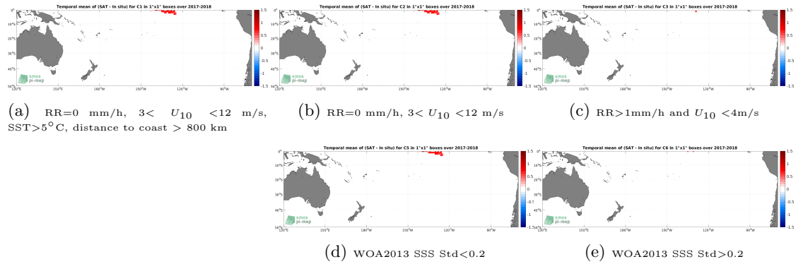
Figure 12: Temporal mean gridded over spatial boxes of size 1^\circ \times 1^\circ of \Delta SSS (SMOS and SMAP SSS L4 OI v1 - 7 Days (LOPS) - Sairdrone) for 5 different subdatasets corresponding to:RR=0 mm/h, 3 < U_{10} < 12 m/s, SST >5^\circ\text{C} , distance to coast > 800 km (a), RR=0 mm/h, 3 < U_{10} < 12 m/s (b), RR >1 mm/h and U_{10} < 4 m/s (c), WOA2013 SSS Std <0.2 (d), WOA2013 SSS Std >0.2 (e).
