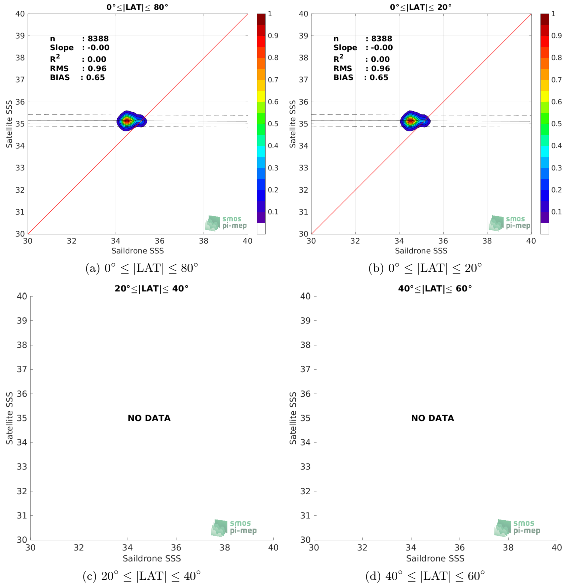
Figure 9: Contour maps of the concentration of SMOS and SMAP SSS L4 OI v1 - 7 Days (LOPS) SSS (y-axis) versus Sailldrone SSS (x-axis) at match-up pairs for different latitude bands. For each plot, the red line shows x=y . The black thin and dashed lines indicate a linear fit through the data cloud and the \pm 95\% confidence levels, respectively. The number match-up pairs n , the slope and R^2 coefficient of the linear fit, the root mean square (RMS) and the mean bias between satellite and in situ data are indicated for each latitude band in each plots.
