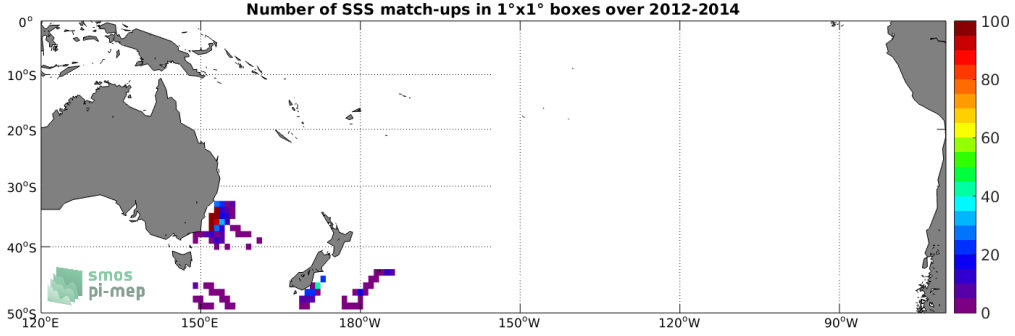
Figure 4: Number of SSS match-ups between Marine mammals SSS and the SMOS and SMAP SSS L4 OI v1 - 7 Days (LOPS) SSS product for the South Pacific Ocean Pi-MEP region over 1^\circ \times 1^\circ boxes and for the full satellite product period.
