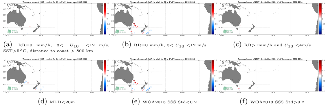
Figure 12: Temporal mean gridded over spatial boxes of size 1^\circ \times 1^\circ of \Delta SSS (SMOS and SMAP SSS L4 OI v1 - 7 Days (LOPS) - Marine mammals) for 6 different subdatasets corresponding to: RR=0 mm/h, 3 < U_{10} < 12 m/s, SST > 5^\circ C , distance to coast > 800 km (a), RR=0 mm/h, 3 < U_{10} < 12 m/s (b), RR > 1 mm/h and U_{10} < 4 m/s (c), MLD < 20 m (d), WOA2013 SSS Std < 0.2 (e), WOA2013 SSS Std > 0.2 (f).
