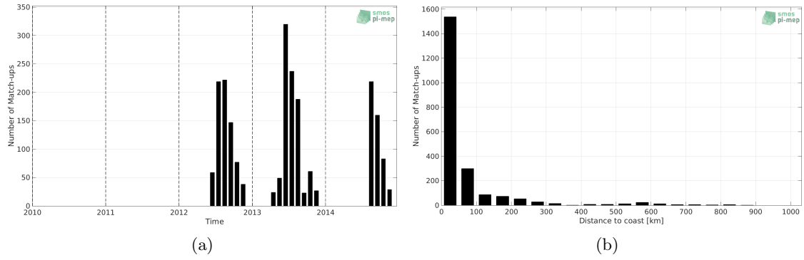
Figure 1: Number of match-ups between Marine mammals and SMOS and SMAP SSS L4 OI v1 - 7 Days (LOPS) SSS as a function of time (a) and as function of the distance to coast (b) over the South Pacific Ocean Pi-MEP region and for the full satellite product period.
