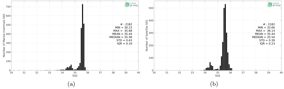
Figure 2: Histograms of SSS from Marine mammals (a) and SMOS and SMAP SSS L4 OI v1 - 7 Days (LOPS) (b) considering all match-up pairs per bins of 0.1 over the South Pacific Ocean Pi-MEP region and for the full satellite product period.
