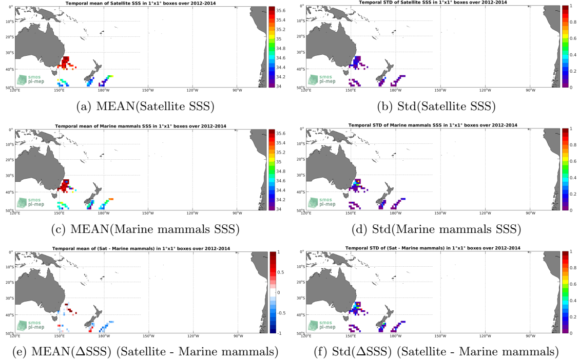
Figure 6: Temporal mean (left) and Std (right) of SSS from SMOS and SMAP SSS L4 OI v1 - 7 Days (LOPS) (top), Marine mammals (middle), and of \Delta SSS (Satellite - Marine mammals). Only match-up pairs are used to generate these maps.
