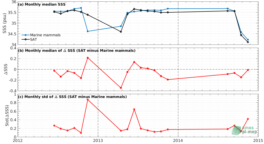
Figure 7: Time series of the monthly median SSS (top), median of \Delta\text{SSS} (Satellite - Marine mammals) and Std of \Delta\text{SSS} (Satellite - Marine mammals) over the South Pacific Ocean Pi-MEP region considering all match-ups collected by the Pi-MEP.
