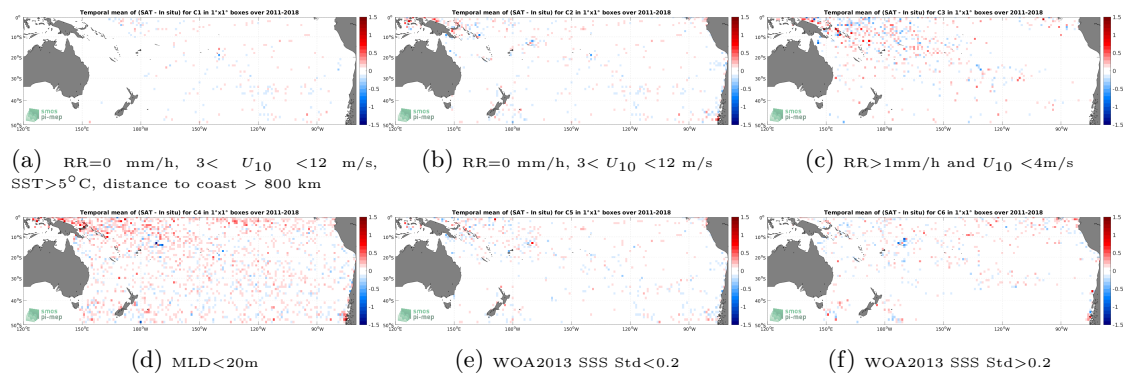
Figure 12: Temporal mean gridded over spatial boxes of size 1^\circ \times 1^\circ of \Delta SSS (SMOS and SMAP SSS L4 OI v1 - 7 Days (LOPS) - Argo) for 6 different subdatasets corresponding to:RR=0 mm/h, 3 < U_{10} < 12 m/s, SST >5^\circ C, distance to coast > 800 km (a), RR=0 mm/h, 3 < U_{10} < 12 m/s (b), RR >1 mm/h and U_{10} < 4 m/s (c),MLD <20 m (d),WOA2013 SSS Std <0.2 (e),WOA2013 SSS Std >0.2 (f).
