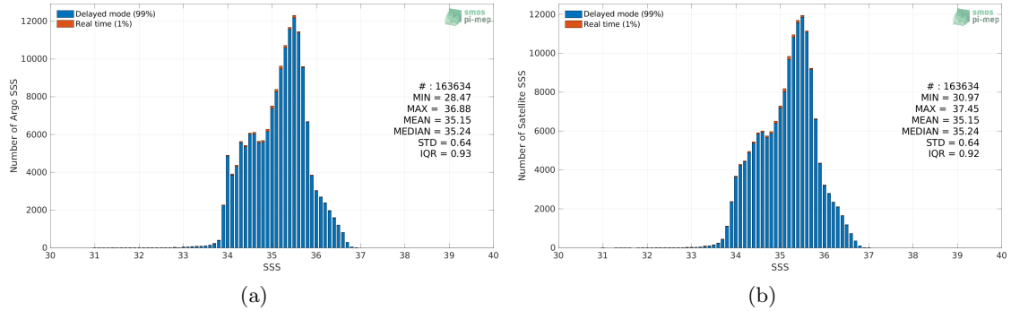
Figure 2: Histograms of SSS from Argo (a) and SMOS and SMAP SSS L4 OI v1 - 7 Days (LOPS) (b) considering all match-up pairs per bins of 0.1 over the South Pacific Ocean Pi-MEP region and for the full satellite product period.
