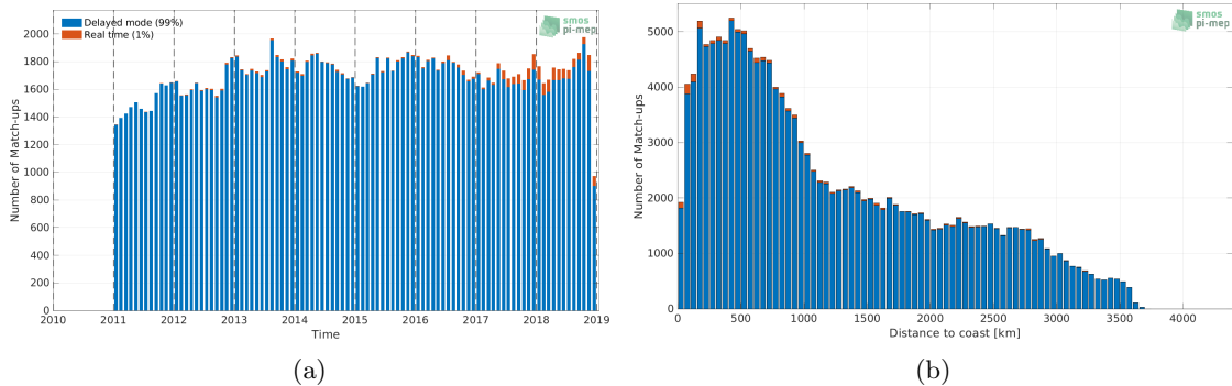
Figure 1: Number of match-ups between Argo and SMOS and SMAP SSS L4 OI v1 - 7 Days (LOPS) SSS as a function of time (a) and as function of the distance to coast (b) over the South Pacific Ocean Pi-MEP region and for the full satellite product period.
