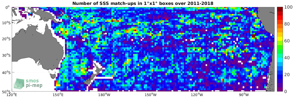
Figure 4: Number of SSS match-ups between Argo SSS and the SMOS and SMAP SSS L4 OI v1 - 7 Days (LOPS) SSS product for the South Pacific Ocean Pi-MEP region over 1^\circ \times 1^\circ boxes and for the full satellite product period.
