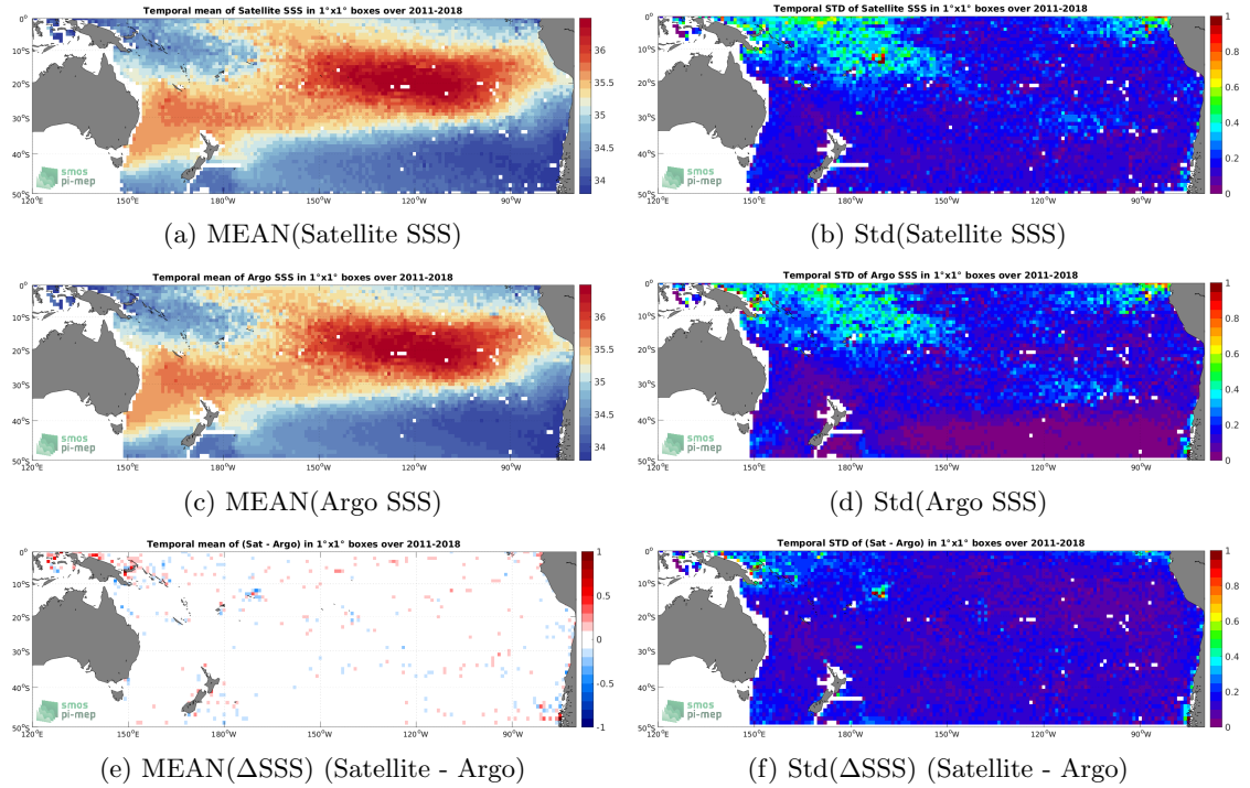
Figure 6: Temporal mean (left) and Std (right) of SSS from SMOS and SMAP SSS L4 OI v1 - 7 Days (LOPS) (top), Argo (middle), and of \Delta SSS (Satellite - Argo). Only match-up pairs are used to generate these maps.
