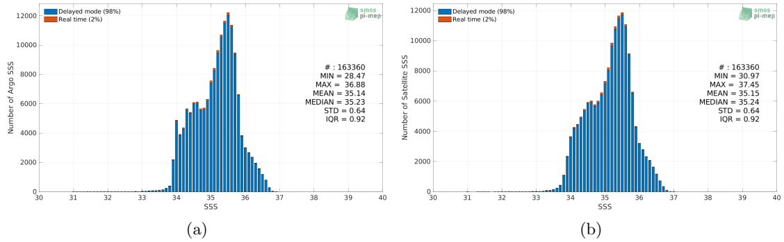
Figure 2: Histograms of SSS from Argo (a) and SMOS and SMAP SSS L4 OI v1 - 7 Days (LOPS) (b) considering all match-up pairs per bins of 0.1 over the South Pacific Ocean Pi-MEP region and for the full satellite product period.
