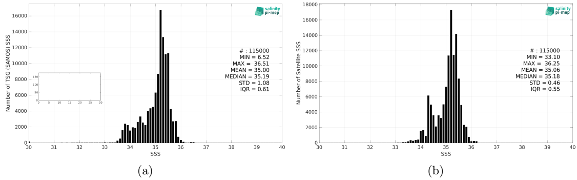
Figure 2: Histograms of SSS from TSG (SAMOS) (a) and SMOS SSS L4 v1 - Weekly (CMEMS-CNR) (b) considering all match-up pairs per bins of 0.1 over the South Pacific Ocean Pi-MEP region and for the full satellite product period.
