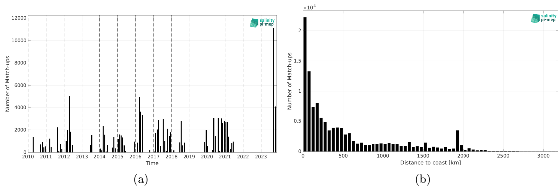
Figure 1: Number of match-ups between TSG (SAMOS) and SMOS SSS L4 v1 - Weekly (CMEMS-CNR) SSS as a function of time (a) and as function of the distance to coast (b) over the South Pacific Ocean Pi-MEP region and for the full satellite product period.
