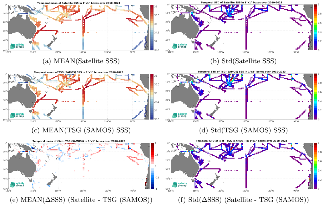
Figure 6: Temporal mean (left) and Std (right) of SSS from SMOS SSS L4 v1 - Weekly (CMEMS-CNR) (top), TSG (SAMOS) (middle), and of \Delta SSS (Satellite - TSG (SAMOS)). Only match-up pairs are used to generate these maps.
