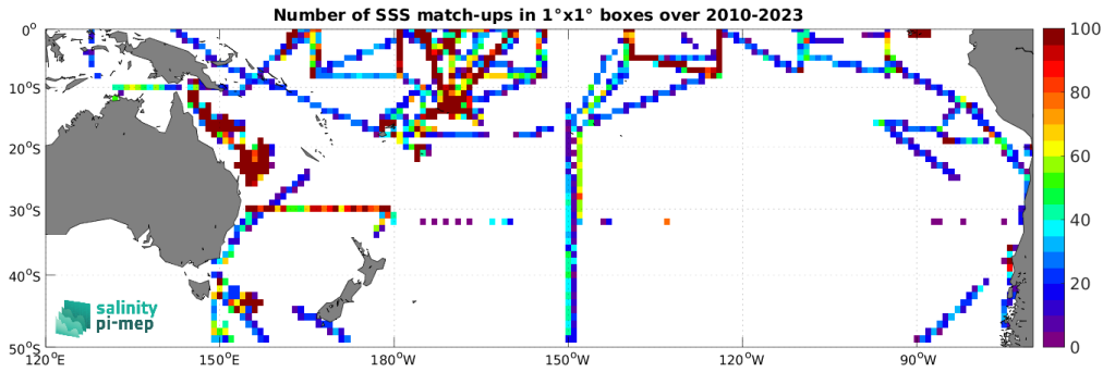
Figure 4: Number of SSS match-ups between TSG (SAMOS) SSS and the SMOS SSS L4 v1 - Weekly (CMEMS-CNR) SSS product for the South Pacific Ocean Pi-MEP region over 1^\circ \times 1^\circ boxes and for the full satellite product period.
