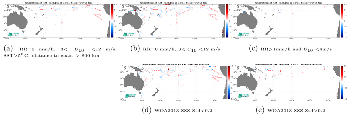
Figure 12: Temporal mean gridded over spatial boxes of size 1^\circ \times 1^\circ of \Delta SSS (SMOS SSS L4 v1 - Weekly (CMEMS-CNR) - TSG (SAMOS)) for 5 different subdatasets corresponding to:RR=0 mm/h, 3 < U_{10} < 12 m/s, SST >5^\circ\text{C} , distance to coast > 800 km (a), RR=0 mm/h, 3 < U_{10} < 12 m/s (b), RR >1 mm/h and U_{10} < 4 m/s (c), WOA2013 SSS Std <0.2 (d), WOA2013 SSS Std >0.2 (e).
