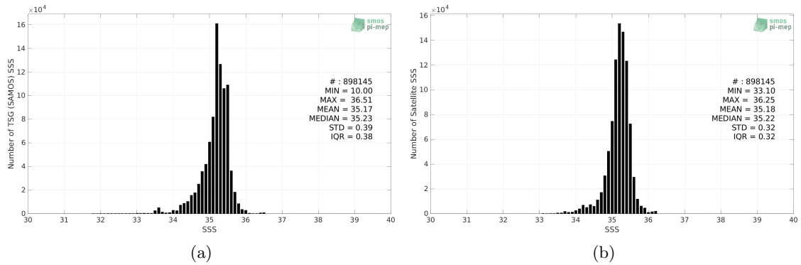
Figure 2: Histograms of SSS from TSG (SAMOS) (a) and SMOS SSS L4 v1 - Weekly (CMEMS-CNR) (b) considering all match-up pairs per bins of 0.1 over the South Pacific Ocean Pi-MEP region and for the full satellite product period.
