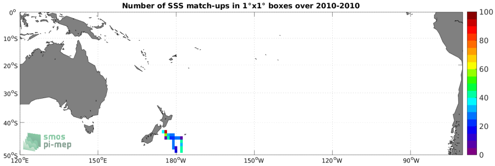
Figure 4: Number of SSS match-ups between TSG (Polarstern) SSS and the SMOS SSS L4 v1 - Weekly (CMEMS-CNR) SSS product for the South Pacific Ocean Pi-MEP region over 1^\circ \times 1^\circ boxes and for the full satellite product period.
