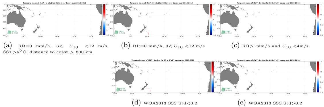
Figure 12: Temporal mean gridded over spatial boxes of size 1^{\circ}\times 1^{\circ} of \Delta\text{SSS} (SMOS SSS L4 v1 - Weekly (CMEMS-CNR) - TSG (Polarstern)) for 5 different subdatasets corresponding to:RR=0 mm/h, 3 < U_{10} < 12 m/s, SST > 5^{\circ}\text{C} , distance to coast > 800 km (a), RR=0 mm/h, 3 < U_{10} < 12 m/s (b), RR > 1 mm/h and U_{10} < 4 m/s (c), WOA2013 SSS Std < 0.2 (d), WOA2013 SSS Std > 0.2 (e).
