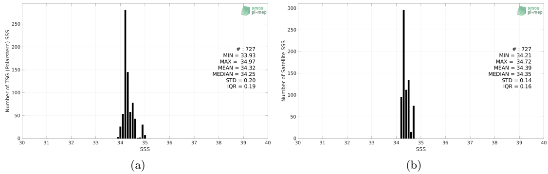
Figure 2: Histograms of SSS from TSG (Polarstern) (a) and SMOS SSS L4 v1 - Weekly (CMEMS-CNR) (b) considering all match-up pairs per bins of 0.1 over the South Pacific Ocean Pi-MEP region and for the full satellite product period.
