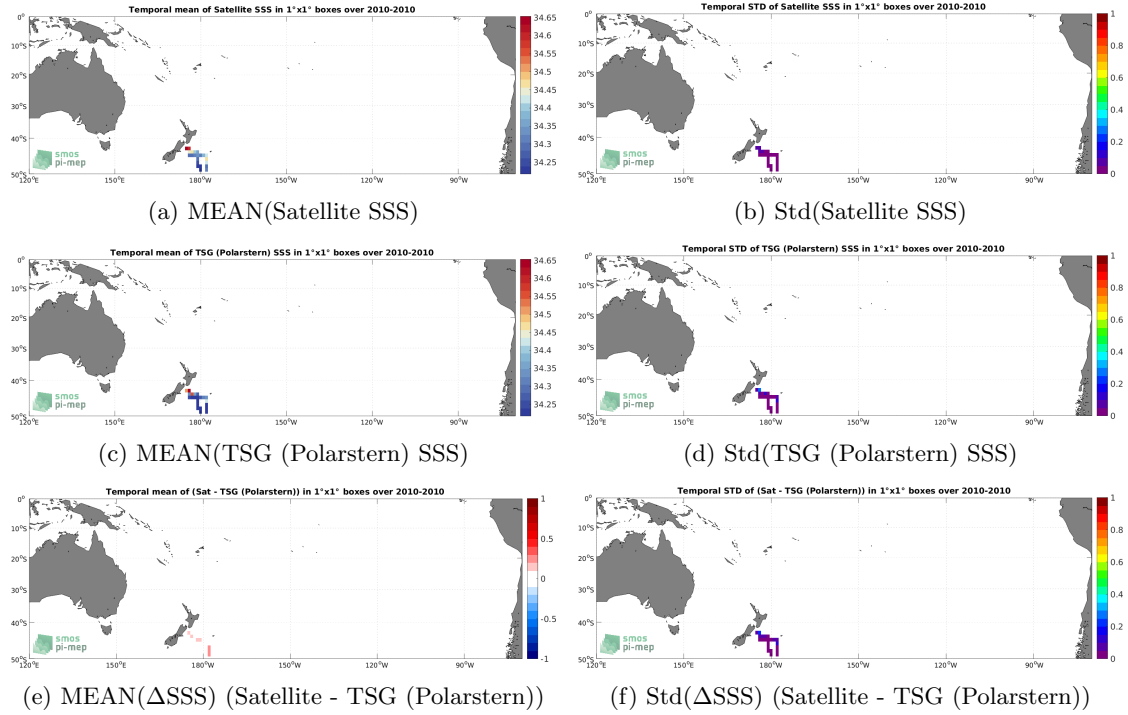
Figure 6: Temporal mean (left) and Std (right) of SSS from SMOS SSS L4 v1 - Weekly (CMEMS-CNR) (top), TSG (Polarstern) (middle), and of \Delta SSS (Satellite - TSG (Polarstern)). Only match-up pairs are used to generate these maps.
