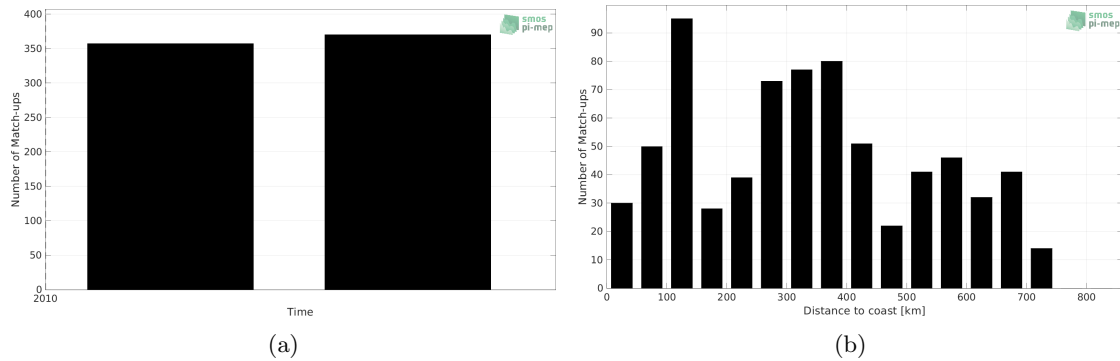
Figure 1: Number of match-ups between TSG (Polarstern) and SMOS SSS L4 v1 - Weekly (CMEMS-CNR) SSS as a function of time (a) and as function of the distance to coast (b) over the South Pacific Ocean Pi-MEP region and for the full satellite product period.
