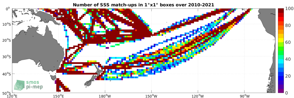
Figure 3: Number of SSS match-ups between TSG (LEGOS-DM) SSS and the SMOS SSS L4 v1 - Weekly (CMEMS-CNR) SSS product for the South Pacific Ocean Pi-MEP region over 1^\circ \times 1^\circ boxes and for the full satellite product period.
