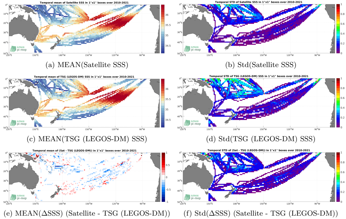
Figure 5: Temporal mean (left) and Std (right) of SSS from SMOS SSS L4 v1 - Weekly (CMEMS-CNR) (top), TSG (LEGOS-DM) (middle), and of \Delta SSS (Satellite - TSG (LEGOS-DM)). Only match-up pairs are used to generate these maps.
