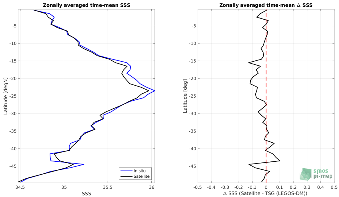
Figure 7: Left panel: Zonal mean SSS from SMOS SSS L4 v1 - Weekly (CMEMS-CNR) satellite product (black) and from TSG (LEGOS-DM) (blue). Right panel: Zonal mean of \Delta SSS (Satellite - TSG (LEGOS-DM)) for all the collected Pi-MEP match-up pairs estimated over the full satellite product period.
