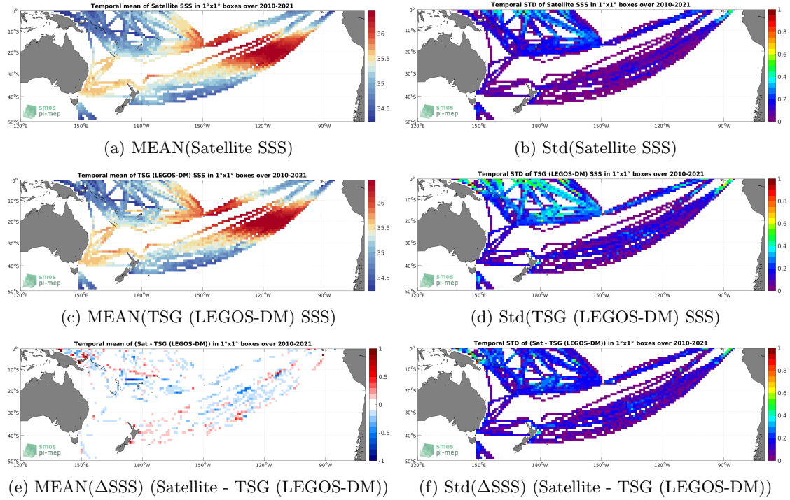
Figure 6: Temporal mean (left) and Std (right) of SSS from SMOS SSS L4 v1 - Weekly (CMEMS-CNR) (top), TSG (LEGOS-DM) (middle), and of \Delta SSS (Satellite - TSG (LEGOS-DM)). Only match-up pairs are used to generate these maps.
