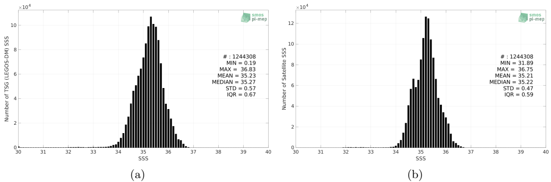
Figure 2: Histograms of SSS from TSG (LEGOS-DM) (a) and SMOS SSS L4 v1 - Weekly (CMEMS-CNR) (b) considering all match-up pairs per bins of 0.1 over the South Pacific Ocean Pi-MEP region and for the full satellite product period.
