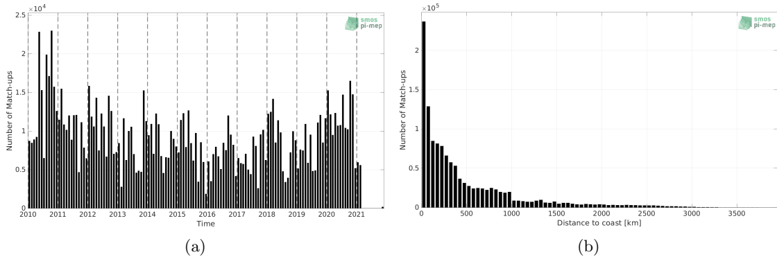
Figure 1: Number of match-ups between TSG (LEGOS-DM) and SMOS SSS L4 v1 - Weekly (CMEMS-CNR) SSS as a function of time (a) and as function of the distance to coast (b) over the South Pacific Ocean Pi-MEP region and for the full satellite product period.
