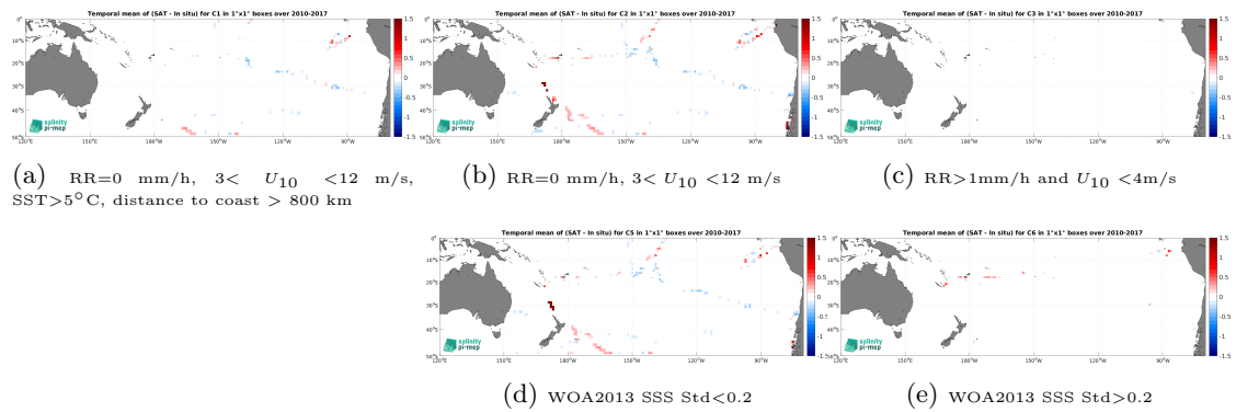
Figure 12: Temporal mean gridded over spatial boxes of size 1^\circ \times 1^\circ of \Delta\text{SSS} (SMOS SSS L4 v1 - Weekly (CMEMS-CNR) - TSG (GOSUD-Sailing-ship)) for 5 different subdatasets corresponding to:RR=0 mm/h, 3 < U_{10} < 12 m/s, SST >5^\circ\text{C} , distance to coast > 800 km (a), RR=0 mm/h, 3 < U_{10} < 12 m/s (b), RR >1 mm/h and U_{10} < 4 m/s (c), WOA2013 SSS Std <0.2 (d), WOA2013 SSS Std >0.2 (e).
