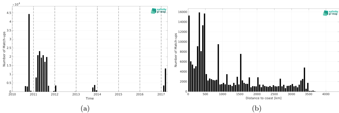
Figure 1: Number of match-ups between TSG (GOSUD-Sailing-ship) and SMOS SSS L4 v1 - Weekly (CMEMS-CNR) SSS as a function of time (a) and as function of the distance to coast (b) over the South Pacific Ocean Pi-MEP region and for the full satellite product period.
