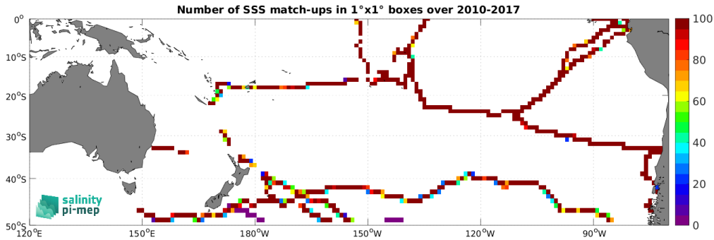
Figure 4: Number of SSS match-ups between TSG (GOSUD-Sailing-ship) SSS and the SMOS SSS L4 v1 - Weekly (CMEMS-CNR) SSS product for the South Pacific Ocean Pi-MEP region over 1^\circ \times 1^\circ boxes and for the full satellite product period.
