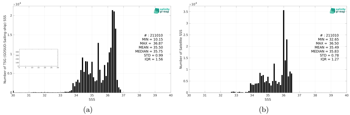
Figure 2: Histograms of SSS from TSG (GOSUD-Sailing-ship) (a) and SMOS SSS L4 v1 - Weekly (CMEMS-CNR) (b) considering all match-up pairs per bins of 0.1 over the South Pacific Ocean Pi-MEP region and for the full satellite product period.
