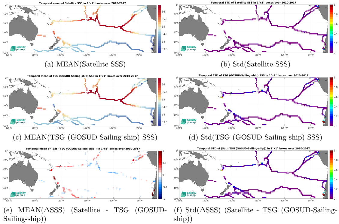
Figure 6: Temporal mean (left) and Std (right) of SSS from SMOS SSS L4 v1 - Weekly (CMEMS-CNR) (top), TSG (GOSUD-Sailing-ship) (middle), and of \Delta SSS (Satellite - TSG (GOSUD-Sailing-ship)). Only match-up pairs are used to generate these maps.
