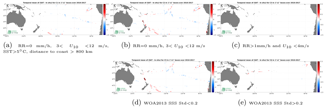
Figure 12: Temporal mean gridded over spatial boxes of size 1^\circ \times 1^\circ of \Delta SSS (SMOS SSS L4 v1 - Weekly (CMEMS-CNR) - TSG (GOSUD-Sailing-ship)) for 5 different subdatasets corresponding to:RR=0 mm/h, 3 < U_{10} < 12 m/s, SST >5^\circ C, distance to coast > 800 km (a), RR=0 mm/h, 3 < U_{10} < 12 m/s (b), RR >1 mm/h and U_{10} < 4 m/s (c), WOA2013 SSS Std <0.2 (d), WOA2013 SSS Std >0.2 (e).
