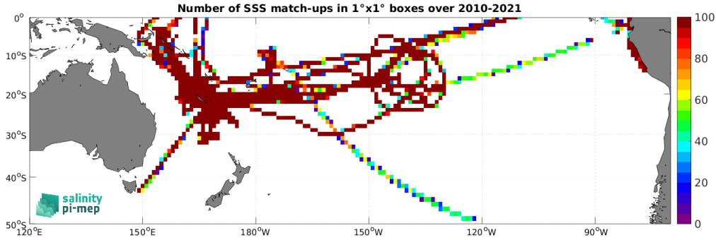
Figure 4: Number of SSS match-ups between TSG (GOSUD-Research-vessel) SSS and the SMOS SSS L4 v1 - Weekly (CMEMS-CNR) SSS product for the South Pacific Ocean Pi-MEP region over 1^\circ \times 1^\circ boxes and for the full satellite product period.
