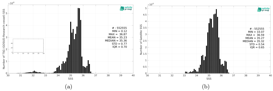
Figure 2: Histograms of SSS from TSG (GOSUD-Research-vessel) (a) and SMOS SSS L4 v1 - Weekly (CMEMS-CNR) (b) considering all match-up pairs per bins of 0.1 over the South Pacific Ocean Pi-MEP region and for the full satellite product period.
