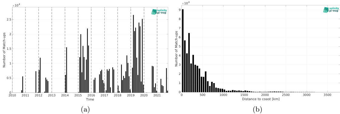
Figure 1: Number of match-ups between TSG (GOSUD-Research-vessel) and SMOS SSS L4 v1 - Weekly (CMEMS-CNR) SSS as a function of time (a) and as function of the distance to coast (b) over the South Pacific Ocean Pi-MEP region and for the full satellite product period.
