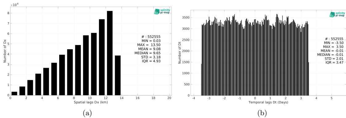
Figure 5: Histograms of the spatial (a) and temporal (b) lags between the location/time of the TSG (GOSUD-Research-vessel) measurement and the date of the corresponding SMOS SSS L4 v1 - Weekly (CMEMS-CNR) SSS pixel.
