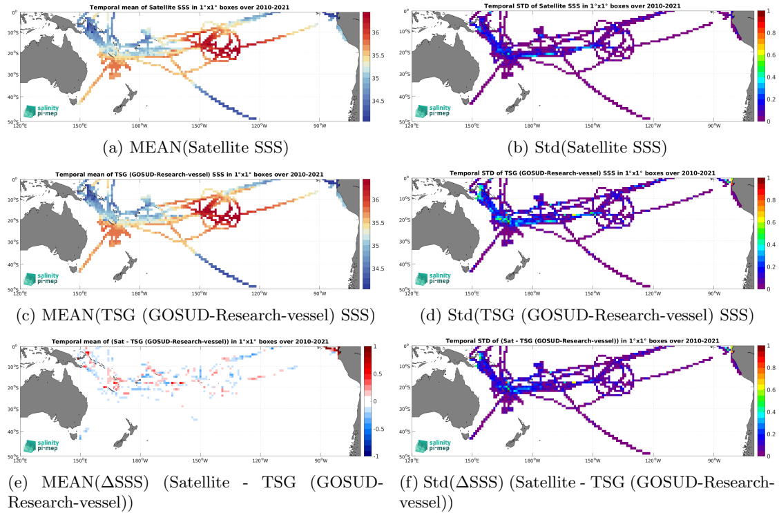
Figure 6: Temporal mean (left) and Std (right) of SSS from SMOS SSS L4 v1 - Weekly (CMEMS-CNR) (top), TSG (GOSUD-Research-vessel) (middle), and of \Delta SSS (Satellite - TSG (GOSUD-Research-vessel)). Only match-up pairs are used to generate these maps.
