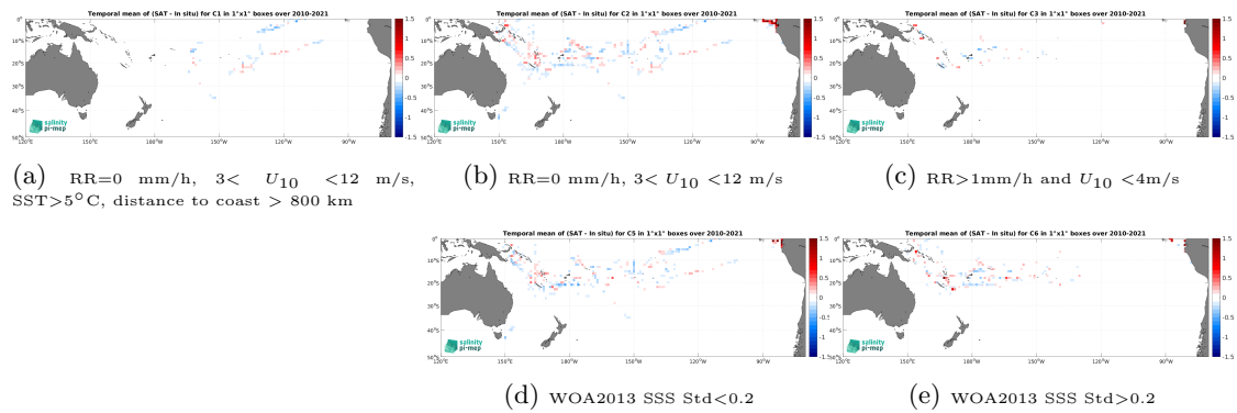
Figure 12: Temporal mean gridded over spatial boxes of size 1^\circ \times 1^\circ of \Delta SSS (SMOS SSS L4 v1 - Weekly (CMEMS-CNR) - TSG (GOSUD-Research-vessel)) for 5 different subdatasets corresponding to:RR=0 mm/h, 3 < U_{10} < 12 m/s, SST>5°C, distance to coast > 800 km (a), RR=0 mm/h, 3 < U_{10} < 12 m/s (b), RR>1mm/h and U_{10} < 4 m/s (c), WOA2013 SSS Std<0.2 (d), WOA2013 SSS Std>0.2 (e).
