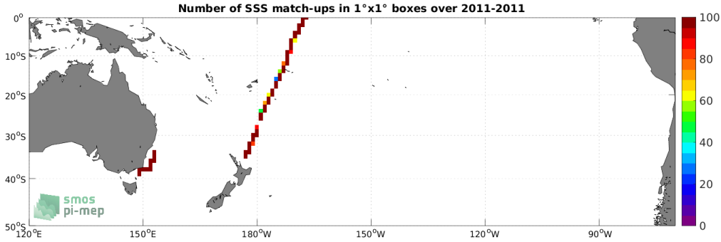
Figure 4: Number of SSS match-ups between TSG (CSIC-UTM) SSS and the SMOS SSS L4 v1 - Weekly (CMEMS-CNR) SSS product for the South Pacific Ocean Pi-MEP region over 1^\circ \times 1^\circ boxes and for the full satellite product period.
