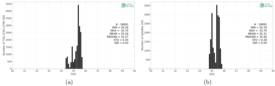
Figure 2: Histograms of SSS from TSG (CSIC-UTM) (a) and SMOS SSS L4 v1 - Weekly (CMEMS-CNR) (b) considering all match-up pairs per bins of 0.1 over the South Pacific Ocean Pi-MEP region and for the full satellite product period.
