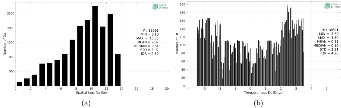
Figure 5: Histograms of the spatial (a) and temporal (b) lags between the location/time of the TSG (CSIC-UTM) measurement and the date of the corresponding SMOS SSS L4 v1 - Weekly (CMEMS-CNR) SSS pixel.
