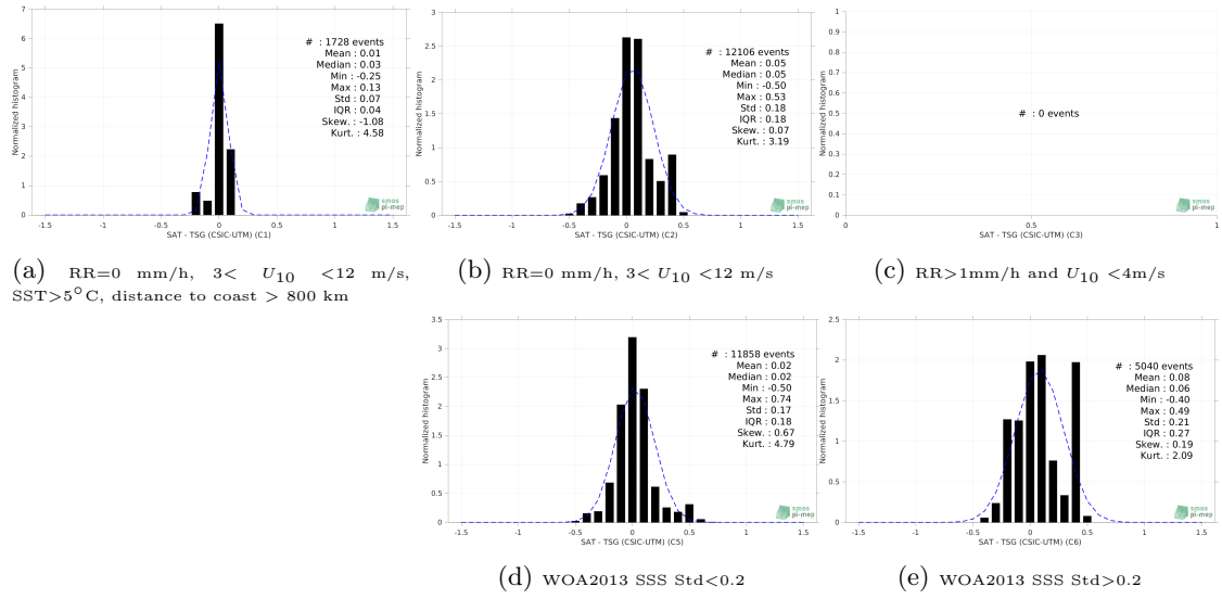
Figure 13: Normalized histogram of \Delta SSS (SMOS SSS L4 v1 - Weekly (CMEMS-CNR) - TSG (CSIC-UTM)) for 5 different subdatasets corresponding to: RR=0 mm/h, 3 < U_{10} < 12 m/s, SST>5°C, distance to coast > 800 km (a), RR=0 mm/h, 3 < U_{10} < 12 m/s (b), RR>1mm/h and U_{10} < 4 m/s (c), WOA2013 SSS Std<0.2 (d), WOA2013 SSS Std>0.2 (e).
