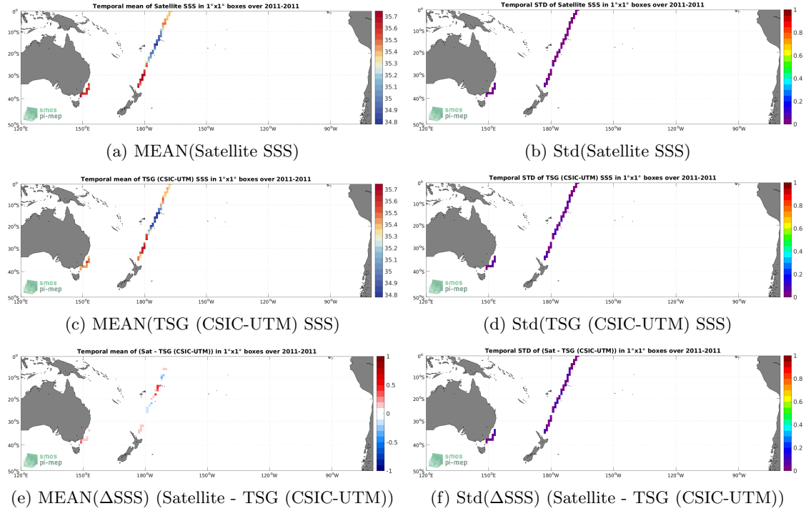
Figure 6: Temporal mean (left) and Std (right) of SSS from SMOS SSS L4 v1 - Weekly (CMEMS-CNR) (top), TSG (CSIC-UTM) (middle), and of \Delta SSS (Satellite - TSG (CSIC-UTM)). Only match-up pairs are used to generate these maps.
