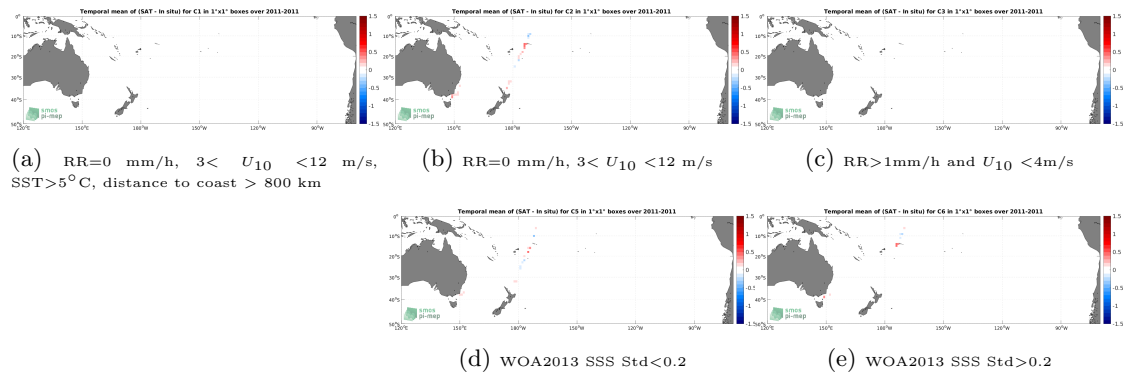
Figure 12: Temporal mean gridded over spatial boxes of size 1^\circ \times 1^\circ of \Delta SSS (SMOS SSS L4 v1 - Weekly (CMEMS-CNR) - TSG (CSIC-UTM)) for 5 different subdatasets corresponding to:RR=0 mm/h, 3 < U_{10} < 12 m/s, SST >5^\circ C, distance to coast > 800 km (a), RR=0 mm/h, 3 < U_{10} < 12 m/s (b), RR >1 mm/h and U_{10} < 4 m/s (c), WOA2013 SSS Std <0.2 (d), WOA2013 SSS Std >0.2 (e).
