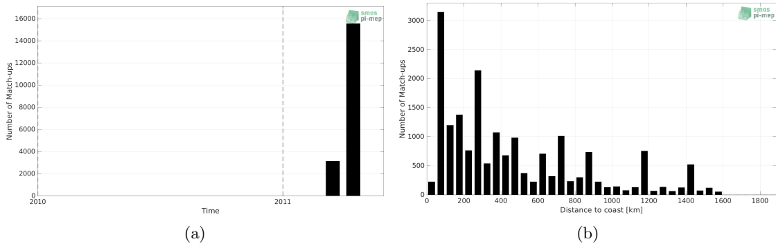
Figure 1: Number of match-ups between TSG (CSIC-UTM) and SMOS SSS L4 v1 - Weekly (CMEMS-CNR) SSS as a function of time (a) and as function of the distance to coast (b) over the South Pacific Ocean Pi-MEP region and for the full satellite product period.
