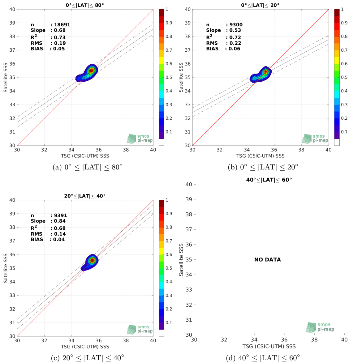
Figure 9: Contour maps of the concentration of SMOS SSS L4 v1 - Weekly (CMEMS-CNR) SSS (y-axis) versus TSG (CSIC-UTM) SSS (x-axis) at match-up pairs for different latitude bands. For each plot, the red line shows x=y . The black thin and dashed lines indicate a linear fit through the data cloud and the \pm 95\% confidence levels, respectively. The number match-up pairs n , the slope and R^2 coefficient of the linear fit, the root mean square (RMS) and the mean bias between satellite and in situ data are indicated for each latitude band in each plots.
