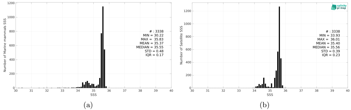
Figure 2: Histograms of SSS from Marine mammals (a) and SMOS SSS L4 v1 - Weekly (CMEMS-CNR) (b) considering all match-up pairs per bins of 0.1 over the South Pacific Ocean Pi-MEP region and for the full satellite product period.
