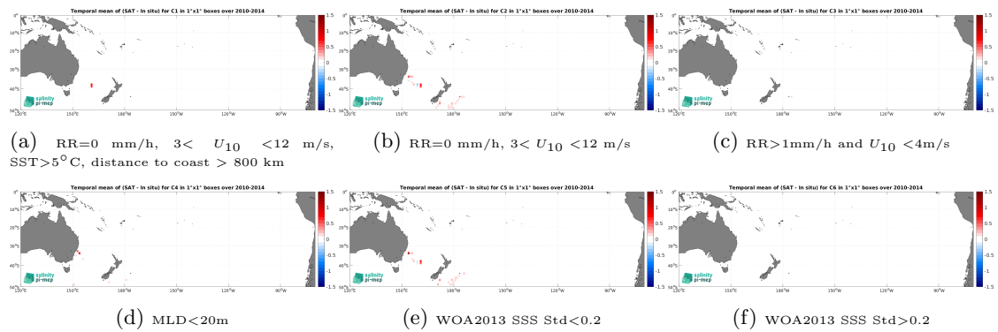
Figure 12: Temporal mean gridded over spatial boxes of size 1^\circ \times 1^\circ of \Delta SSS (SMOS SSS L4 v1 - Weekly (CMEMS-CNR) - Marine mammals) for 6 different subdatasets corresponding to:RR=0 mm/h, 3 < U_{10} < 12 m/s, SST > 5^\circ\text{C} , distance to coast > 800 km (a), RR=0 mm/h, 3 < U_{10} < 12 m/s (b), RR > 1 mm/h and U_{10} < 4 m/s (c),MLD < 20 m (d),WOA2013 SSS Std < 0.2 (e),WOA2013 SSS Std > 0.2 (f).
