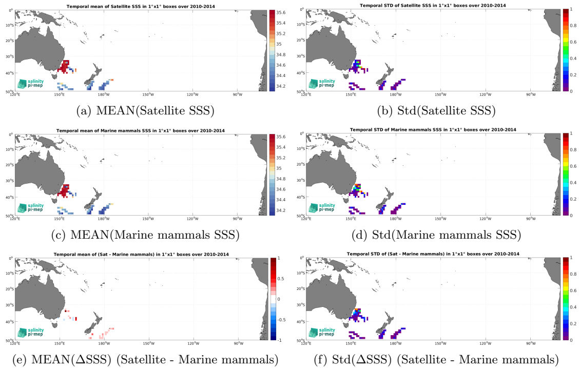
Figure 6: Temporal mean (left) and Std (right) of SSS from SMOS SSS L4 v1 - Weekly (CMEMS-CNR) (top), Marine mammals (middle), and of \Delta SSS (Satellite - Marine mammals). Only match-up pairs are used to generate these maps.
