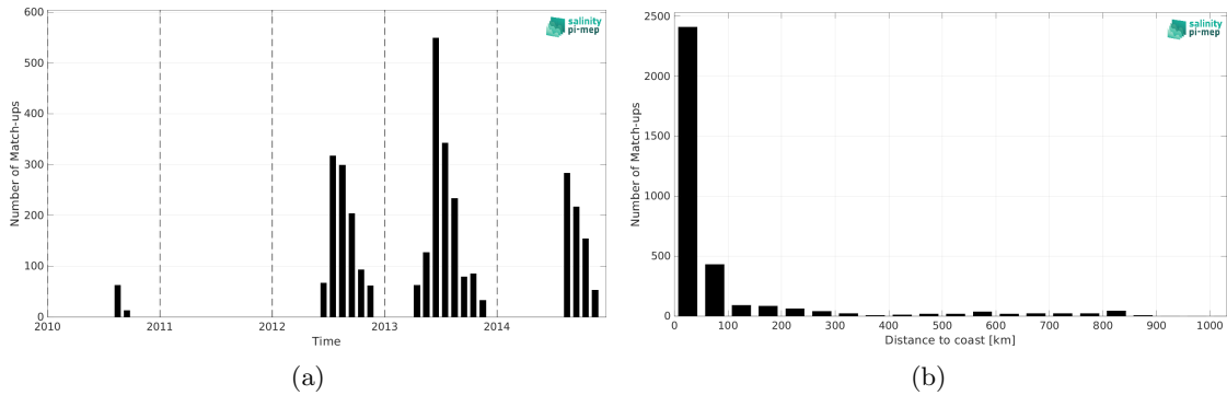
Figure 1: Number of match-ups between Marine mammals and SMOS SSS L4 v1 - Weekly (CMEMS-CNR) SSS as a function of time (a) and as function of the distance to coast (b) over the South Pacific Ocean Pi-MEP region and for the full satellite product period.
