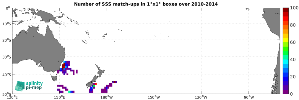
Figure 4: Number of SSS match-ups between Marine mammals SSS and the SMOS SSS L4 v1 - Weekly (CMEMS-CNR) SSS product for the South Pacific Ocean Pi-MEP region over 1^\circ \times 1^\circ boxes and for the full satellite product period.
