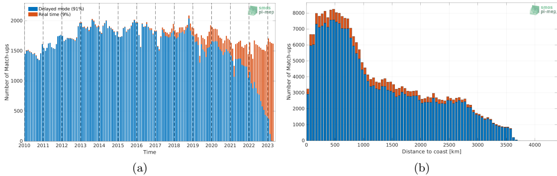
Figure 1: Number of match-ups between Argo and SMOS SSS L4 v1 - Weekly (CMEMS-CNR) SSS as a function of time (a) and as function of the distance to coast (b) over the South Pacific Ocean Pi-MEP region and for the full satellite product period.
