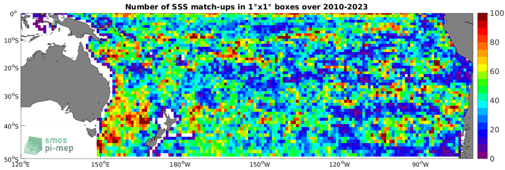
Figure 4: Number of SSS match-ups between Argo SSS and the SMOS SSS L4 v1 - Weekly (CMEMS-CNR) SSS product for the South Pacific Ocean Pi-MEP region over 1^\circ \times 1^\circ boxes and for the full satellite product period.
