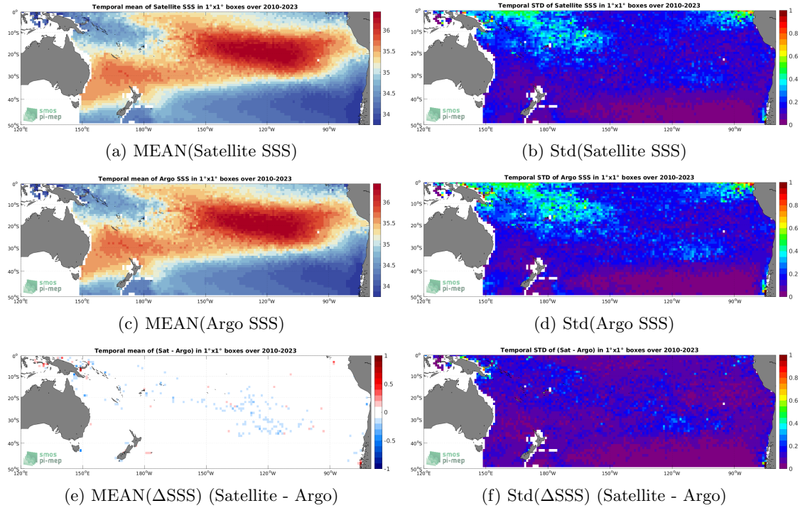
Figure 6: Temporal mean (left) and Std (right) of SSS from SMOS SSS L4 v1 - Weekly (CMEMS-CNR) (top), Argo (middle), and of \Delta SSS (Satellite - Argo). Only match-up pairs are used to generate these maps.
