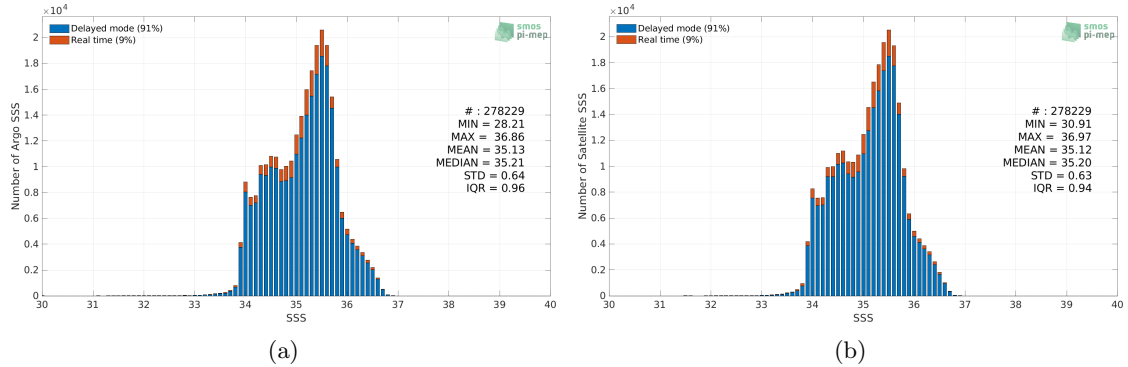
Figure 2: Histograms of SSS from Argo (a) and SMOS SSS L4 v1 - Weekly (CMEMS-CNR) (b) considering all match-up pairs per bins of 0.1 over the South Pacific Ocean Pi-MEP region and for the full satellite product period.
