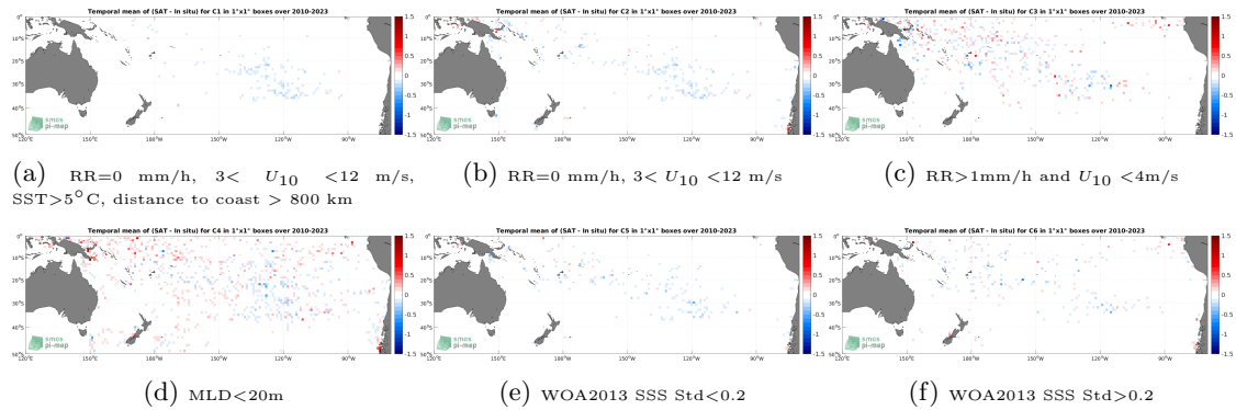
Figure 12: Temporal mean gridded over spatial boxes of size 1^\circ \times 1^\circ of \Delta SSS (SMOS SSS L4 v1 - Weekly (CMEMS-CNR) - Argo) for 6 different subdatasets corresponding to:RR=0 mm/h, 3 < U_{10} < 12 m/s, SST >5^\circ\text{C} , distance to coast > 800 km (a), RR=0 mm/h, 3 < U_{10} < 12 m/s (b), RR >1 mm/h and U_{10} < 4 m/s (c),MLD <20 m (d),WOA2013 SSS Std <0.2 (e),WOA2013 SSS Std >0.2 (f).
