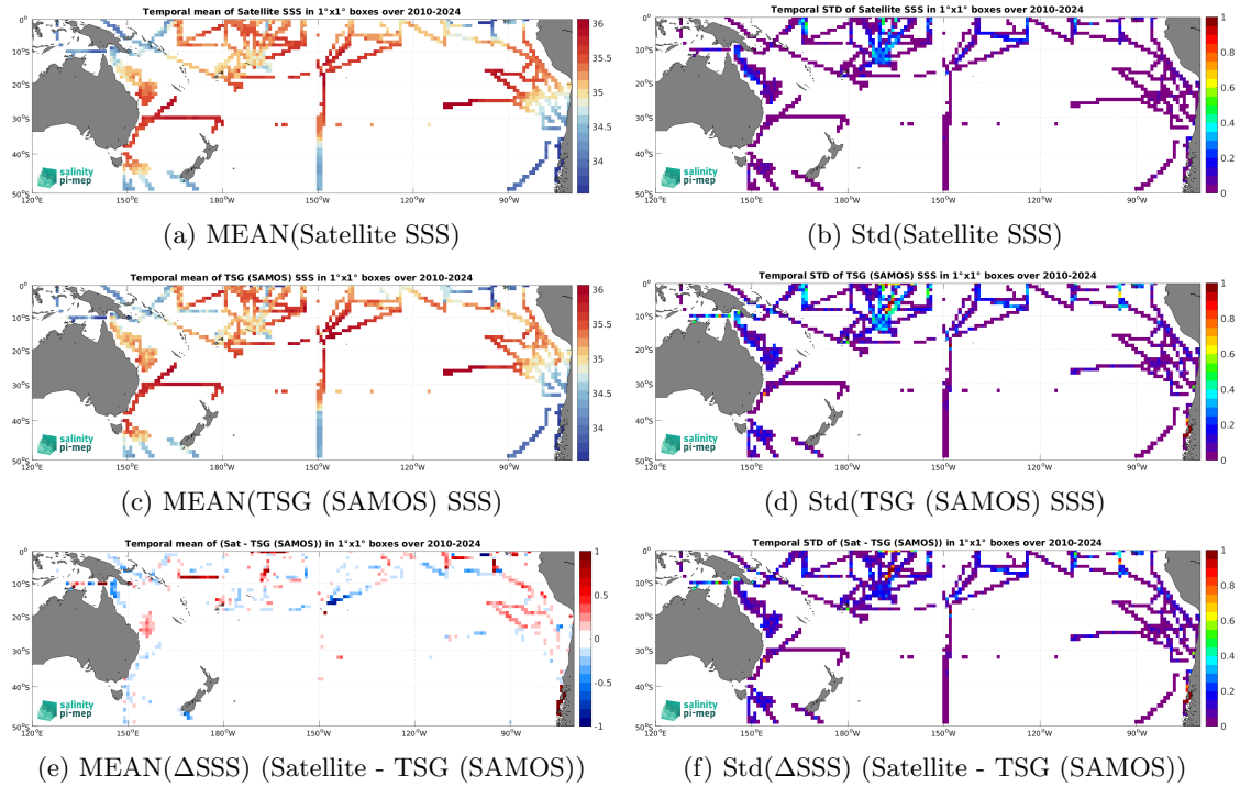
Figure 7: Temporal mean (left) and Std (right) of SSS from SMOS SSS L4 v1 - Monthly (CMEMS-CNR) (top), TSG (SAMOS) (middle), and of \Delta SSS (Satellite - TSG (SAMOS)). Only match-up pairs are used to generate these maps.
