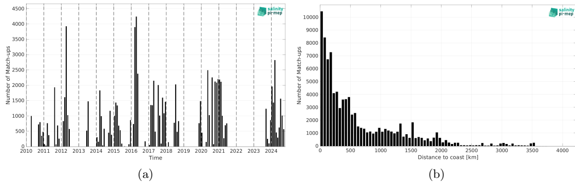
Figure 2: Number of match-ups between TSG (SAMOS) and SMOS SSS L4 v1 - Monthly (CMEMS-CNR) SSS as a function of time (a) and as function of the distance to coast (b) over the South Pacific Ocean Pi-MEP region and for the full satellite product period.
