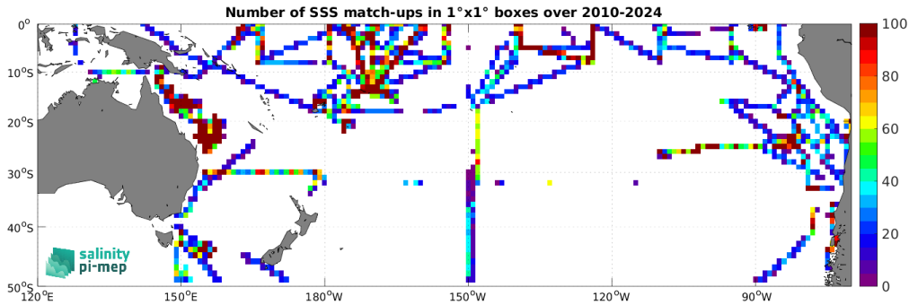
Figure 5: Number of SSS match-ups between TSG (SAMOS) SSS and the SMOS SSS L4 v1 - Monthly (CMEMS-CNR) SSS product for the South Pacific Ocean Pi-MEP region over 1^\circ \times 1^\circ boxes and for the full satellite product period.
