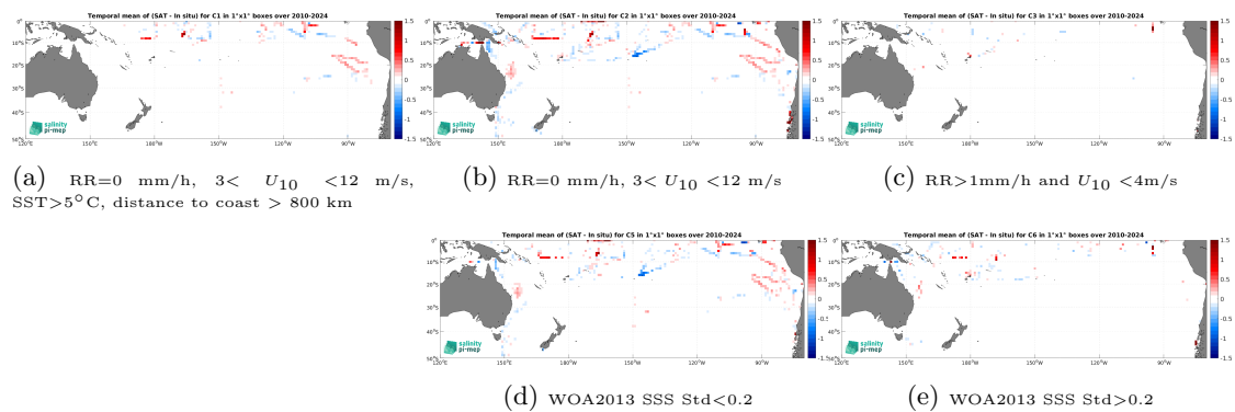
Figure 14: Temporal mean gridded over spatial boxes of size 1^\circ \times 1^\circ of \Delta SSS (SMOS SSS L4 v1 - Monthly (CMEMS-CNR) - TSG (SAMOS)) for 5 different subdatasets corresponding to:RR=0 mm/h, 3 < U_{10} < 12 m/s, SST >5^\circ\text{C} , distance to coast > 800 km (a), RR=0 mm/h, 3 < U_{10} < 12 m/s (b), RR >1 mm/h and U_{10} < 4 m/s (c), WOA2013 SSS Std <0.2 (d), WOA2013 SSS Std >0.2 (e).
