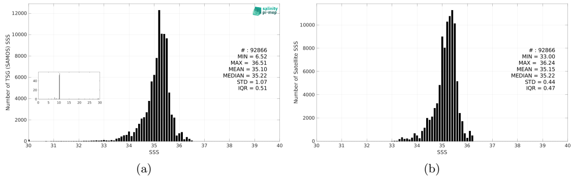
Figure 3: Histograms of SSS from TSG (SAMOS) (a) and SMOS SSS L4 v1 - Monthly (CMEMS-CNR) (b) considering all match-up pairs per bins of 0.1 over the South Pacific Ocean Pi-MEP region and for the full satellite product period.
