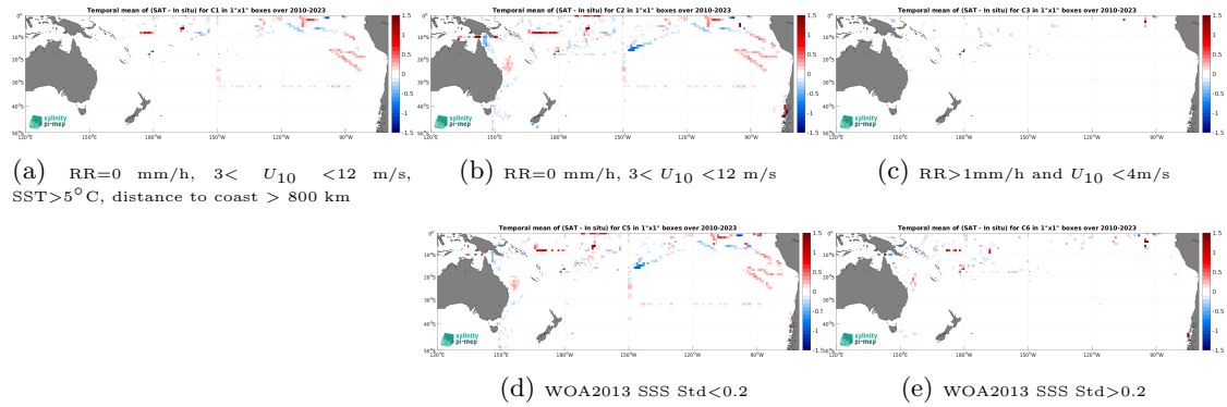
Figure 12: Temporal mean gridded over spatial boxes of size 1^\circ \times 1^\circ of \Delta\text{SSS} (SMOS SSS L4 v1 - Monthly (CMEMS-CNR) - TSG (SAMOS)) for 5 different subdatasets corresponding to:RR=0 mm/h, 3 < U_{10} < 12 m/s, SST >5^\circ\text{C} , distance to coast > 800 km (a), RR=0 mm/h, 3 < U_{10} < 12 m/s (b), RR >1 mm/h and U_{10} < 4 m/s (c), WOA2013 SSS Std <0.2 (d), WOA2013 SSS Std >0.2 (e).
