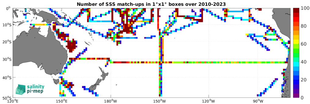
Figure 4: Number of SSS match-ups between TSG (SAMOS) SSS and the SMOS SSS L4 v1 - Monthly (CMEMS-CNR) SSS product for the South Pacific Ocean Pi-MEP region over 1^\circ \times 1^\circ boxes and for the full satellite product period.
