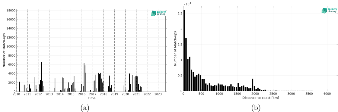
Figure 1: Number of match-ups between TSG (SAMOS) and SMOS SSS L4 v1 - Monthly (CMEMS-CNR) SSS as a function of time (a) and as function of the distance to coast (b) over the South Pacific Ocean Pi-MEP region and for the full satellite product period.
