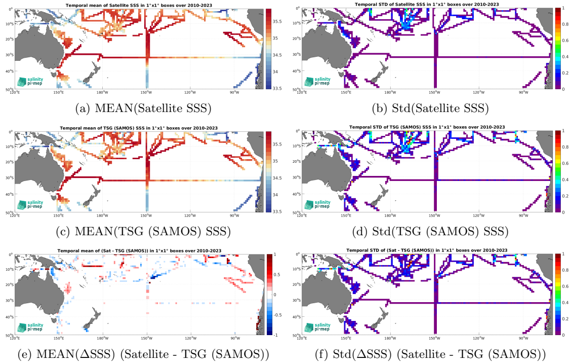
Figure 6: Temporal mean (left) and Std (right) of SSS from SMOS SSS L4 v1 - Monthly (CMEMS-CNR) (top), TSG (SAMOS) (middle), and of \Delta SSS (Satellite - TSG (SAMOS)). Only match-up pairs are used to generate these maps.
