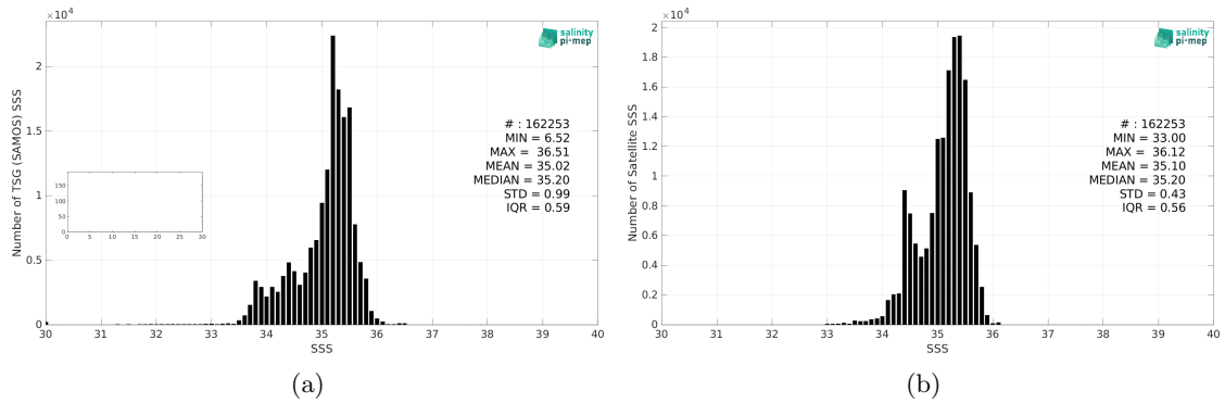
Figure 2: Histograms of SSS from TSG (SAMOS) (a) and SMOS SSS L4 v1 - Monthly (CMEMS-CNR) (b) considering all match-up pairs per bins of 0.1 over the South Pacific Ocean Pi-MEP region and for the full satellite product period.
