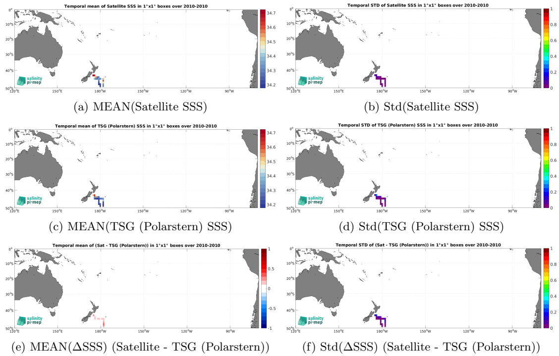
Figure 7: Temporal mean (left) and Std (right) of SSS from SMOS SSS L4 v1 - Monthly (CMEMS-CNR) (top), TSG (Polarstern) (middle), and of \Delta SSS (Satellite - TSG (Polarstern)). Only match-up pairs are used to generate these maps.
