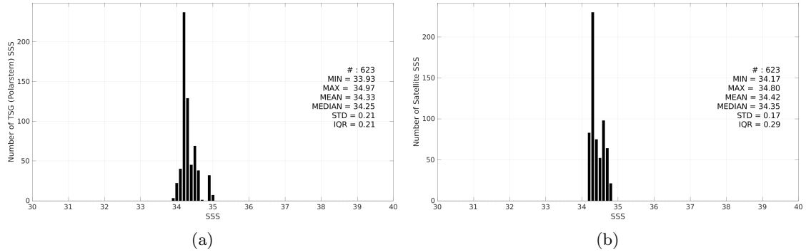
Figure 3: Histograms of SSS from TSG (Polarstern) (a) and SMOS SSS L4 v1 - Monthly (CMEMS-CNR) (b) considering all match-up pairs per bins of 0.1 over the South Pacific Ocean Pi-MEP region and for the full satellite product period.
