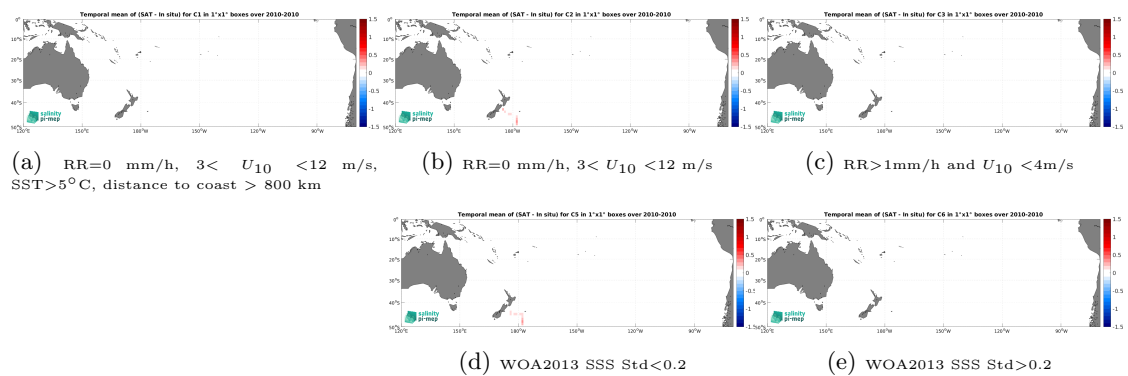
Figure 14: Temporal mean gridded over spatial boxes of size 1^\circ \times 1^\circ of \Delta SSS (SMOS SSS L4 v1 - Monthly (CMEMS-CNR) - TSG (Polarstern)) for 5 different subdatasets corresponding to:RR=0 mm/h, 3 < U_{10} < 12 m/s, SST >5^\circ\text{C} , distance to coast > 800 km (a), RR=0 mm/h, 3 < U_{10} < 12 m/s (b), RR >1 mm/h and U_{10} < 4 m/s (c), WOA2013 SSS Std <0.2 (d), WOA2013 SSS Std >0.2 (e).
