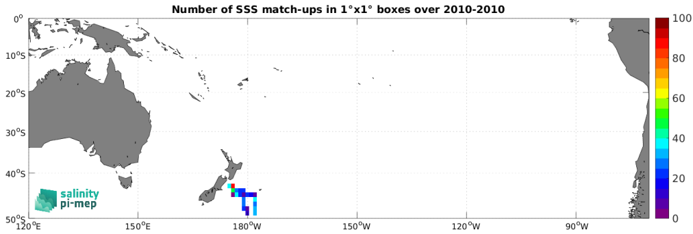
Figure 5: Number of SSS match-ups between TSG (Polarstern) SSS and the SMOS SSS L4 v1 - Monthly (CMEMS-CNR) SSS product for the South Pacific Ocean Pi-MEP region over 1^\circ \times 1^\circ boxes and for the full satellite product period.
