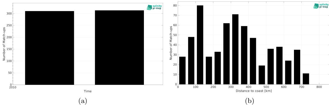
Figure 2: Number of match-ups between TSG (Polarstern) and SMOS SSS L4 v1 - Monthly (CMEMS-CNR) SSS as a function of time (a) and as function of the distance to coast (b) over the South Pacific Ocean Pi-MEP region and for the full satellite product period.
