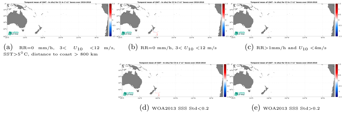
Figure 12: Temporal mean gridded over spatial boxes of size 1^{\circ}\times 1^{\circ} of \Delta\text{SSS} (SMOS SSS L4 v1 - Monthly (CMEMS-CNR) - TSG (Polarstern)) for 5 different subdatasets corresponding to:RR=0 mm/h, 3 < U_{10} < 12 m/s, SST > 5^{\circ}\text{C} , distance to coast > 800 km (a), RR=0 mm/h, 3 < U_{10} < 12 m/s (b), RR > 1 mm/h and U_{10} < 4 m/s (c), WOA2013 SSS Std < 0.2 (d), WOA2013 SSS Std > 0.2 (e).
