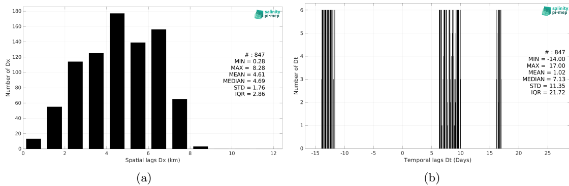
Figure 5: Histograms of the spatial (a) and temporal (b) lags between the location/time of the TSG (Polarstern) measurement and the date of the corresponding SMOS SSS L4 v1 - Monthly (CMEMS-CNR) SSS pixel.
