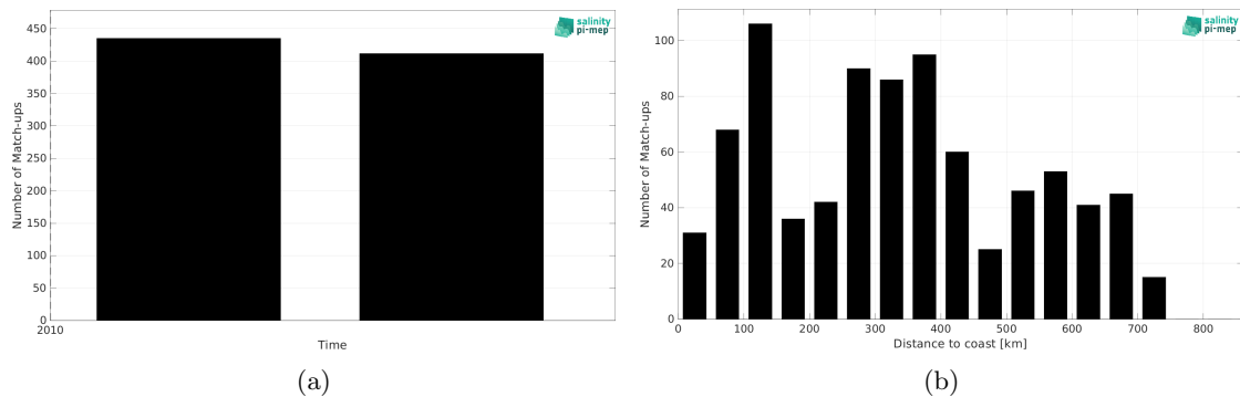
Figure 1: Number of match-ups between TSG (Polarstern) and SMOS SSS L4 v1 - Monthly (CMEMS-CNR) SSS as a function of time (a) and as function of the distance to coast (b) over the South Pacific Ocean Pi-MEP region and for the full satellite product period.
