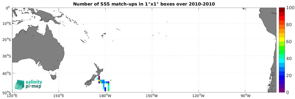
Figure 4: Number of SSS match-ups between TSG (Polarstern) SSS and the SMOS SSS L4 v1 - Monthly (CMEMS-CNR) SSS product for the South Pacific Ocean Pi-MEP region over 1^\circ \times 1^\circ boxes and for the full satellite product period.
