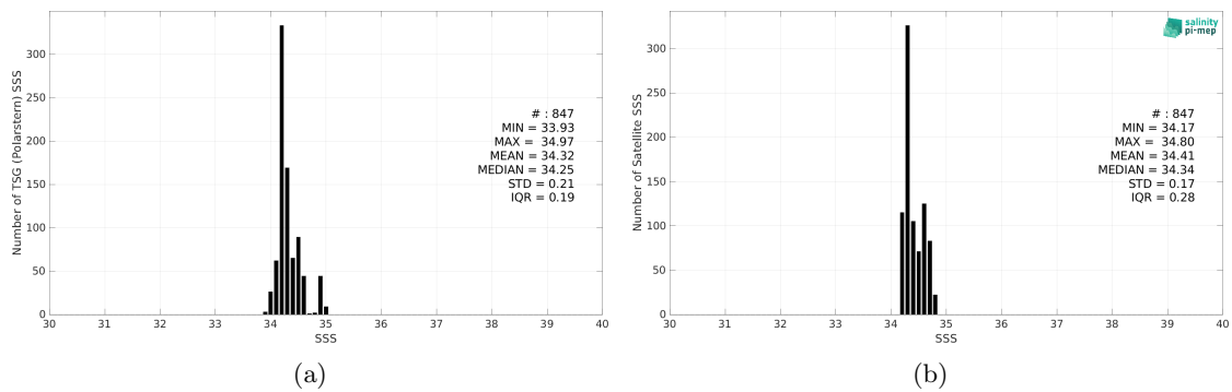
Figure 2: Histograms of SSS from TSG (Polarstern) (a) and SMOS SSS L4 v1 - Monthly (CMEMS-CNR) (b) considering all match-up pairs per bins of 0.1 over the South Pacific Ocean Pi-MEP region and for the full satellite product period.
