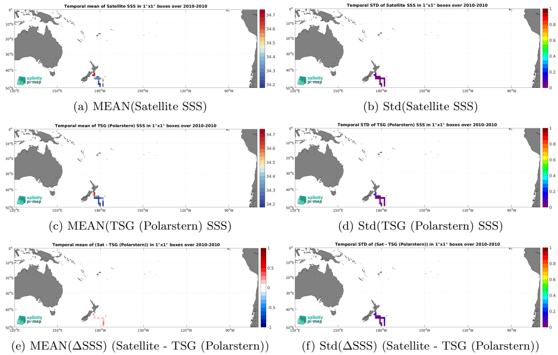
Figure 6: Temporal mean (left) and Std (right) of SSS from SMOS SSS L4 v1 - Monthly (CMEMS-CNR) (top), TSG (Polarstern) (middle), and of \Delta SSS (Satellite - TSG (Polarstern)). Only match-up pairs are used to generate these maps.
