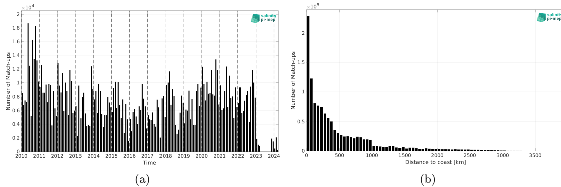
Figure 2: Number of match-ups between TSG (LEGOS-DM) and SMOS SSS L4 v1 - Monthly (CMEMS-CNR) SSS as a function of time (a) and as function of the distance to coast (b) over the South Pacific Ocean Pi-MEP region and for the full satellite product period.
