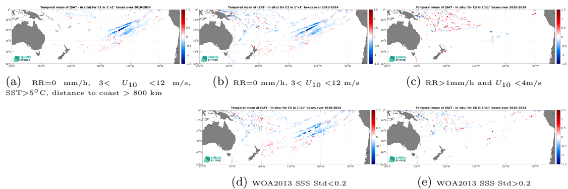
Figure 14: Temporal mean gridded over spatial boxes of size 1^\circ \times 1^\circ of \Delta\text{SSS} (SMOS SSS L4 v1 - Monthly (CMEMS-CNR) - TSG (LEGOS-DM)) for 5 different subdatasets corresponding to:RR=0 mm/h, 3 < U_{10} < 12 m/s, SST>5°C, distance to coast > 800 km (a), RR=0 mm/h, 3 < U_{10} < 12 m/s (b), RR>1mm/h and U_{10} < 4 m/s (c), WOA2013 SSS Std<0.2 (d), WOA2013 SSS Std>0.2 (e).
