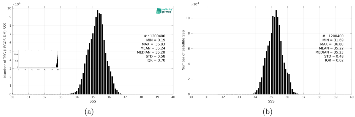
Figure 3: Histograms of SSS from TSG (LEGOS-DM) (a) and SMOS SSS L4 v1 - Monthly (CMEMS-CNR) (b) considering all match-up pairs per bins of 0.1 over the South Pacific Ocean Pi-MEP region and for the full satellite product period.
