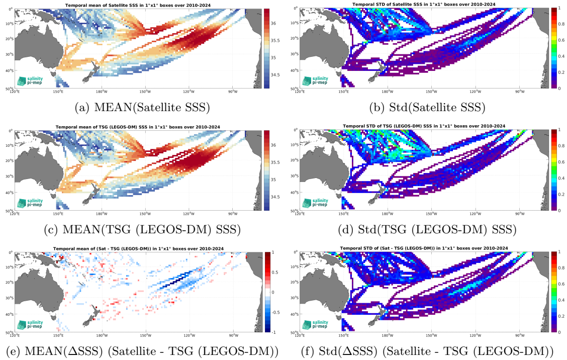
Figure 7: Temporal mean (left) and Std (right) of SSS from SMOS SSS L4 v1 - Monthly (CMEMS-CNR) (top), TSG (LEGOS-DM) (middle), and of \Delta SSS (Satellite - TSG (LEGOS-DM)). Only match-up pairs are used to generate these maps.
