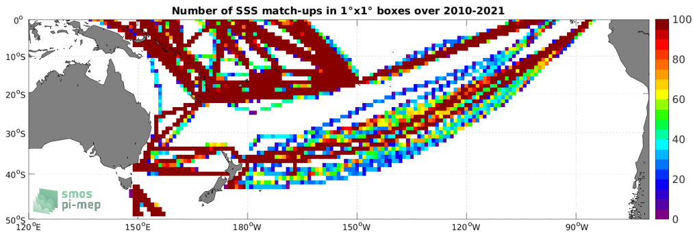
Figure 4: Number of SSS match-ups between TSG (LEGOS-DM) SSS and the SMOS SSS L4 v1 - Monthly (CMEMS-CNR) SSS product for the South Pacific Ocean Pi-MEP region over 1^\circ \times 1^\circ boxes and for the full satellite product period.
