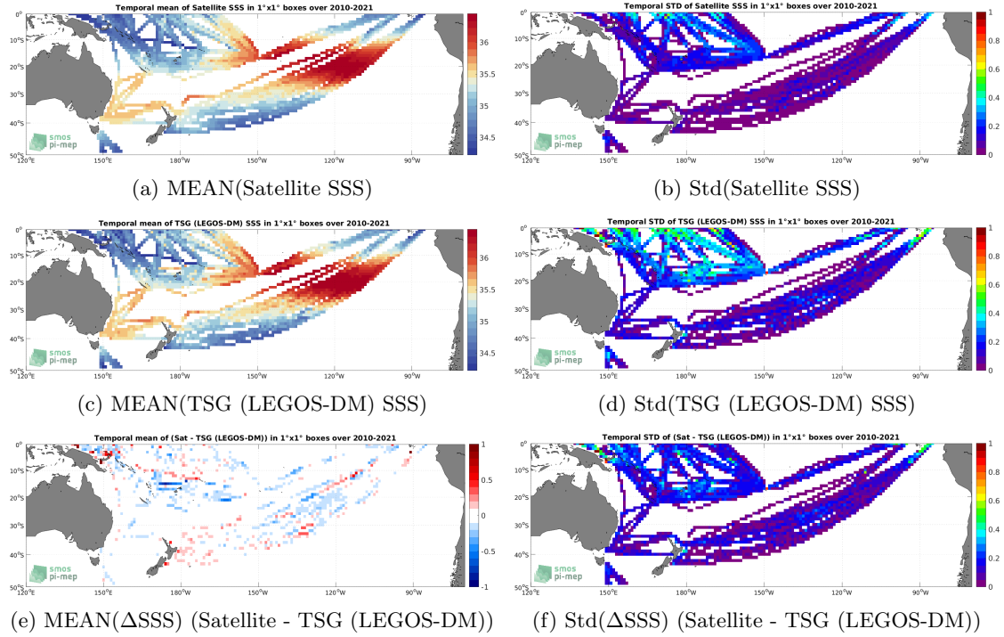
Figure 6: Temporal mean (left) and Std (right) of SSS from SMOS SSS L4 v1 - Monthly (CMEMS-CNR) (top), TSG (LEGOS-DM) (middle), and of \Delta SSS (Satellite - TSG (LEGOS-DM)). Only match-up pairs are used to generate these maps.
