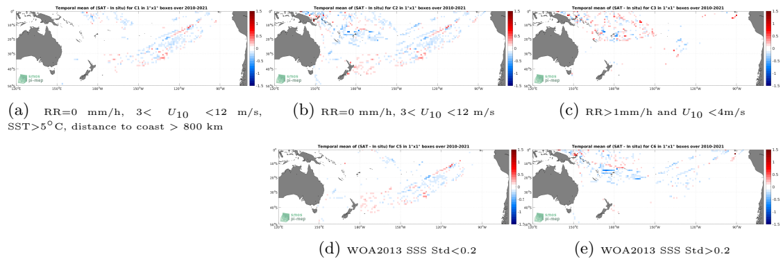
Figure 12: Temporal mean gridded over spatial boxes of size 1^\circ \times 1^\circ of \Delta SSS (SMOS SSS L4 v1 - Monthly (CMEMS-CNR) - TSG (LEGOS-DM)) for 5 different subdatasets corresponding to:RR=0 mm/h, 3 < U_{10} < 12 m/s, SST >5^\circ C, distance to coast > 800 km (a), RR=0 mm/h, 3 < U_{10} < 12 m/s (b), RR >1 mm/h and U_{10} < 4 m/s (c), WOA2013 SSS Std <0.2 (d), WOA2013 SSS Std >0.2 (e).
