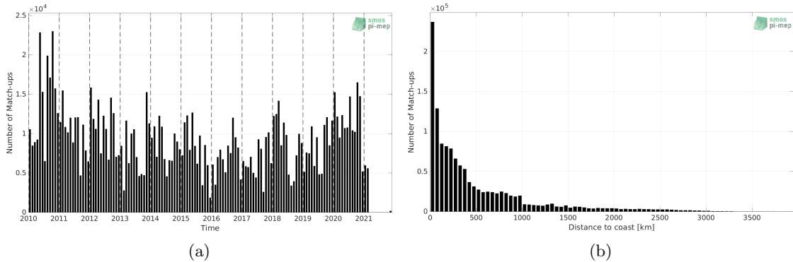
Figure 1: Number of match-ups between TSG (LEGOS-DM) and SMOS SSS L4 v1 - Monthly (CMEMS-CNR) SSS as a function of time (a) and as function of the distance to coast (b) over the South Pacific Ocean Pi-MEP region and for the full satellite product period.
