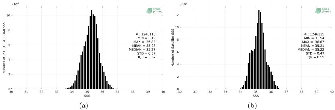
Figure 2: Histograms of SSS from TSG (LEGOS-DM) (a) and SMOS SSS L4 v1 - Monthly (CMEMS-CNR) (b) considering all match-up pairs per bins of 0.1 over the South Pacific Ocean Pi-MEP region and for the full satellite product period.
