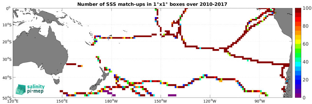
Figure 5: Number of SSS match-ups between TSG (GOSUD-Sailing-ship) SSS and the SMOS SSS L4 v1 - Monthly (CMEMS-CNR) SSS product for the South Pacific Ocean Pi-MEP region over 1^\circ \times 1^\circ boxes and for the full satellite product period.
