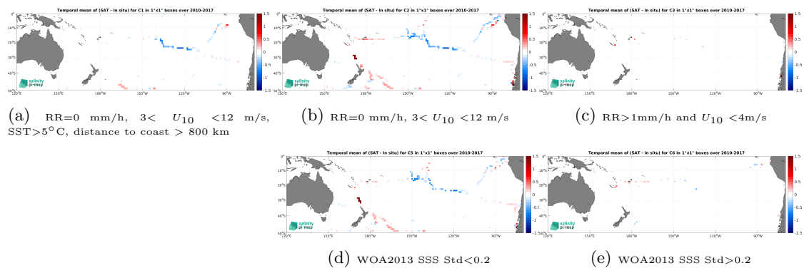
Figure 14: Temporal mean gridded over spatial boxes of size 1^\circ \times 1^\circ of \Delta SSS (SMOS SSS L4 v1 - Monthly (CMEMS-CNR) - TSG (GOSUD-Sailing-ship)) for 5 different subdatasets corresponding to:RR=0 mm/h, 3 < U_{10} < 12 m/s, SST >5^\circ C, distance to coast > 800 km (a), RR=0 mm/h, 3 < U_{10} < 12 m/s (b), RR >1 mm/h and U_{10} < 4 m/s (c), WOA2013 SSS Std <0.2 (d), WOA2013 SSS Std >0.2 (e).
