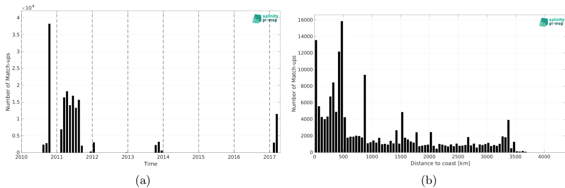
Figure 2: Number of match-ups between TSG (GOSUD-Sailing-ship) and SMOS SSS L4 v1 - Monthly (CMEMS-CNR) SSS as a function of time (a) and as function of the distance to coast (b) over the South Pacific Ocean Pi-MEP region and for the full satellite product period.
