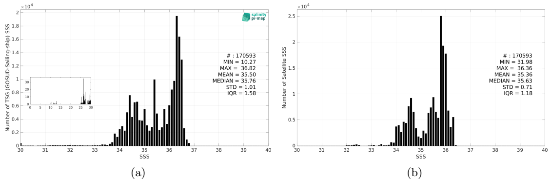
Figure 3: Histograms of SSS from TSG (GOSUD-Sailing-ship) (a) and SMOS SSS L4 v1 - Monthly (CMEMS-CNR) (b) considering all match-up pairs per bins of 0.1 over the South Pacific Ocean Pi-MEP region and for the full satellite product period.
