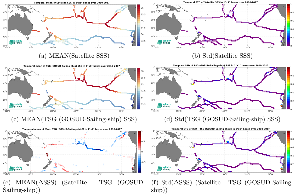
Figure 7: Temporal mean (left) and Std (right) of SSS from SMOS SSS L4 v1 - Monthly (CMEMS-CNR) (top), TSG (GOSUD-Sailing-ship) (middle), and of \Delta SSS (Satellite - TSG (GOSUD-Sailing-ship)). Only match-up pairs are used to generate these maps.
