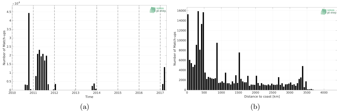
Figure 1: Number of match-ups between TSG (GOSUD-Sailing-ship) and SMOS SSS L4 v1 - Monthly (CMEMS-CNR) SSS as a function of time (a) and as function of the distance to coast (b) over the South Pacific Ocean Pi-MEP region and for the full satellite product period.
