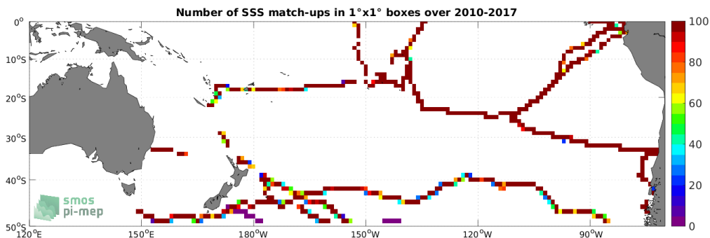
Figure 4: Number of SSS match-ups between TSG (GOSUD-Sailing-ship) SSS and the SMOS SSS L4 v1 - Monthly (CMEMS-CNR) SSS product for the South Pacific Ocean Pi-MEP region over 1^\circ \times 1^\circ boxes and for the full satellite product period.
