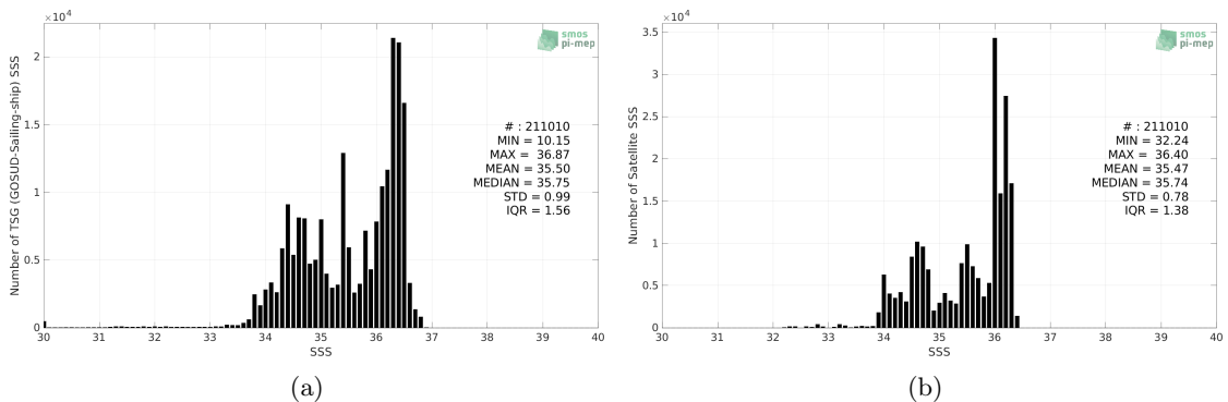
Figure 2: Histograms of SSS from TSG (GOSUD-Sailing-ship) (a) and SMOS SSS L4 v1 - Monthly (CMEMS-CNR) (b) considering all match-up pairs per bins of 0.1 over the South Pacific Ocean Pi-MEP region and for the full satellite product period.
