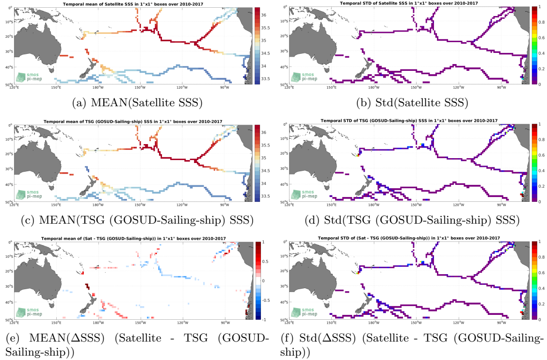
Figure 6: Temporal mean (left) and Std (right) of SSS from SMOS SSS L4 v1 - Monthly (CMEMS-CNR) (top), TSG (GOSUD-Sailing-ship) (middle), and of \Delta SSS (Satellite - TSG (GOSUD-Sailing-ship)). Only match-up pairs are used to generate these maps.
