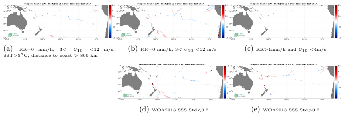
Figure 12: Temporal mean gridded over spatial boxes of size 1^\circ \times 1^\circ of \Delta\text{SSS} (SMOS SSS L4 v1 - Monthly (CMEMS-CNR) - TSG (GOSUD-Sailing-ship)) for 5 different subdatasets corresponding to:RR=0 mm/h, 3 < U_{10} < 12 m/s, SST>5°C, distance to coast > 800 km (a), RR=0 mm/h, 3 < U_{10} < 12 m/s (b), RR>1mm/h and U_{10} < 4 m/s (c), WOA2013 SSS Std<0.2 (d), WOA2013 SSS Std>0.2 (e).
