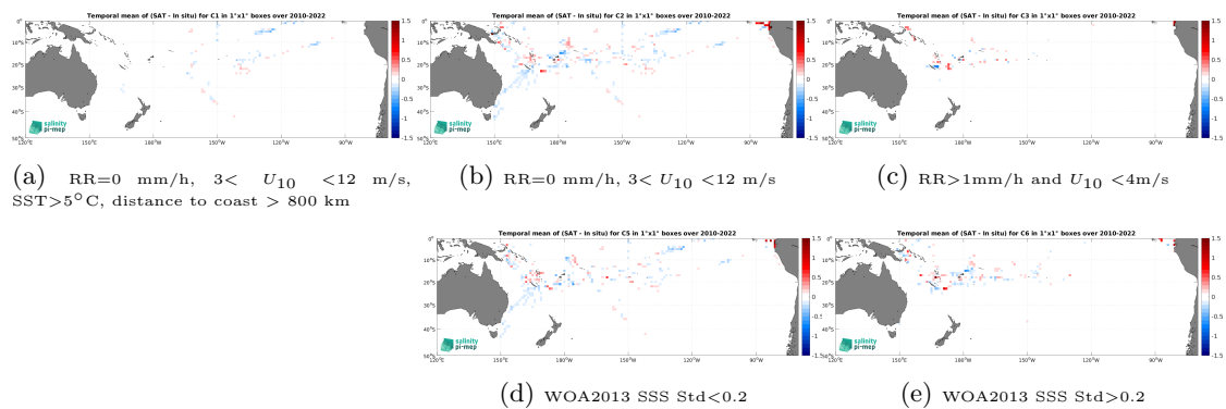
Figure 14: Temporal mean gridded over spatial boxes of size 1^\circ \times 1^\circ of \Delta SSS (SMOS SSS L4 v1 - Monthly (CMEMS-CNR) - TSG (GOSUD-Research-vessel)) for 5 different subdatasets corresponding to:RR=0 mm/h, 3 < U_{10} < 12 m/s, SST >5^\circ\text{C} , distance to coast > 800 km (a), RR=0 mm/h, 3 < U_{10} < 12 m/s (b), RR >1 mm/h and U_{10} < 4 m/s (c), WOA2013 SSS Std <0.2 (d), WOA2013 SSS Std >0.2 (e).
