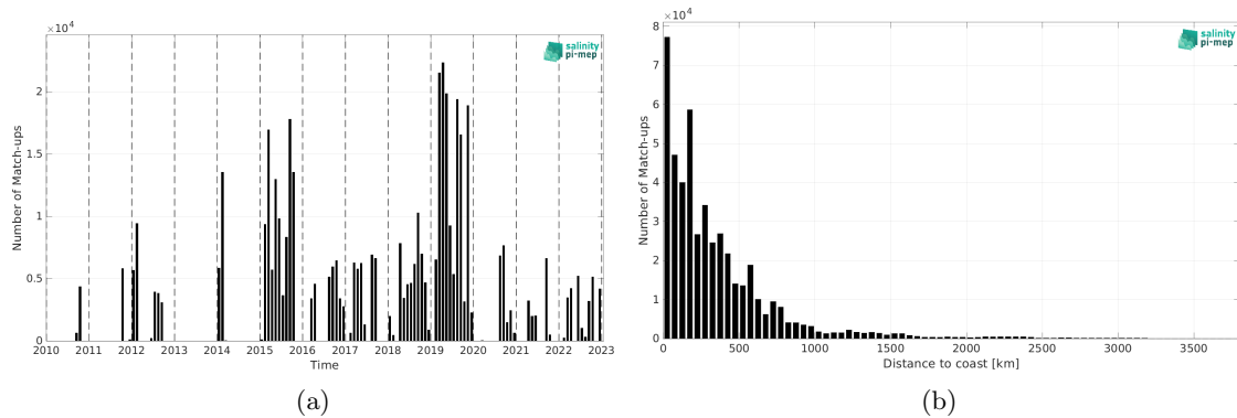
Figure 2: Number of match-ups between TSG (GOSUD-Research-vessel) and SMOS SSS L4 v1 - Monthly (CMEMS-CNR) SSS as a function of time (a) and as function of the distance to coast (b) over the South Pacific Ocean Pi-MEP region and for the full satellite product period.
