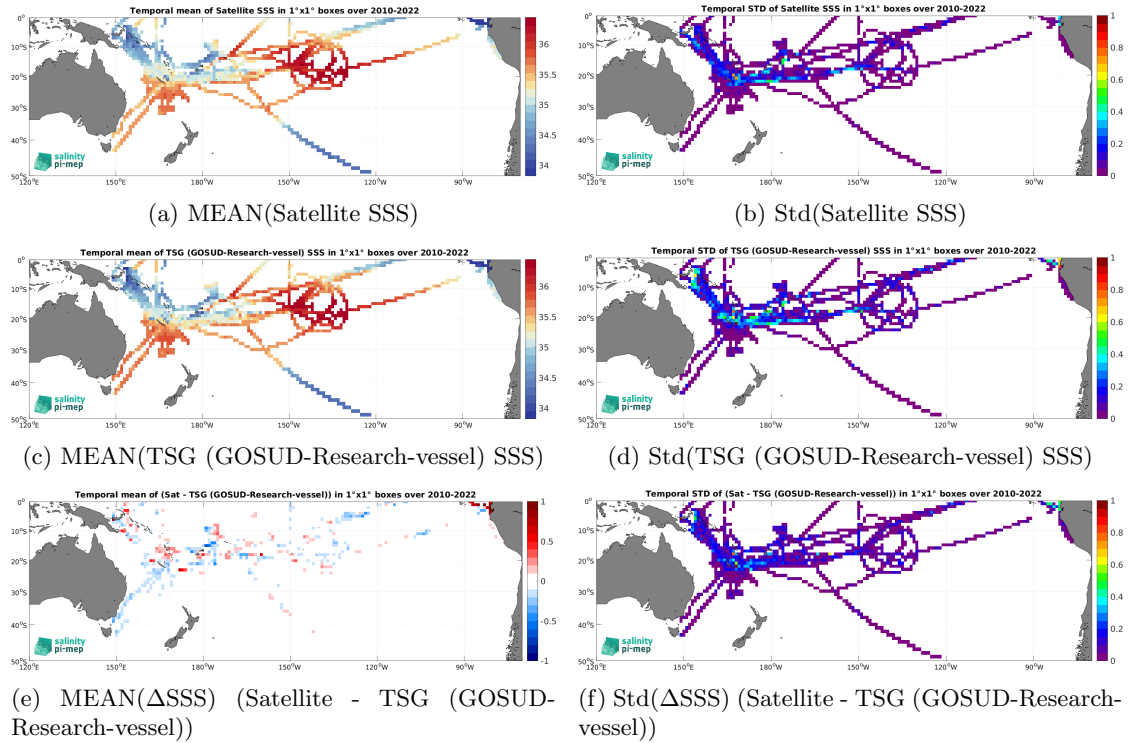
Figure 7: Temporal mean (left) and Std (right) of SSS from SMOS SSS L4 v1 - Monthly (CMEMS-CNR) (top), TSG (GOSUD-Research-vessel) (middle), and of \Delta SSS (Satellite - TSG (GOSUD-Research-vessel)). Only match-up pairs are used to generate these maps.
