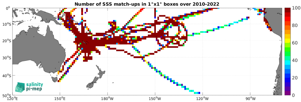
Figure 5: Number of SSS match-ups between TSG (GOSUD-Research-vessel) SSS and the SMOS SSS L4 v1 - Monthly (CMEMS-CNR) SSS product for the South Pacific Ocean Pi-MEP region over 1^\circ \times 1^\circ boxes and for the full satellite product period.
