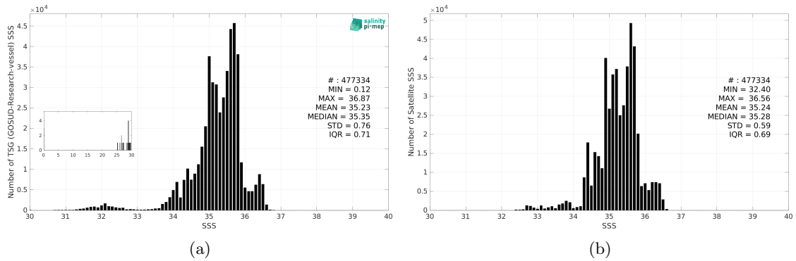
Figure 3: Histograms of SSS from TSG (GOSUD-Research-vessel) (a) and SMOS SSS L4 v1 - Monthly (CMEMS-CNR) (b) considering all match-up pairs per bins of 0.1 over the South Pacific Ocean Pi-MEP region and for the full satellite product period.
