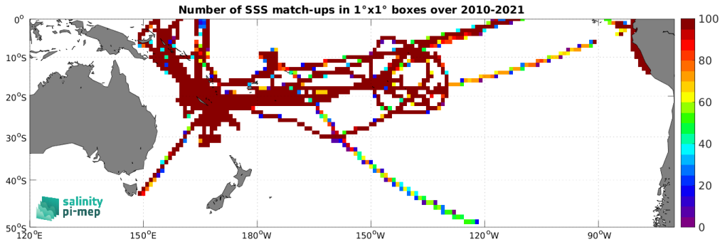
Figure 4: Number of SSS match-ups between TSG (GOSUD-Research-vessel) SSS and the SMOS SSS L4 v1 - Monthly (CMEMS-CNR) SSS product for the South Pacific Ocean Pi-MEP region over 1^\circ \times 1^\circ boxes and for the full satellite product period.
