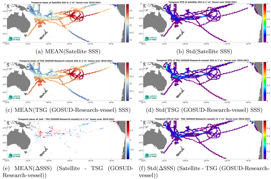
Figure 6: Temporal mean (left) and Std (right) of SSS from SMOS SSS L4 v1 - Monthly (CMEMS-CNR) (top), TSG (GOSUD-Research-vessel) (middle), and of \Delta SSS (Satellite - TSG (GOSUD-Research-vessel)). Only match-up pairs are used to generate these maps.
