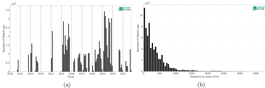
Figure 1: Number of match-ups between TSG (GOSUD-Research-vessel) and SMOS SSS L4 v1 - Monthly (CMEMS-CNR) SSS as a function of time (a) and as function of the distance to coast (b) over the South Pacific Ocean Pi-MEP region and for the full satellite product period.
