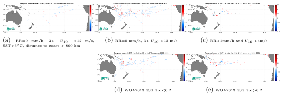
Figure 12: Temporal mean gridded over spatial boxes of size 1^\circ \times 1^\circ of \Delta SSS (SMOS SSS L4 v1 - Monthly (CMEMS-CNR) - TSG (GOSUD-Research-vessel)) for 5 different subdatasets corresponding to:RR=0 mm/h, 3 < U_{10} < 12 m/s, SST >5^\circ\text{C} , distance to coast > 800 km (a), RR=0 mm/h, 3 < U_{10} < 12 m/s (b), RR >1 mm/h and U_{10} < 4 m/s (c), WOA2013 SSS Std <0.2 (d), WOA2013 SSS Std >0.2 (e).
