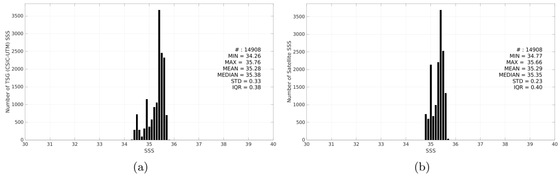
Figure 3: Histograms of SSS from TSG (CSIC-UTM) (a) and SMOS SSS L4 v1 - Monthly (CMEMS-CNR) (b) considering all match-up pairs per bins of 0.1 over the South Pacific Ocean Pi-MEP region and for the full satellite product period.
