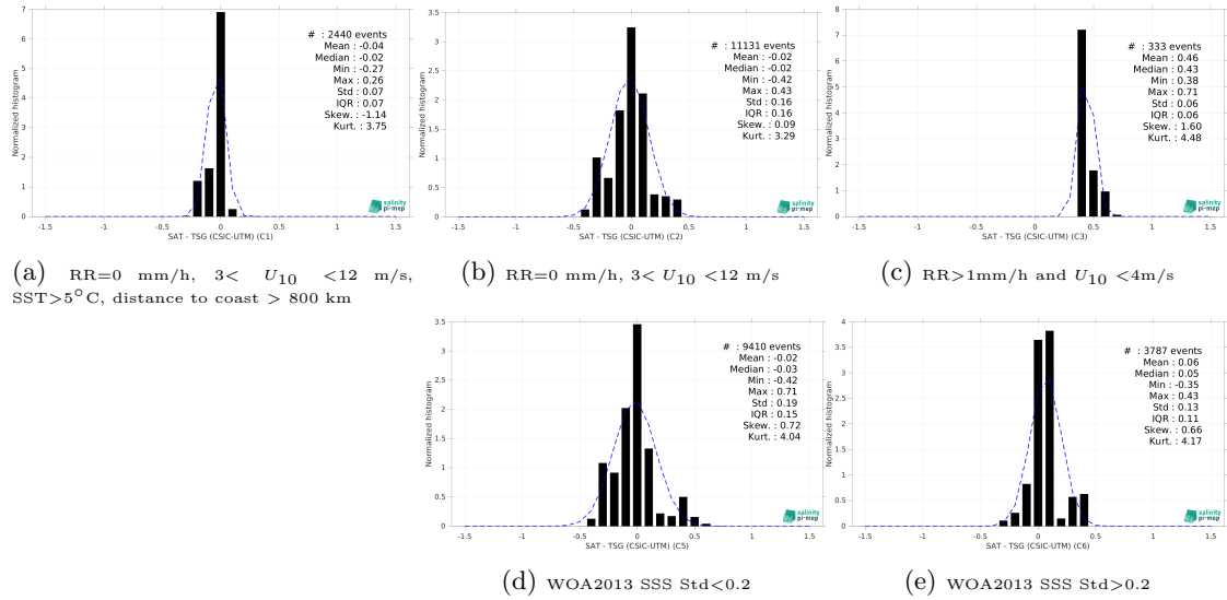
Figure 15: Normalized histogram of \Delta SSS (SMOS SSS L4 v1 - Monthly (CMEMS-CNR) - TSG (CSIC-UTM)) for 5 different subdatasets corresponding to: RR=0 mm/h, 3 < U_{10} < 12 m/s, SST > 5°C, distance to coast > 800 km (a), RR=0 mm/h, 3 < U_{10} < 12 m/s (b), RR > 1mm/h and U_{10} < 4 m/s (c), WOA2013 SSS Std < 0.2 (d), WOA2013 SSS Std > 0.2 (e).
