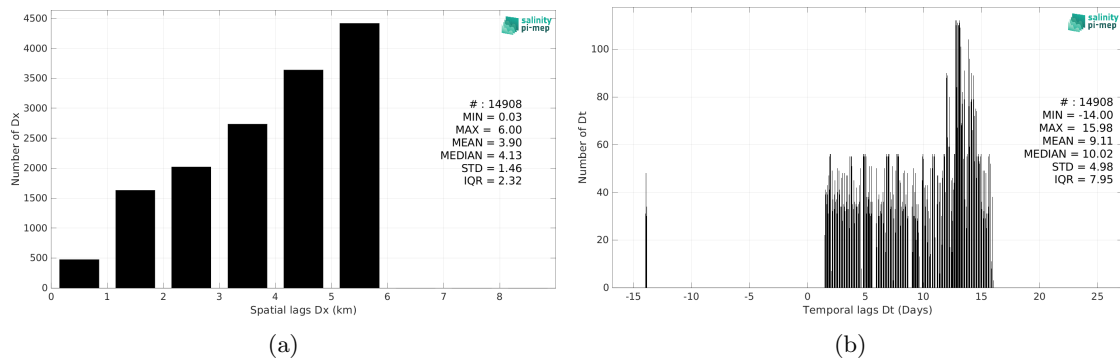
Figure 6: Histograms of the spatial (a) and temporal (b) lags between the location/time of the TSG (CSIC-UTM) measurement and the date of the corresponding SMOS SSS L4 v1 - Monthly (CMEMS-CNR) SSS pixel.
