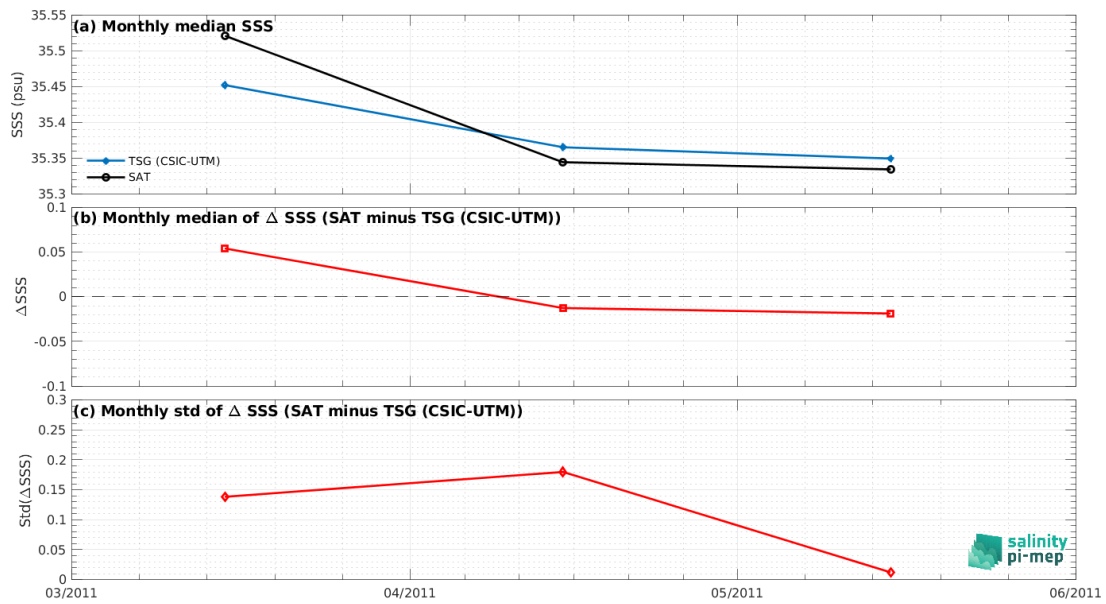
Figure 8: Time series of the monthly median SSS (top), median of \Delta SSS (Satellite - TSG (CSIC-UTM)) and Std of \Delta SSS (Satellite - TSG (CSIC-UTM)) over the South Pacific Ocean Pi-MEP region considering all match-ups collected by the Pi-MEP.
