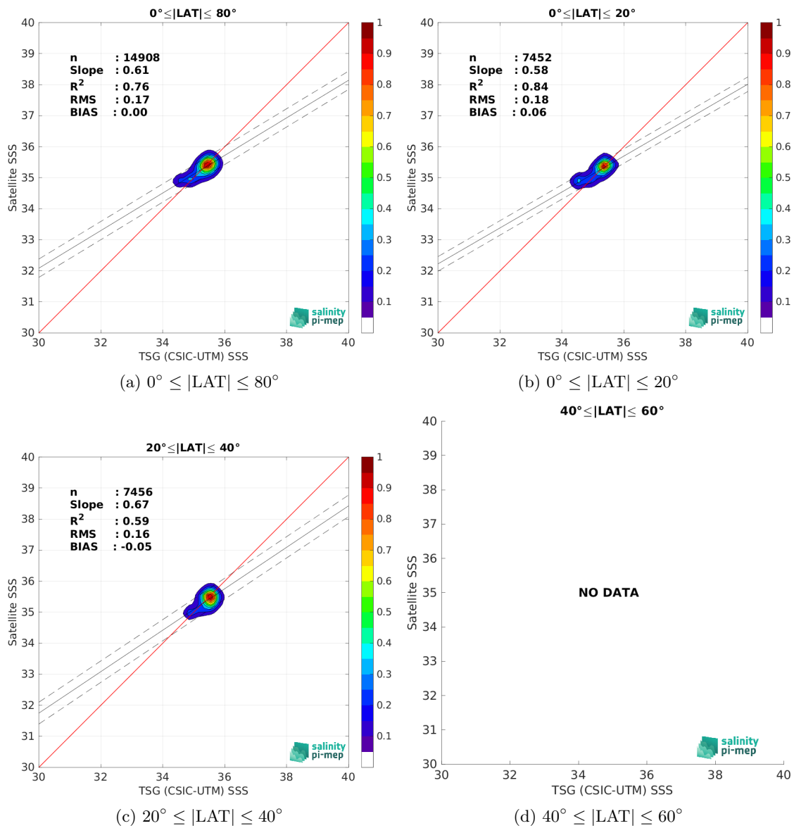
Figure 10: Contour maps of the concentration of SMOS SSS L4 v1 - Monthly (CMEMS-CNR) SSS (y-axis) versus TSG (CSIC-UTM) SSS (x-axis) at match-up pairs for different latitude bands. For each plot, the red line shows x=y . The black thin and dashed lines indicate a linear fit through the data cloud and the \pm 95\% confidence levels, respectively. The number match-up pairs n , the slope and R^2 coefficient of the linear fit, the root mean square (RMS) and the mean bias between satellite and in situ data are indicated for each latitude band in each plots.
