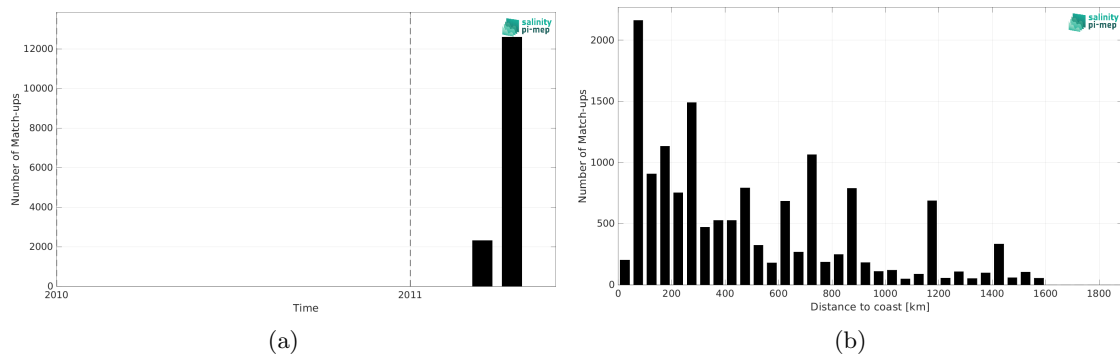
Figure 2: Number of match-ups between TSG (CSIC-UTM) and SMOS SSS L4 v1 - Monthly (CMEMS-CNR) SSS as a function of time (a) and as function of the distance to coast (b) over the South Pacific Ocean Pi-MEP region and for the full satellite product period.
