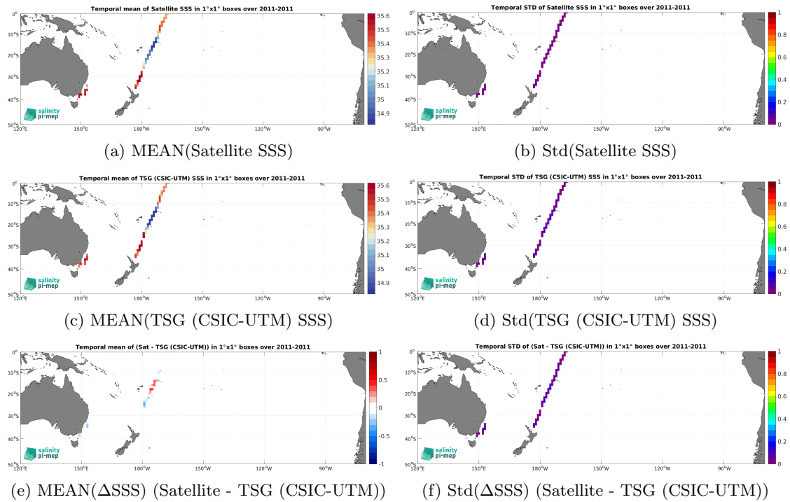
Figure 7: Temporal mean (left) and Std (right) of SSS from SMOS SSS L4 v1 - Monthly (CMEMS-CNR) (top), TSG (CSIC-UTM) (middle), and of \Delta SSS (Satellite - TSG (CSIC-UTM)). Only match-up pairs are used to generate these maps.
