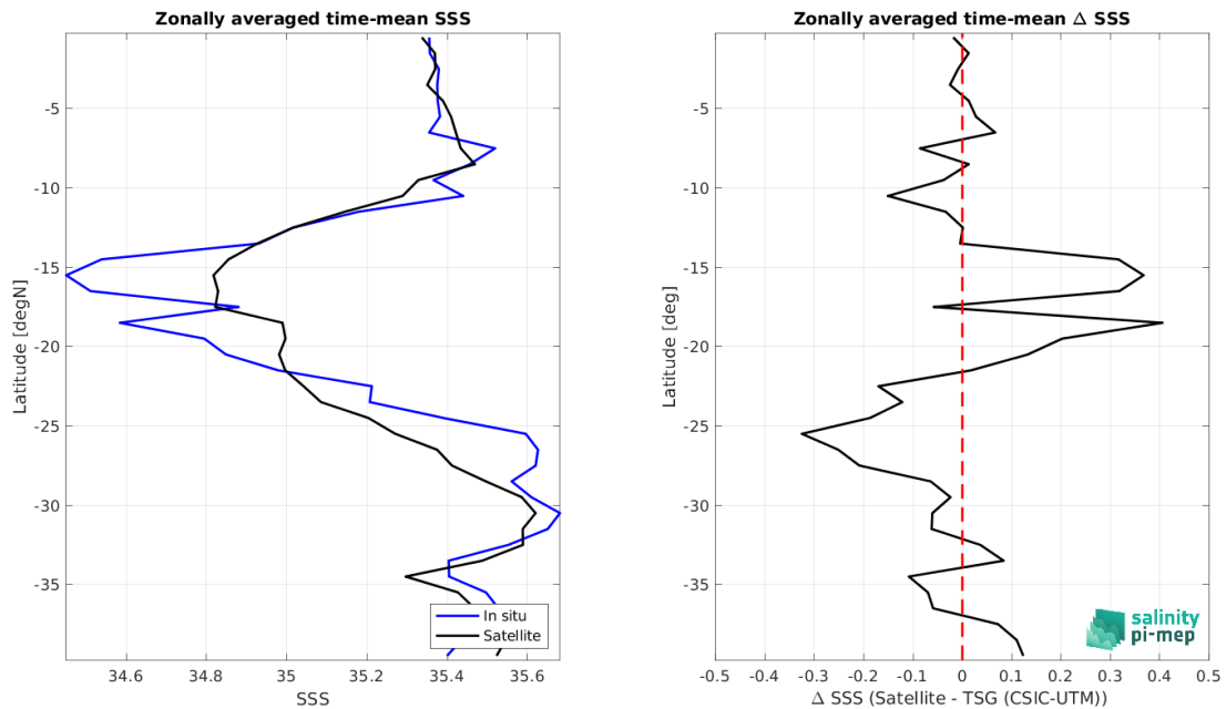
Figure 9: Left panel: Zonal mean SSS from SMOS SSS L4 v1 - Monthly (CMEMS-CNR) satellite product (black) and from TSG (CSIC-UTM) (blue). Right panel: Zonal mean of \Delta SSS (Satellite - TSG (CSIC-UTM)) for all the collected Pi-MEP match-up pairs estimated over the full satellite product period.
