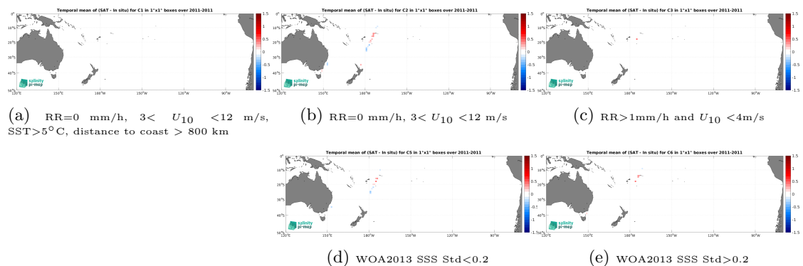
Figure 14: Temporal mean gridded over spatial boxes of size 1^\circ \times 1^\circ of \Delta SSS (SMOS SSS L4 v1 - Monthly (CMEMS-CNR) - TSG (CSIC-UTM)) for 5 different subdatasets corresponding to:RR=0 mm/h, 3 < U_{10} < 12 m/s, SST>5°C, distance to coast > 800 km (a), RR=0 mm/h, 3 < U_{10} < 12 m/s (b), RR>1mm/h and U_{10} < 4 m/s (c), WOA2013 SSS Std<0.2 (d), WOA2013 SSS Std>0.2 (e).
