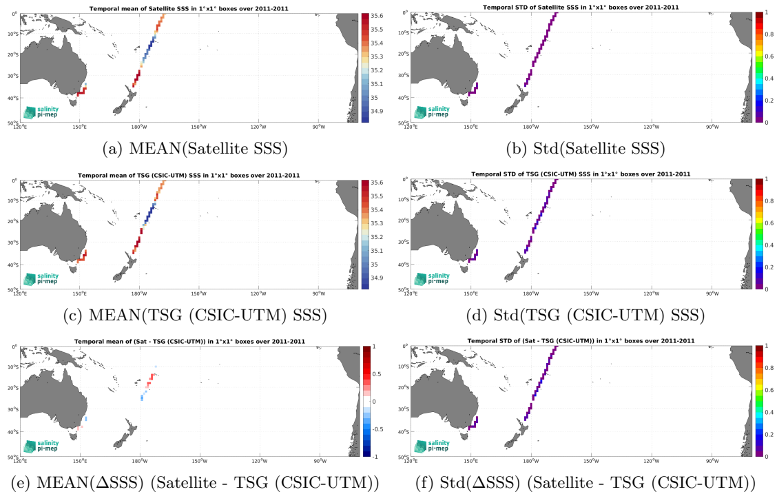
Figure 6: Temporal mean (left) and Std (right) of SSS from SMOS SSS L4 v1 - Monthly (CMEMS-CNR) (top), TSG (CSIC-UTM) (middle), and of \Delta SSS (Satellite - TSG (CSIC-UTM)). Only match-up pairs are used to generate these maps.
