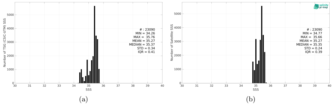
Figure 2: Histograms of SSS from TSG (CSIC-UTM) (a) and SMOS SSS L4 v1 - Monthly (CMEMS-CNR) (b) considering all match-up pairs per bins of 0.1 over the South Pacific Ocean Pi-MEP region and for the full satellite product period.
