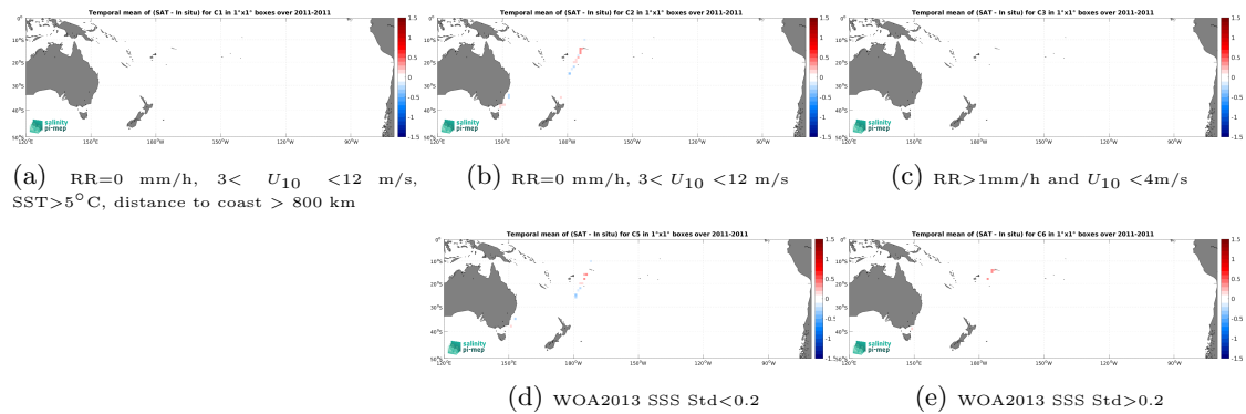
Figure 12: Temporal mean gridded over spatial boxes of size 1^\circ \times 1^\circ of \Delta SSS (SMOS SSS L4 v1 - Monthly (CMEMS-CNR) - TSG (CSIC-UTM)) for 5 different subdatasets corresponding to:RR=0 mm/h, 3 < U_{10} < 12 m/s, SST >5^\circ C, distance to coast > 800 km (a), RR=0 mm/h, 3 < U_{10} < 12 m/s (b), RR >1 mm/h and U_{10} < 4 m/s (c), WOA2013 SSS Std <0.2 (d), WOA2013 SSS Std >0.2 (e).
