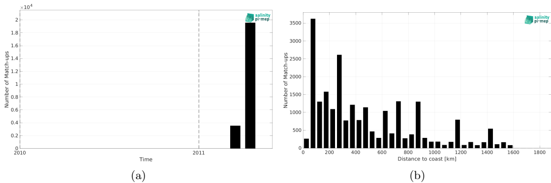
Figure 1: Number of match-ups between TSG (CSIC-UTM) and SMOS SSS L4 v1 - Monthly (CMEMS-CNR) SSS as a function of time (a) and as function of the distance to coast (b) over the South Pacific Ocean Pi-MEP region and for the full satellite product period.
