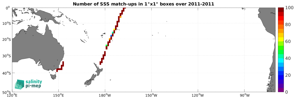
Figure 4: Number of SSS match-ups between TSG (CSIC-UTM) SSS and the SMOS SSS L4 v1 - Monthly (CMEMS-CNR) SSS product for the South Pacific Ocean Pi-MEP region over 1^\circ \times 1^\circ boxes and for the full satellite product period.
