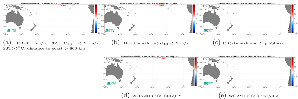
Figure 14: Temporal mean gridded over spatial boxes of size 1^\circ \times 1^\circ of \Delta SSS (SMOS SSS L4 v1 - Monthly (CMEMS-CNR) - Saildrone) for 5 different subdatasets corresponding to:RR=0 mm/h, 3 < U_{10} < 12 m/s, SST >5^\circ\text{C} , distance to coast > 800 km (a), RR=0 mm/h, 3 < U_{10} < 12 m/s (b), RR >1 mm/h and U_{10} < 4 m/s (c), WOA2013 SSS Std <0.2 (d), WOA2013 SSS Std >0.2 (e).
