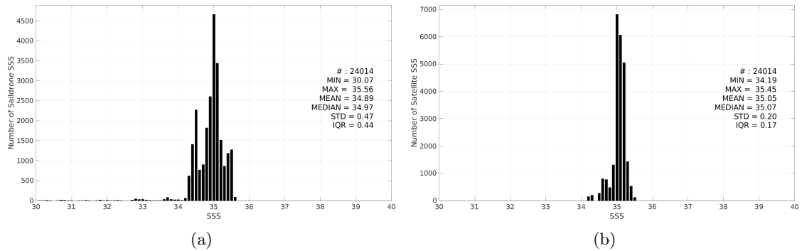
Figure 3: Histograms of SSS from Saildrone (a) and SMOS SSS L4 v1 - Monthly (CMEMS-CNR) (b) considering all match-up pairs per bins of 0.1 over the South Pacific Ocean Pi-MEP region and for the full satellite product period.
