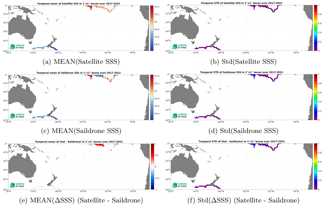
Figure 7: Temporal mean (left) and Std (right) of SSS from SMOS SSS L4 v1 - Monthly (CMEMS-CNR) (top), Saildrone (middle), and of \Delta SSS (Satellite - Saildrone). Only match-up pairs are used to generate these maps.
