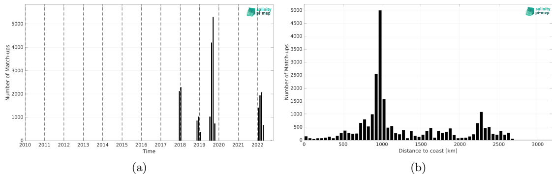
Figure 2: Number of match-ups between Saildrone and SMOS SSS L4 v1 - Monthly (CMEMS-CNR) SSS as a function of time (a) and as function of the distance to coast (b) over the South Pacific Ocean Pi-MEP region and for the full satellite product period.
