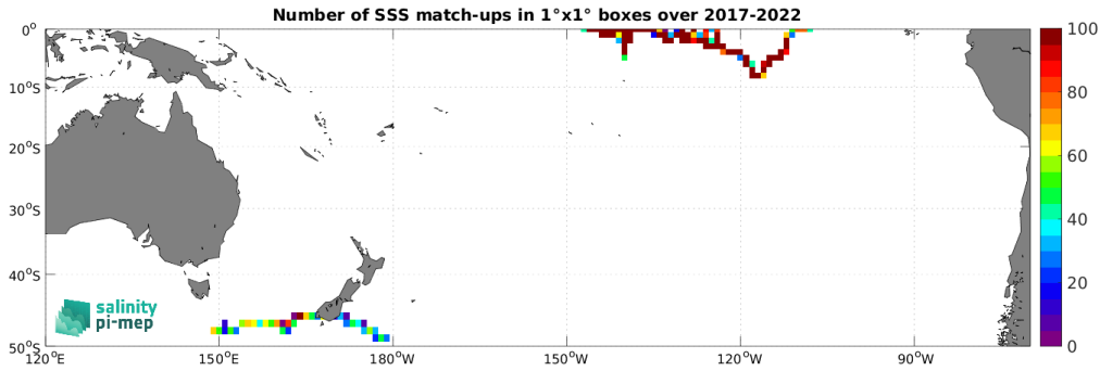
Figure 5: Number of SSS match-ups between Saildrone SSS and the SMOS SSS L4 v1 - Monthly (CMEMS-CNR) SSS product for the South Pacific Ocean Pi-MEP region over 1^\circ \times 1^\circ boxes and for the full satellite product period.
