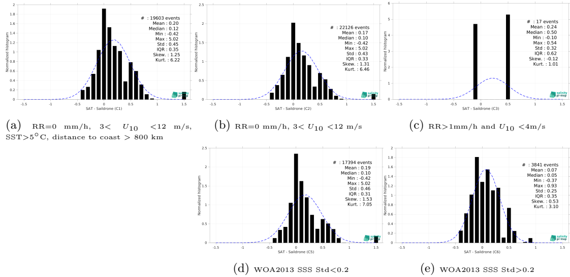
Figure 15: Normalized histogram of \Delta SSS (SMOS SSS L4 v1 - Monthly (CMEMS-CNR) - Saildrone) for 5 different subdatasets corresponding to: RR=0 mm/h, 3 < U_{10} < 12 m/s, SST > 5°C, distance to coast > 800 km (a), RR=0 mm/h, 3 < U_{10} < 12 m/s (b), RR > 1mm/h and U_{10} < 4 m/s (c), WOA2013 SSS Std < 0.2 (d), WOA2013 SSS Std > 0.2 (e).
