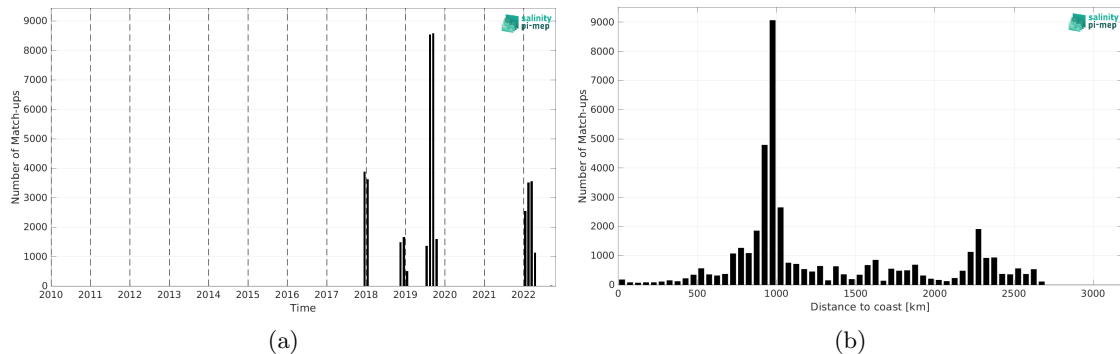
Figure 1: Number of match-ups between Saildrone and SMOS SSS L4 v1 - Monthly (CMEMS-CNR) SSS as a function of time (a) and as function of the distance to coast (b) over the South Pacific Ocean Pi-MEP region and for the full satellite product period.
