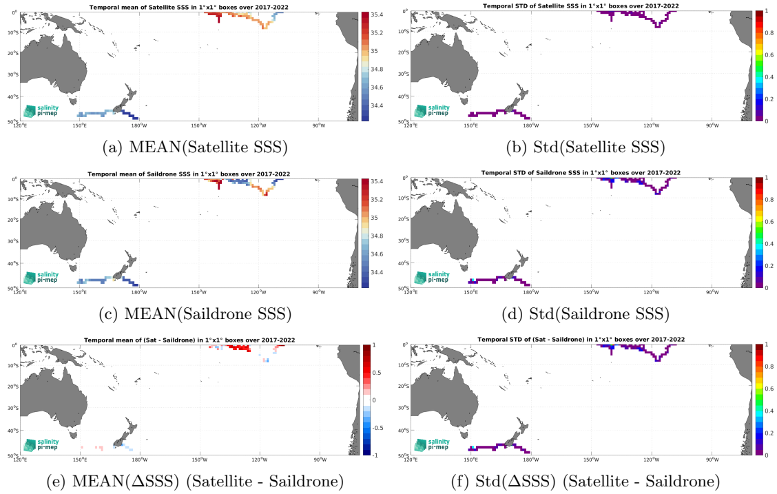
Figure 6: Temporal mean (left) and Std (right) of SSS from SMOS SSS L4 v1 - Monthly (CMEMS-CNR) (top), Saildrone (middle), and of \Delta SSS (Satellite - Saildrone). Only match-up pairs are used to generate these maps.
