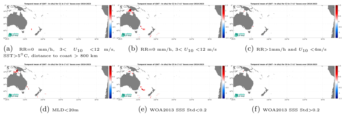
Figure 14: Temporal mean gridded over spatial boxes of size 1^\circ \times 1^\circ of \Delta SSS (SMOS SSS L4 v1 - Monthly (CMEMS-CNR) - Marine mammals) for 6 different subdatasets corresponding to:RR=0 mm/h, 3 < U_{10} < 12 m/s, SST >5^\circ C, distance to coast > 800 km (a), RR=0 mm/h, 3 < U_{10} < 12 m/s (b), RR >1 mm/h and U_{10} < 4 m/s (c),MLD <20 m (d),WOA2013 SSS Std <0.2 (e),WOA2013 SSS Std >0.2 (f).
