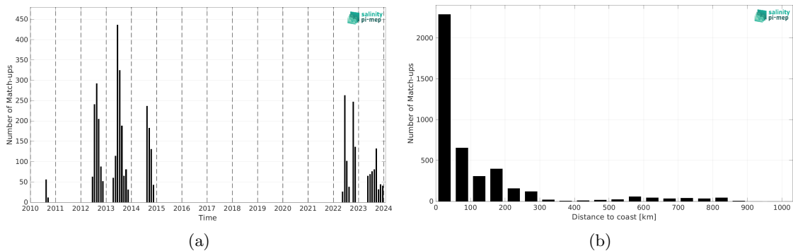
Figure 2: Number of match-ups between Marine mammals and SMOS SSS L4 v1 - Monthly (CMEMS-CNR) SSS as a function of time (a) and as function of the distance to coast (b) over the South Pacific Ocean Pi-MEP region and for the full satellite product period.
