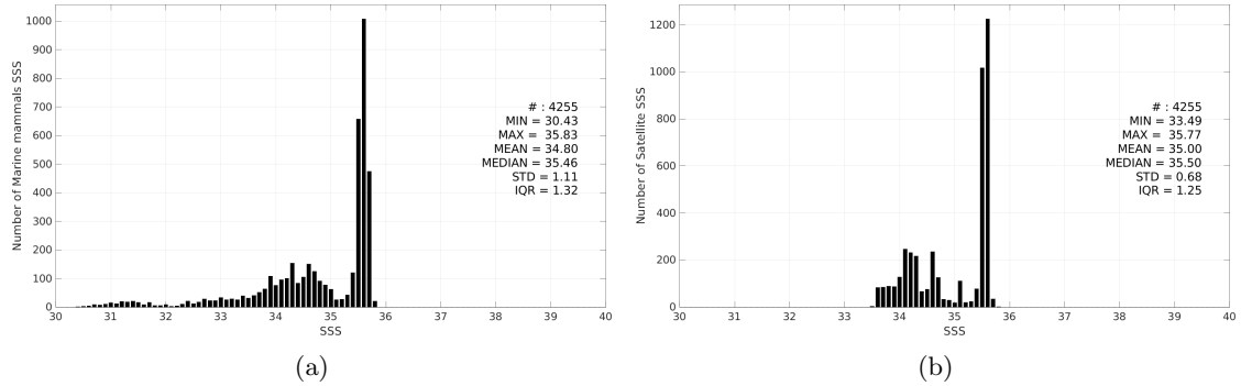
Figure 3: Histograms of SSS from Marine mammals (a) and SMOS SSS L4 v1 - Monthly (CMEMS-CNR) (b) considering all match-up pairs per bins of 0.1 over the South Pacific Ocean Pi-MEP region and for the full satellite product period.
