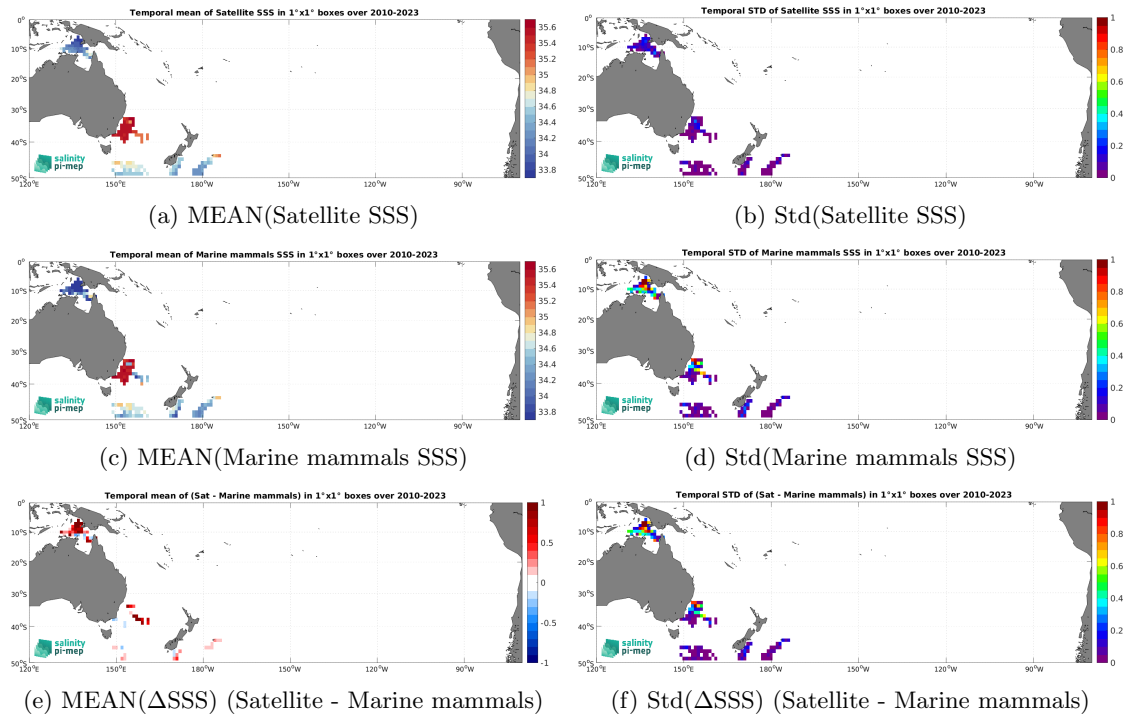
Figure 7: Temporal mean (left) and Std (right) of SSS from SMOS SSS L4 v1 - Monthly (CMEMS-CNR) (top), Marine mammals (middle), and of \Delta SSS (Satellite - Marine mammals). Only match-up pairs are used to generate these maps.
