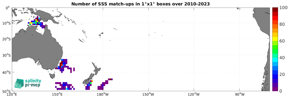
Figure 5: Number of SSS match-ups between Marine mammals SSS and the SMOS SSS L4 v1 - Monthly (CMEMS-CNR) SSS product for the South Pacific Ocean Pi-MEP region over 1^\circ \times 1^\circ boxes and for the full satellite product period.
