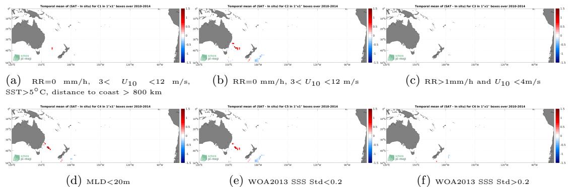
Figure 12: Temporal mean gridded over spatial boxes of size 1^\circ \times 1^\circ of \Delta SSS (SMOS SSS L4 v1 - Monthly (CMEMS-CNR) - Marine mammals) for 6 different subdatasets corresponding to:RR=0 mm/h, 3 < U_{10} < 12 m/s, SST >5^\circ C, distance to coast > 800 km (a), RR=0 mm/h, 3 < U_{10} < 12 m/s (b), RR >1 mm/h and U_{10} < 4 m/s (c),MLD <20 m (d),WOA2013 SSS Std <0.2 (e),WOA2013 SSS Std >0.2 (f).
