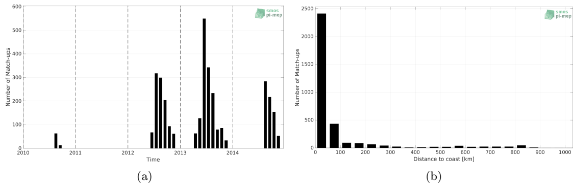
Figure 1: Number of match-ups between Marine mammals and SMOS SSS L4 v1 - Monthly (CMEMS-CNR) SSS as a function of time (a) and as function of the distance to coast (b) over the South Pacific Ocean Pi-MEP region and for the full satellite product period.
