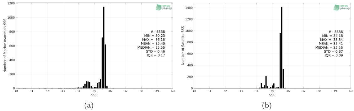
Figure 2: Histograms of SSS from Marine mammals (a) and SMOS SSS L4 v1 - Monthly (CMEMS-CNR) (b) considering all match-up pairs per bins of 0.1 over the South Pacific Ocean Pi-MEP region and for the full satellite product period.
