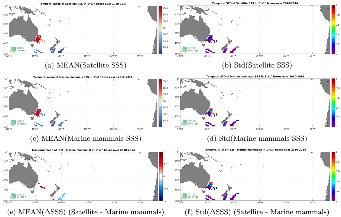
Figure 6: Temporal mean (left) and Std (right) of SSS from SMOS SSS L4 v1 - Monthly (CMEMS-CNR) (top), Marine mammals (middle), and of \Delta SSS (Satellite - Marine mammals). Only match-up pairs are used to generate these maps.
