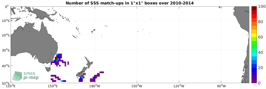
Figure 4: Number of SSS match-ups between Marine mammals SSS and the SMOS SSS L4 v1 - Monthly (CMEMS-CNR) SSS product for the South Pacific Ocean Pi-MEP region over 1^\circ \times 1^\circ boxes and for the full satellite product period.
