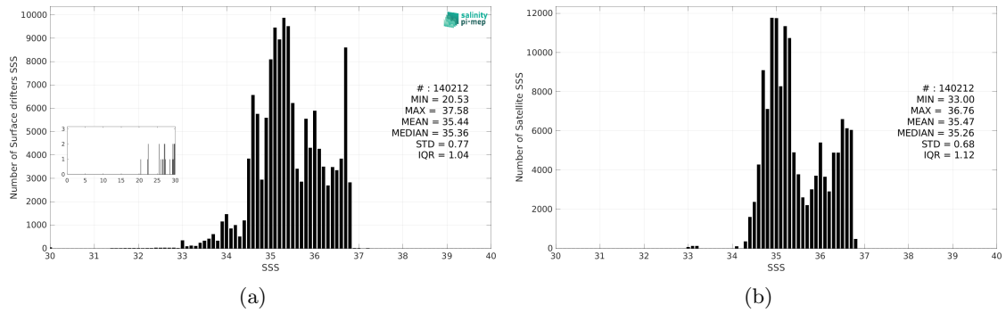
Figure 3: Histograms of SSS from Surface drifters (a) and SMOS SSS L4 v1 - Monthly (CMEMS-CNR) (b) considering all match-up pairs per bins of 0.1 over the South Pacific Ocean Pi-MEP region and for the full satellite product period.
