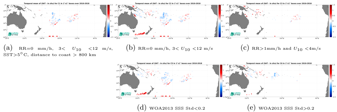
Figure 13: Temporal mean gridded over spatial boxes of size 1^\circ \times 1^\circ of \Delta SSS (SMOS SSS L4 v1 - Monthly (CMEMS-CNR) - Surface drifters) for 5 different subdatasets corresponding to:RR=0 mm/h, 3 < U_{10} < 12 m/s, SST >5^\circ\text{C} , distance to coast > 800 km (a), RR=0 mm/h, 3 < U_{10} < 12 m/s (b), RR >1 mm/h and U_{10} < 4 m/s (c), WOA2013 SSS Std <0.2 (d), WOA2013 SSS Std >0.2 (e).
