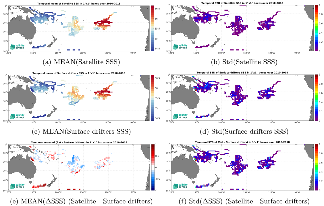
Figure 6: Temporal mean (left) and Std (right) of SSS from SMOS SSS L4 v1 - Monthly (CMEMS-CNR) (top), Surface drifters (middle), and of \Delta SSS (Satellite - Surface drifters). Only match-up pairs are used to generate these maps.
