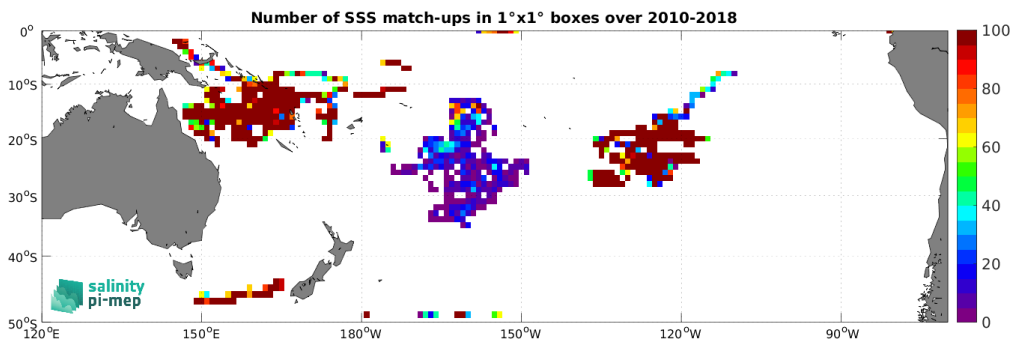
Figure 4: Number of SSS match-ups between Surface drifters SSS and the SMOS SSS L4 v1 - Monthly (CMEMS-CNR) SSS product for the South Pacific Ocean Pi-MEP region over 1^\circ \times 1^\circ boxes and for the full satellite product period.
