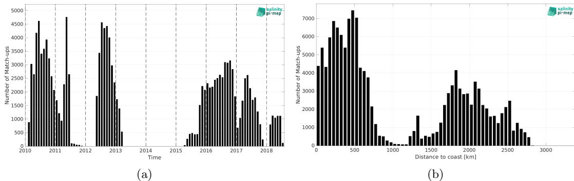
Figure 2: Number of match-ups between Surface drifters and SMOS SSS L4 v1 - Monthly (CMEMS-CNR) SSS as a function of time (a) and as function of the distance to coast (b) over the South Pacific Ocean Pi-MEP region and for the full satellite product period.
