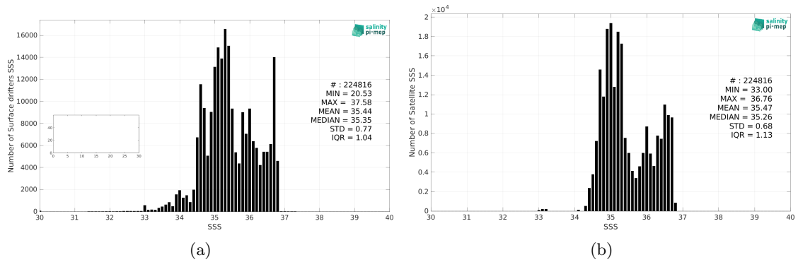
Figure 2: Histograms of SSS from Surface drifters (a) and SMOS SSS L4 v1 - Monthly (CMEMS-CNR) (b) considering all match-up pairs per bins of 0.1 over the South Pacific Ocean Pi-MEP region and for the full satellite product period.
