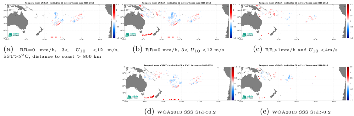
Figure 11: Temporal mean gridded over spatial boxes of size 1^\circ \times 1^\circ of \Delta\text{SSS} (SMOS SSS L4 v1 - Monthly (CMEMS-CNR) - Surface drifters) for 5 different subdatasets corresponding to:RR=0 mm/h, 3 < U_{10} < 12 m/s, SST >5^\circ\text{C} , distance to coast > 800 km (a), RR=0 mm/h, 3 < U_{10} < 12 m/s (b), RR >1 mm/h and U_{10} < 4 m/s (c), WOA2013 SSS Std <0.2 (d), WOA2013 SSS Std >0.2 (e).
