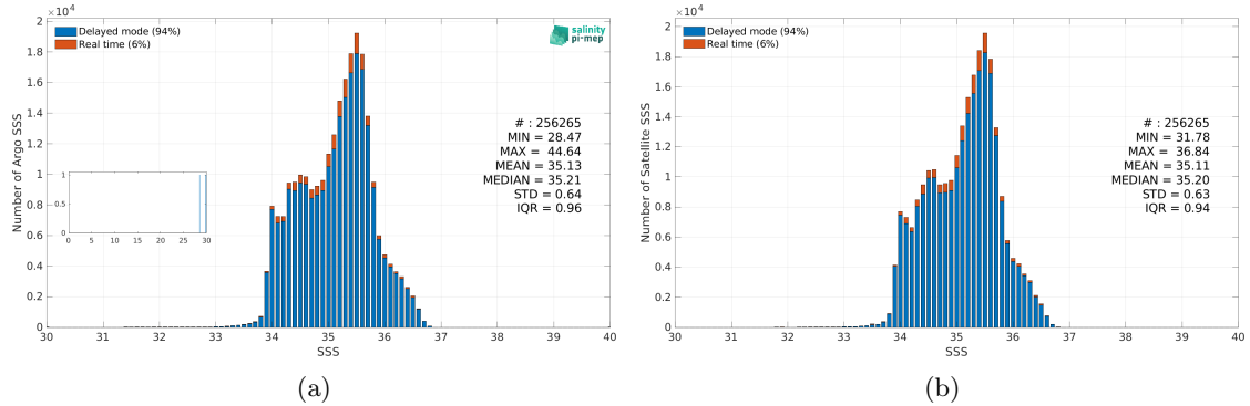
Figure 3: Histograms of SSS from Argo (a) and SMOS SSS L4 v1 - Monthly (CMEMS-CNR) (b) considering all match-up pairs per bins of 0.1 over the South Pacific Ocean Pi-MEP region and for the full satellite product period.
