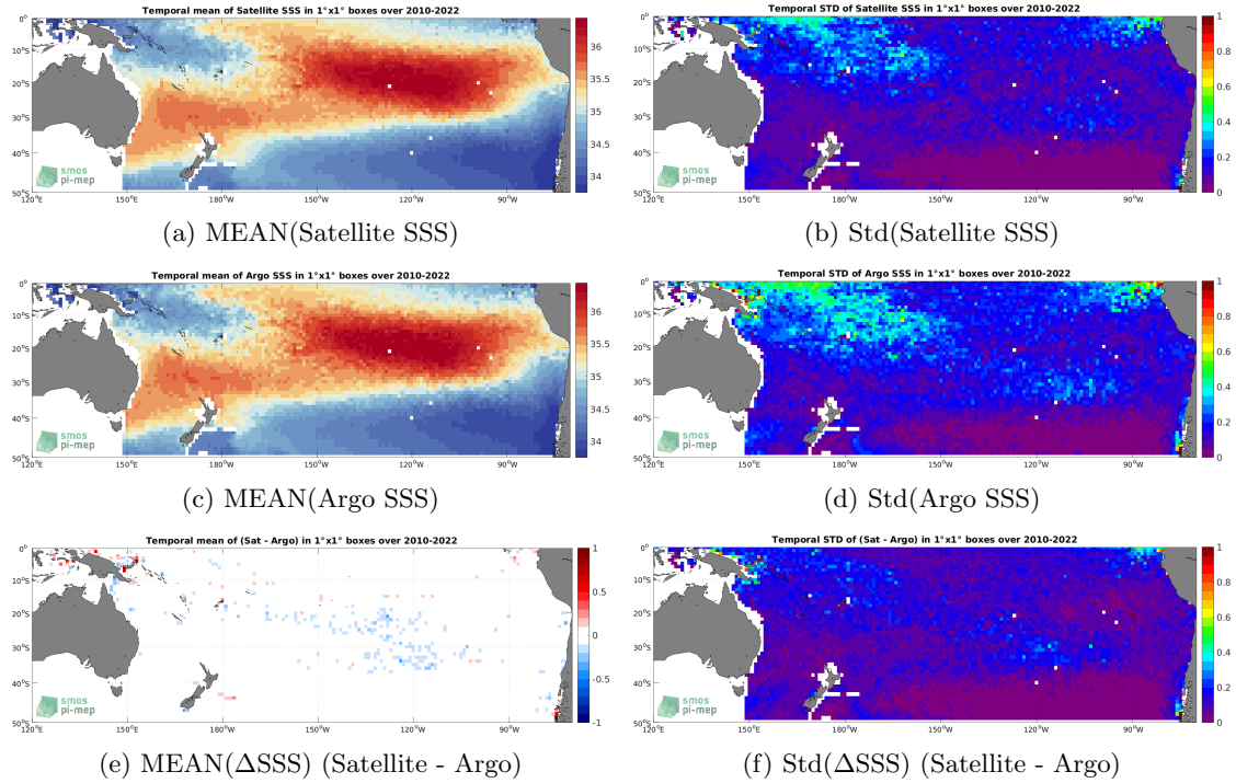
Figure 6: Temporal mean (left) and Std (right) of SSS from SMOS SSS L4 v1 - Monthly (CMEMS-CNR) (top), Argo (middle), and of \Delta SSS (Satellite - Argo). Only match-up pairs are used to generate these maps.
