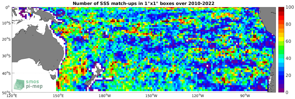
Figure 4: Number of SSS match-ups between Argo SSS and the SMOS SSS L4 v1 - Monthly (CMEMS-CNR) SSS product for the South Pacific Ocean Pi-MEP region over 1^\circ \times 1^\circ boxes and for the full satellite product period.
