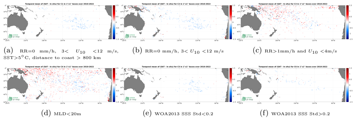
Figure 12: Temporal mean gridded over spatial boxes of size 1^\circ \times 1^\circ of \Delta SSS (SMOS SSS L4 v1 - Monthly (CMEMS-CNR) - Argo) for 6 different subdatasets corresponding to:RR=0 mm/h, 3 < U_{10} < 12 m/s, SST >5^\circ C, distance to coast > 800 km (a), RR=0 mm/h, 3 < U_{10} < 12 m/s (b), RR >1 mm/h and U_{10} < 4 m/s (c),MLD <20 m (d),WOA2013 SSS Std <0.2 (e),WOA2013 SSS Std >0.2 (f).
