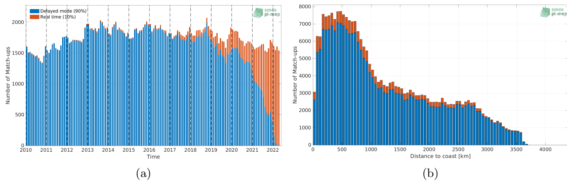
Figure 1: Number of match-ups between Argo and SMOS SSS L4 v1 - Monthly (CMEMS-CNR) SSS as a function of time (a) and as function of the distance to coast (b) over the South Pacific Ocean Pi-MEP region and for the full satellite product period.
