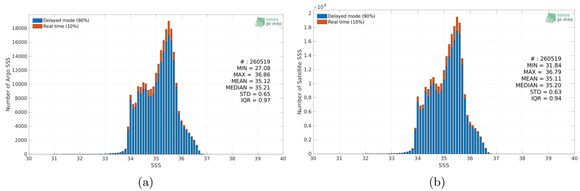
Figure 2: Histograms of SSS from Argo (a) and SMOS SSS L4 v1 - Monthly (CMEMS-CNR) (b) considering all match-up pairs per bins of 0.1 over the South Pacific Ocean Pi-MEP region and for the full satellite product period.
