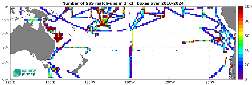
Figure 5: Number of SSS match-ups between TSG (SAMOS) SSS and the SMOS SSS L4 v1 - Daily (CMEMS-CNR) SSS product for the South Pacific Ocean Pi-MEP region over 1^\circ \times 1^\circ boxes and for the full satellite product period.
