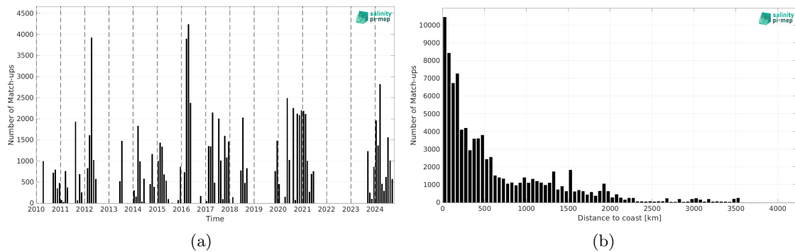
Figure 2: Number of match-ups between TSG (SAMOS) and SMOS SSS L4 v1 - Daily (CMEMS-CNR) SSS as a function of time (a) and as function of the distance to coast (b) over the South Pacific Ocean Pi-MEP region and for the full satellite product period.
