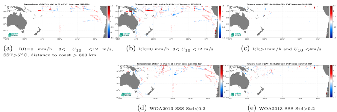
Figure 14: Temporal mean gridded over spatial boxes of size 1^\circ \times 1^\circ of \Delta\text{SSS} (SMOS SSS L4 v1 - Daily (CMEMS-CNR) - TSG (SAMOS)) for 5 different subdatasets corresponding to:RR=0 mm/h, 3 < U_{10} < 12 m/s, SST>5°C, distance to coast > 800 km (a), RR=0 mm/h, 3 < U_{10} < 12 m/s (b), RR>1mm/h and U_{10} < 4 m/s (c), WOA2013 SSS Std<0.2 (d), WOA2013 SSS Std>0.2 (e).
