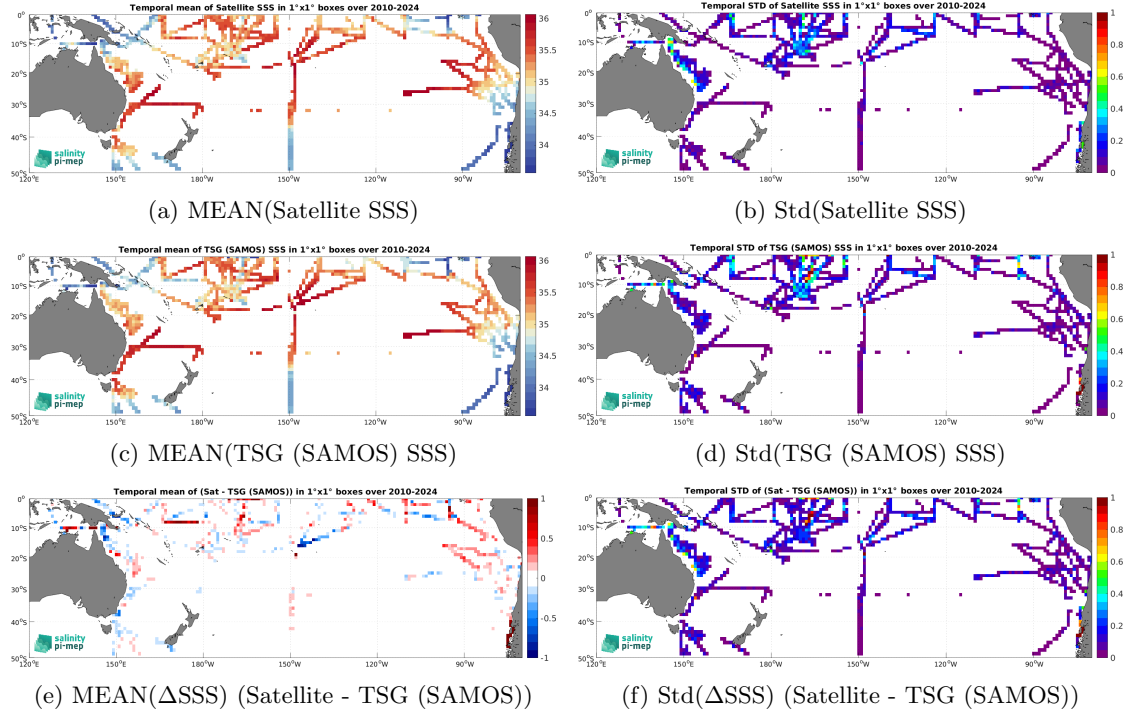
Figure 7: Temporal mean (left) and Std (right) of SSS from SMOS SSS L4 v1 - Daily (CMEMS-CNR) (top), TSG (SAMOS) (middle), and of \Delta SSS (Satellite - TSG (SAMOS)). Only match-up pairs are used to generate these maps.
