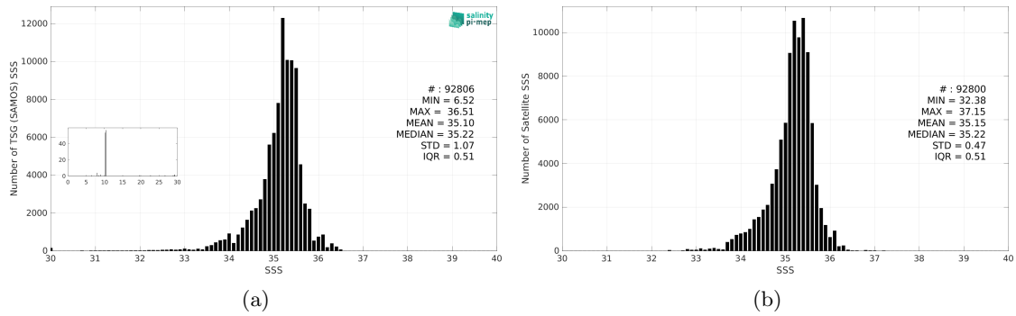
Figure 3: Histograms of SSS from TSG (SAMOS) (a) and SMOS SSS L4 v1 - Daily (CMEMS-CNR) (b) considering all match-up pairs per bins of 0.1 over the South Pacific Ocean Pi-MEP region and for the full satellite product period.
