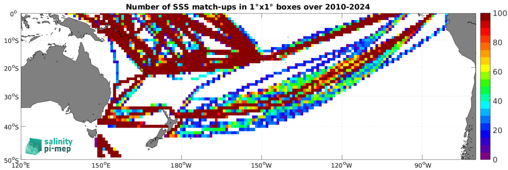
Figure 5: Number of SSS match-ups between TSG (LEGOS-DM) SSS and the SMOS SSS L4 v1 - Daily (CMEMS-CNR) SSS product for the South Pacific Ocean Pi-MEP region over 1^\circ \times 1^\circ boxes and for the full satellite product period.
