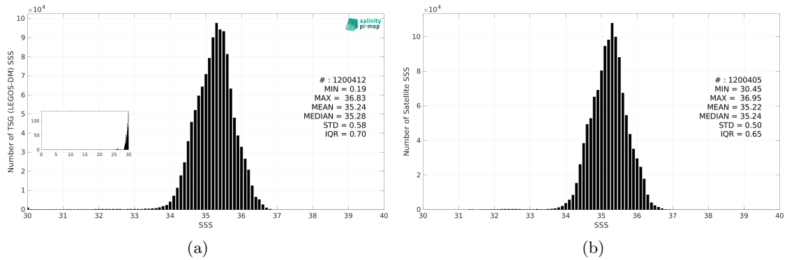
Figure 3: Histograms of SSS from TSG (LEGOS-DM) (a) and SMOS SSS L4 v1 - Daily (CMEMS-CNR) (b) considering all match-up pairs per bins of 0.1 over the South Pacific Ocean Pi-MEP region and for the full satellite product period.
