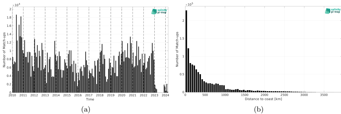
Figure 2: Number of match-ups between TSG (LEGOS-DM) and SMOS SSS L4 v1 - Daily (CMEMS-CNR) SSS as a function of time (a) and as function of the distance to coast (b) over the South Pacific Ocean Pi-MEP region and for the full satellite product period.
