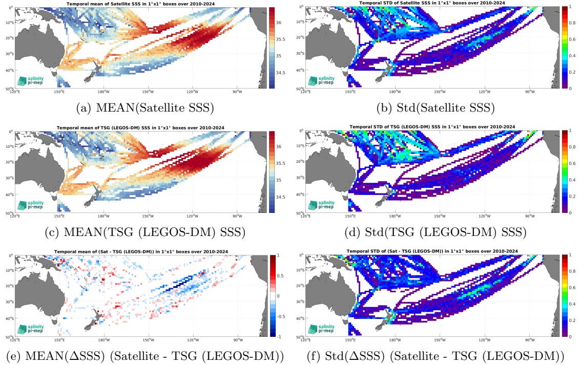
Figure 7: Temporal mean (left) and Std (right) of SSS from SMOS SSS L4 v1 - Daily (CMEMS-CNR) (top), TSG (LEGOS-DM) (middle), and of \Delta SSS (Satellite - TSG (LEGOS-DM)). Only match-up pairs are used to generate these maps.
