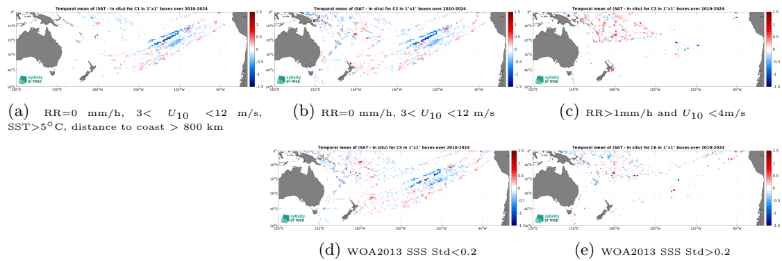
Figure 14: Temporal mean gridded over spatial boxes of size 1^\circ \times 1^\circ of \Delta\text{SSS} (SMOS SSS L4 v1 - Daily (CMEMS-CNR) - TSG (LEGOS-DM)) for 5 different subdatasets corresponding to:RR=0 mm/h, 3 < U_{10} < 12 m/s, SST>5°C, distance to coast > 800 km (a), RR=0 mm/h, 3 < U_{10} < 12 m/s (b), RR>1mm/h and U_{10} < 4 m/s (c), WOA2013 SSS Std<0.2 (d), WOA2013 SSS Std>0.2 (e).
