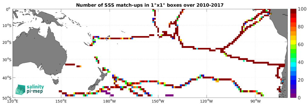
Figure 5: Number of SSS match-ups between TSG (GOSUD-Sailing-ship) SSS and the SMOS SSS L4 v1 - Daily (CMEMS-CNR) SSS product for the South Pacific Ocean Pi-MEP region over 1^\circ \times 1^\circ boxes and for the full satellite product period.
