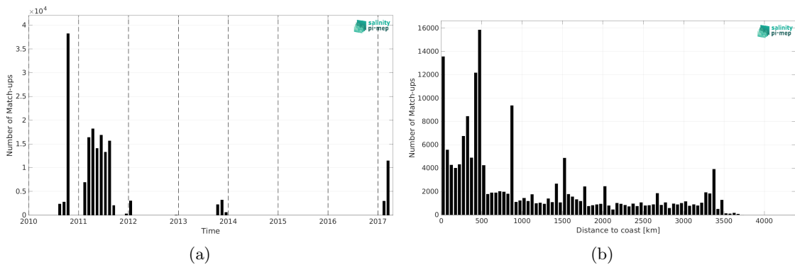
Figure 2: Number of match-ups between TSG (GOSUD-Sailing-ship) and SMOS SSS L4 v1 - Daily (CMEMS-CNR) SSS as a function of time (a) and as function of the distance to coast (b) over the South Pacific Ocean Pi-MEP region and for the full satellite product period.
