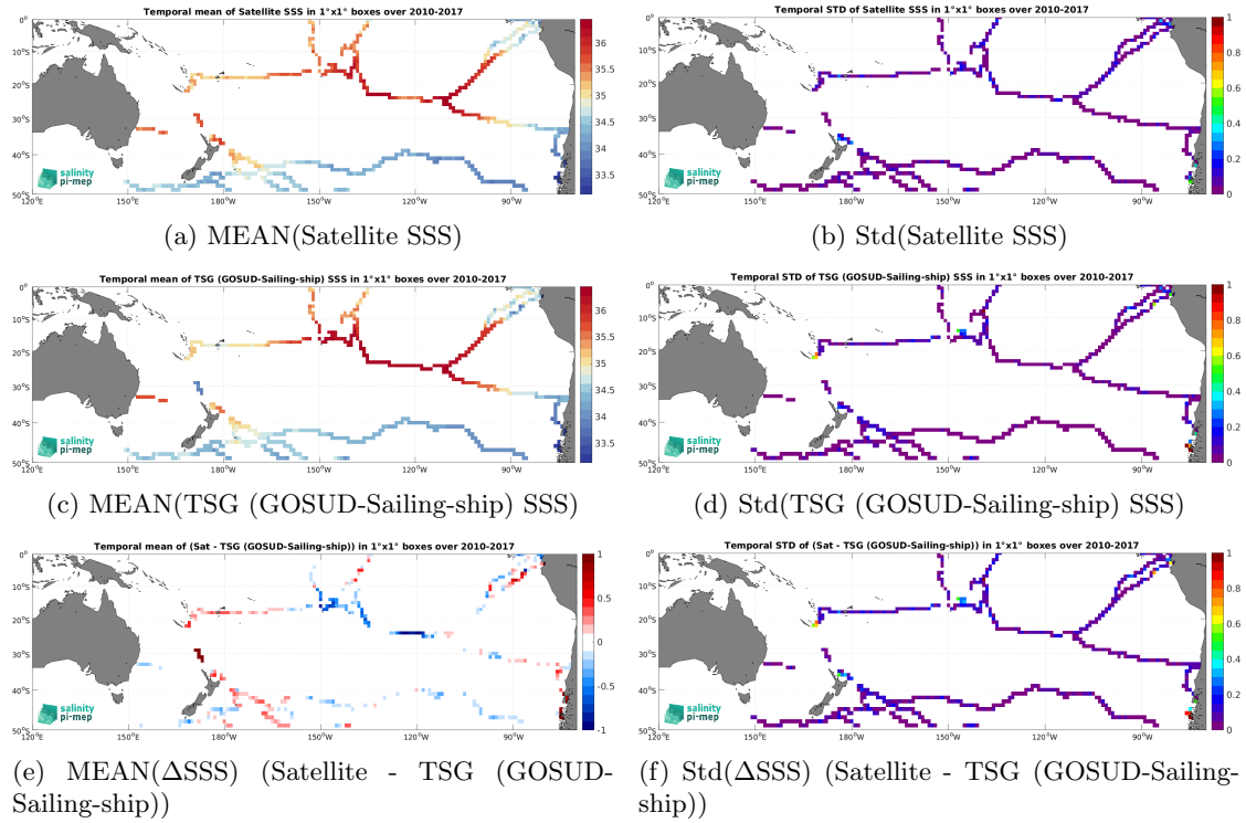
Figure 7: Temporal mean (left) and Std (right) of SSS from SMOS SSS L4 v1 - Daily (CMEMS-CNR) (top), TSG (GOSUD-Sailing-ship) (middle), and of \Delta SSS (Satellite - TSG (GOSUD-Sailing-ship)). Only match-up pairs are used to generate these maps.
