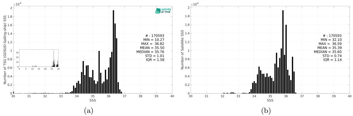
Figure 3: Histograms of SSS from TSG (GOSUD-Sailing-ship) (a) and SMOS SSS L4 v1 - Daily (CMEMS-CNR) (b) considering all match-up pairs per bins of 0.1 over the South Pacific Ocean Pi-MEP region and for the full satellite product period.
