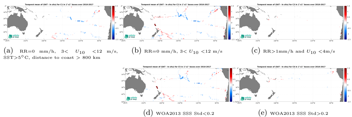
Figure 14: Temporal mean gridded over spatial boxes of size 1^\circ \times 1^\circ of \Delta SSS (SMOS SSS L4 v1 - Daily (CMEMS-CNR) - TSG (GOSUD-Sailing-ship)) for 5 different subdatasets corresponding to:RR=0 mm/h, 3 < U_{10} < 12 m/s, SST >5^\circ\text{C} , distance to coast > 800 km (a), RR=0 mm/h, 3 < U_{10} < 12 m/s (b), RR >1 mm/h and U_{10} < 4 m/s (c), WOA2013 SSS Std <0.2 (d), WOA2013 SSS Std >0.2 (e).
