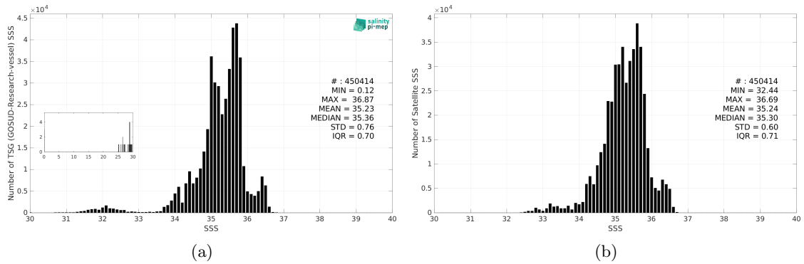
Figure 3: Histograms of SSS from TSG (GOSUD-Research-vessel) (a) and SMOS SSS L4 v1 - Daily (CMEMS-CNR) (b) considering all match-up pairs per bins of 0.1 over the South Pacific Ocean Pi-MEP region and for the full satellite product period.
