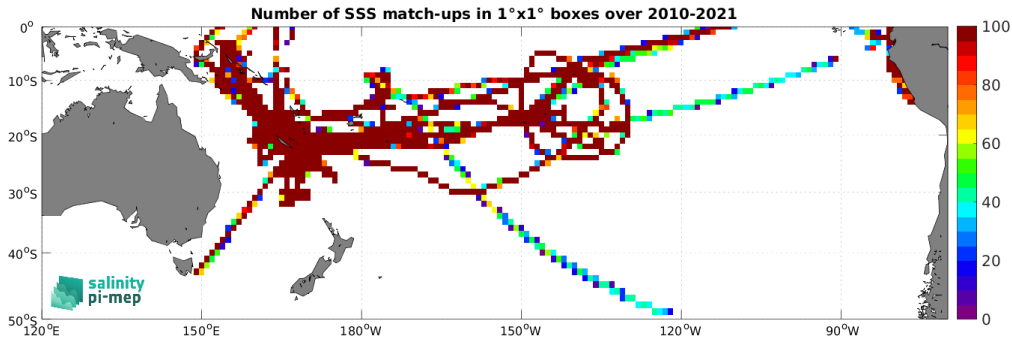
Figure 5: Number of SSS match-ups between TSG (GOSUD-Research-vessel) SSS and the SMOS SSS L4 v1 - Daily (CMEMS-CNR) SSS product for the South Pacific Ocean Pi-MEP region over 1^\circ \times 1^\circ boxes and for the full satellite product period.
