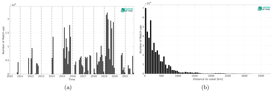
Figure 2: Number of match-ups between TSG (GOSUD-Research-vessel) and SMOS SSS L4 v1 - Daily (CMEMS-CNR) SSS as a function of time (a) and as function of the distance to coast (b) over the South Pacific Ocean Pi-MEP region and for the full satellite product period.
