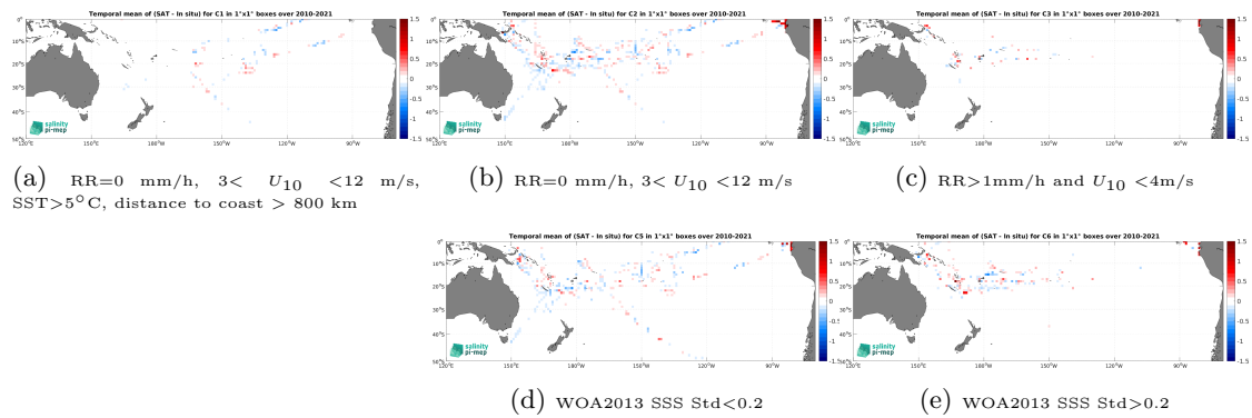
Figure 14: Temporal mean gridded over spatial boxes of size 1^\circ \times 1^\circ of \Delta SSS (SMOS SSS L4 v1 - Daily (CMEMS-CNR) - TSG (GOSUD-Research-vessel)) for 5 different subdatasets corresponding to:RR=0 mm/h, 3 < U_{10} < 12 m/s, SST>5°C, distance to coast > 800 km (a), RR=0 mm/h, 3 < U_{10} < 12 m/s (b), RR>1mm/h and U_{10} < 4 m/s (c), WOA2013 SSS Std<0.2 (d), WOA2013 SSS Std>0.2 (e).
