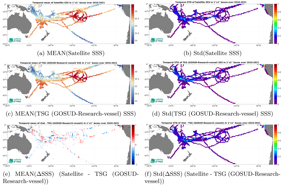
Figure 7: Temporal mean (left) and Std (right) of SSS from SMOS SSS L4 v1 - Daily (CMEMS-CNR) (top), TSG (GOSUD-Research-vessel) (middle), and of \Delta SSS (Satellite - TSG (GOSUD-Research-vessel)). Only match-up pairs are used to generate these maps.
