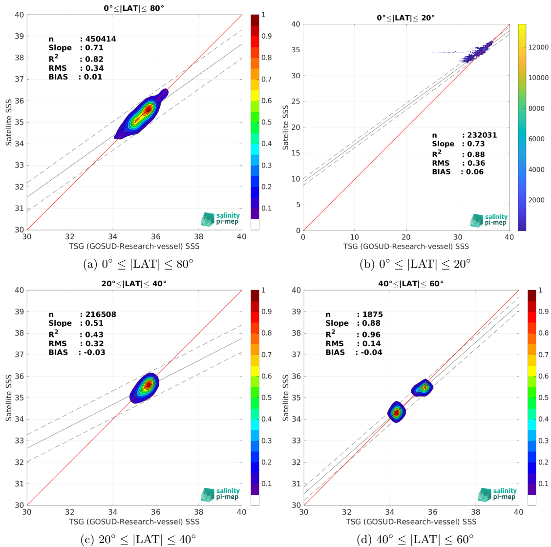
Figure 10: Contour maps of the concentration of SMOS SSS L4 v1 - Daily (CMEMS-CNR) SSS (y-axis) versus TSG (GOSUD-Research-vessel) SSS (x-axis) at match-up pairs for different latitude bands. For each plot, the red line shows x=y . The black thin and dashed lines indicate a linear fit through the data cloud and the \pm 95\% confidence levels, respectively. The number match-up pairs n , the slope and R^2 coefficient of the linear fit, the root mean square (RMS) and the mean bias between satellite and in situ data are indicated for each latitude band in each plots.
