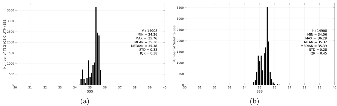
Figure 3: Histograms of SSS from TSG (CSIC-UTM) (a) and SMOS SSS L4 v1 - Daily (CMEMS-CNR) (b) considering all match-up pairs per bins of 0.1 over the South Pacific Ocean Pi-MEP region and for the full satellite product period.
