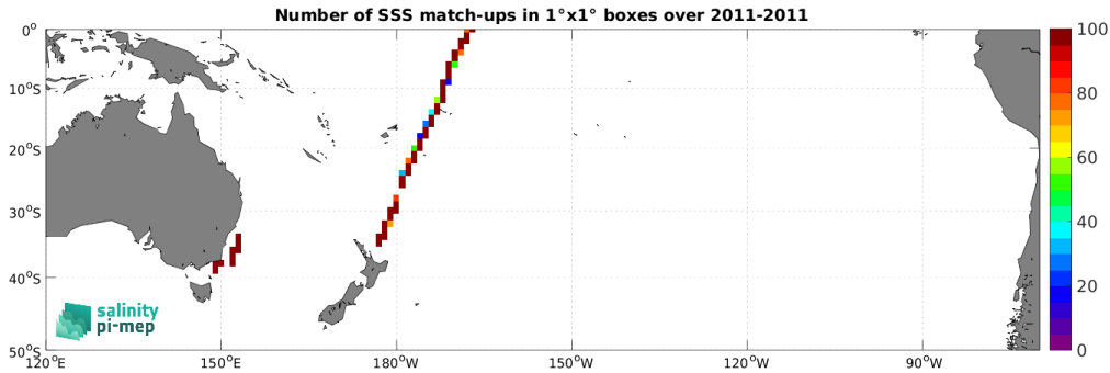
Figure 5: Number of SSS match-ups between TSG (CSIC-UTM) SSS and the SMOS SSS L4 v1 - Daily (CMEMS-CNR) SSS product for the South Pacific Ocean Pi-MEP region over 1^\circ \times 1^\circ boxes and for the full satellite product period.
