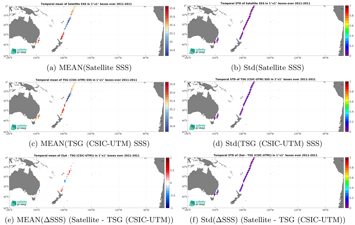
Figure 7: Temporal mean (left) and Std (right) of SSS from SMOS SSS L4 v1 - Daily (CMEMS-CNR) (top), TSG (CSIC-UTM) (middle), and of \Delta SSS (Satellite - TSG (CSIC-UTM)). Only match-up pairs are used to generate these maps.
