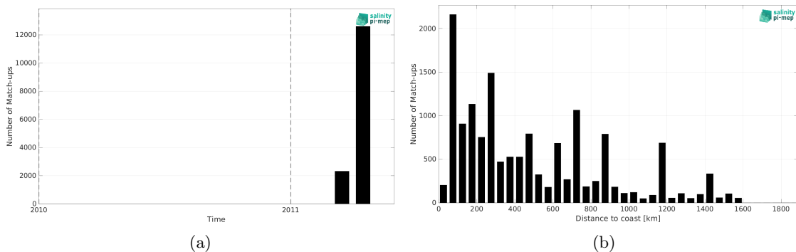
Figure 2: Number of match-ups between TSG (CSIC-UTM) and SMOS SSS L4 v1 - Daily (CMEMS-CNR) SSS as a function of time (a) and as function of the distance to coast (b) over the South Pacific Ocean Pi-MEP region and for the full satellite product period.
