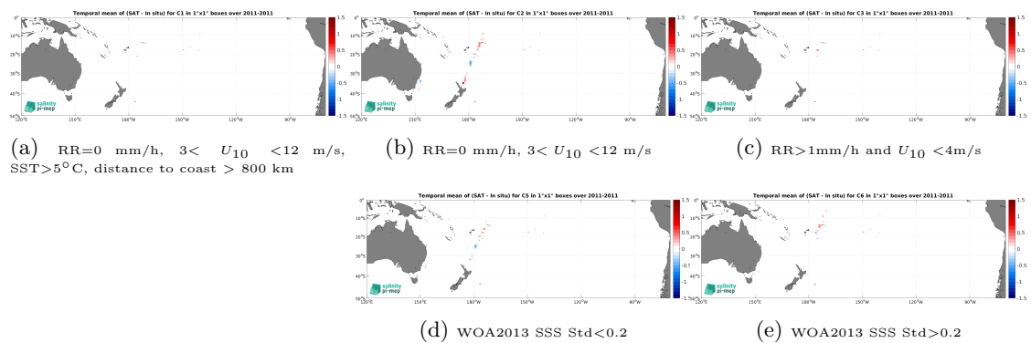
Figure 14: Temporal mean gridded over spatial boxes of size 1^\circ \times 1^\circ of \Delta SSS (SMOS SSS L4 v1 - Daily (CMEMS-CNR) - TSG (CSIC-UTM)) for 5 different subdatasets corresponding to:RR=0 mm/h, 3 < U_{10} < 12 m/s, SST > 5°C, distance to coast > 800 km (a), RR=0 mm/h, 3 < U_{10} < 12 m/s (b), RR > 1mm/h and U_{10} < 4 m/s (c), WOA2013 SSS Std < 0.2 (d), WOA2013 SSS Std > 0.2 (e).
