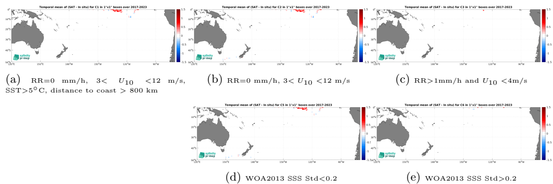
Figure 14: Temporal mean gridded over spatial boxes of size 1^\circ \times 1^\circ of \Delta\text{SSS} (SMOS SSS L4 v1 - Daily (CMEMS-CNR) - Sairdrone) for 5 different subdatasets corresponding to:RR=0 mm/h, 3 < U_{10} < 12 m/s, SST >5^\circ\text{C} , distance to coast > 800 km (a), RR=0 mm/h, 3 < U_{10} < 12 m/s (b), RR >1 mm/h and U_{10} < 4 m/s (c), WOA2013 SSS Std <0.2 (d), WOA2013 SSS Std >0.2 (e).
