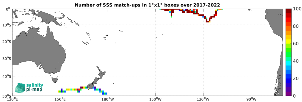
Figure 5: Number of SSS match-ups between Saildrone SSS and the SMOS SSS L4 v1 - Daily (CMEMS-CNR) SSS product for the South Pacific Ocean Pi-MEP region over 1^\circ \times 1^\circ boxes and for the full satellite product period.
