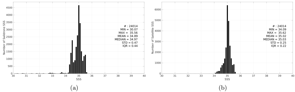
Figure 3: Histograms of SSS from Saildrone (a) and SMOS SSS L4 v1 - Daily (CMEMS-CNR) (b) considering all match-up pairs per bins of 0.1 over the South Pacific Ocean Pi-MEP region and for the full satellite product period.
