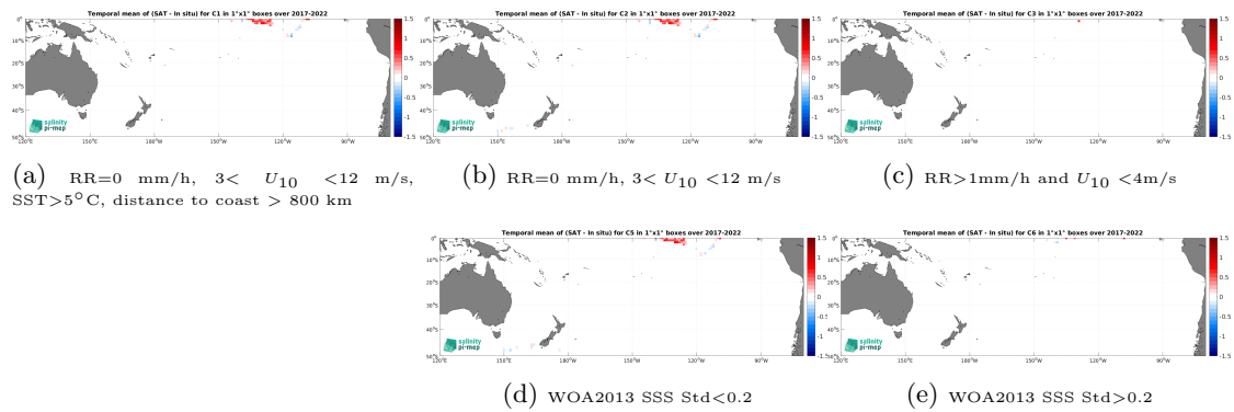
Figure 14: Temporal mean gridded over spatial boxes of size 1^\circ \times 1^\circ of \Delta SSS (SMOS SSS L4 v1 - Daily (CMEMS-CNR) - Sairdrone) for 5 different subdatasets corresponding to:RR=0 mm/h, 3 < U_{10} < 12 m/s, SST >5^\circ\text{C} , distance to coast > 800 km (a), RR=0 mm/h, 3 < U_{10} < 12 m/s (b), RR >1 mm/h and U_{10} < 4 m/s (c), WOA2013 SSS Std <0.2 (d), WOA2013 SSS Std >0.2 (e).
