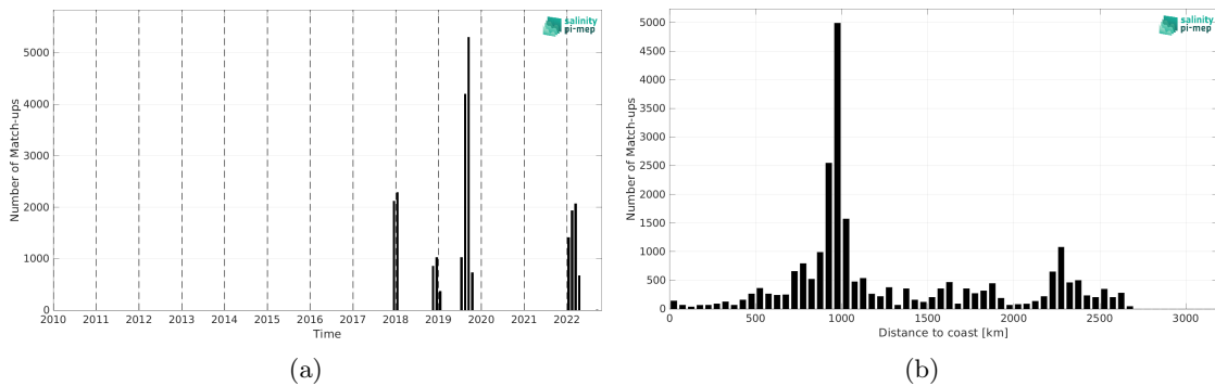
Figure 2: Number of match-ups between Saildrone and SMOS SSS L4 v1 - Daily (CMEMS-CNR) SSS as a function of time (a) and as function of the distance to coast (b) over the South Pacific Ocean Pi-MEP region and for the full satellite product period.
