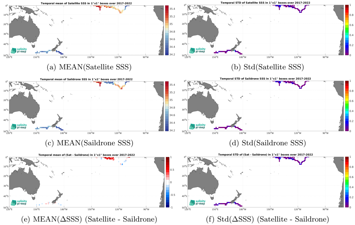
Figure 7: Temporal mean (left) and Std (right) of SSS from SMOS SSS L4 v1 - Daily (CMEMS-CNR) (top), Saildrone (middle), and of \Delta SSS (Satellite - Saildrone). Only match-up pairs are used to generate these maps.
