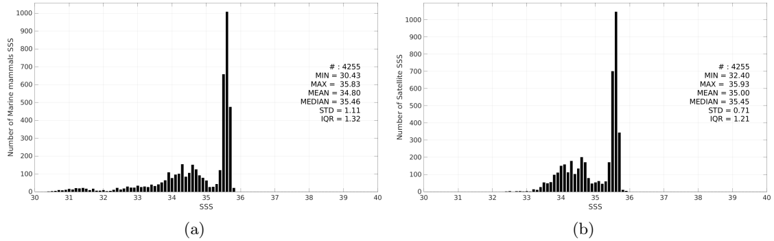
Figure 3: Histograms of SSS from Marine mammals (a) and SMOS SSS L4 v1 - Daily (CMEMS-CNR) (b) considering all match-up pairs per bins of 0.1 over the South Pacific Ocean Pi-MEP region and for the full satellite product period.
