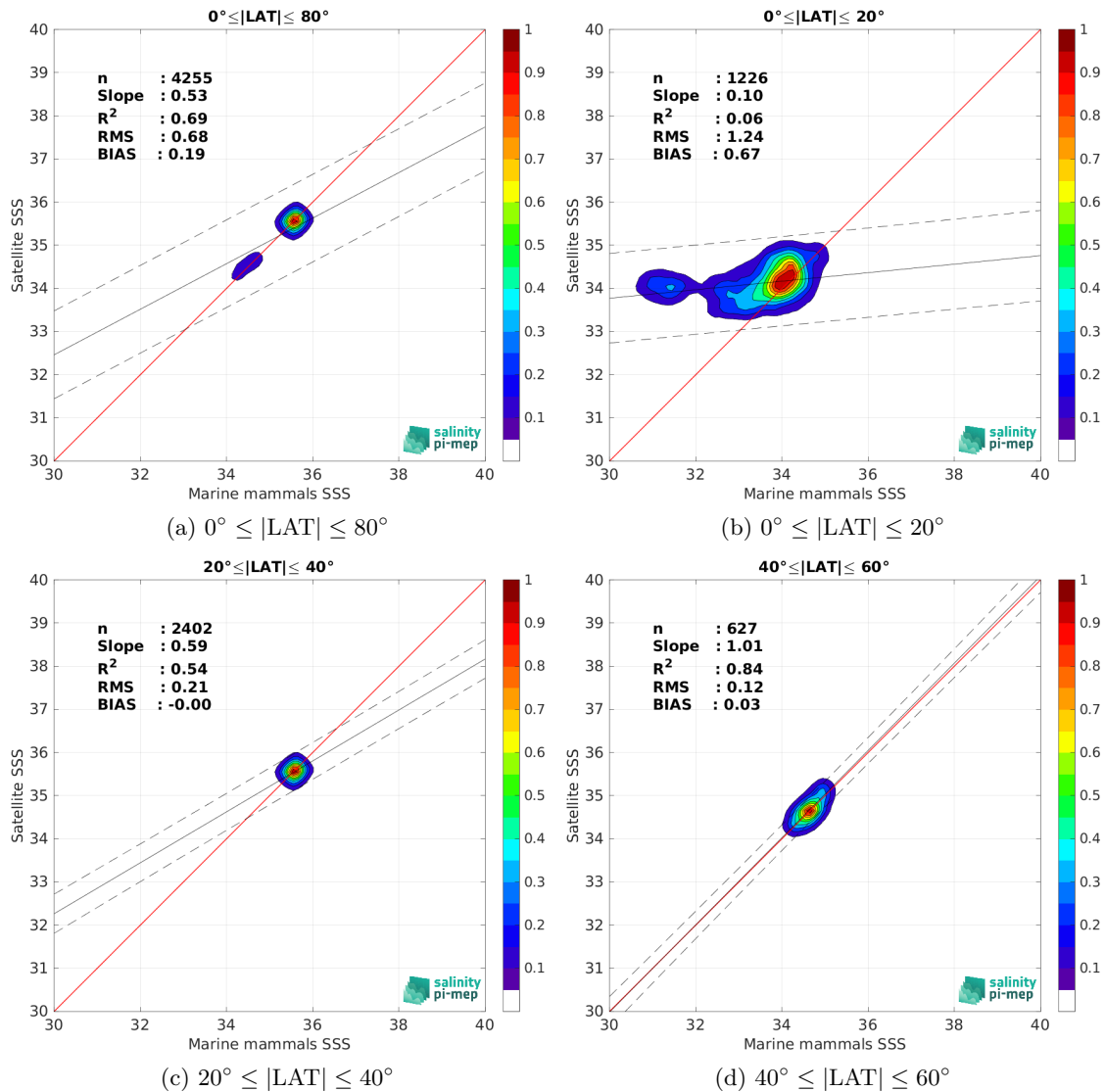
Figure 10: Contour maps of the concentration of SMOS SSS L4 v1 - Daily (CMEMS-CNR) SSS (y-axis) versus Marine mammals SSS (x-axis) at match-up pairs for different latitude bands. For each plot, the red line shows x=y . The black thin and dashed lines indicate a linear fit through the data cloud and the \pm 95\% confidence levels, respectively. The number match-up pairs n , the slope and R^2 coefficient of the linear fit, the root mean square (RMS) and the mean bias between satellite and in situ data are indicated for each latitude band in each plots.
