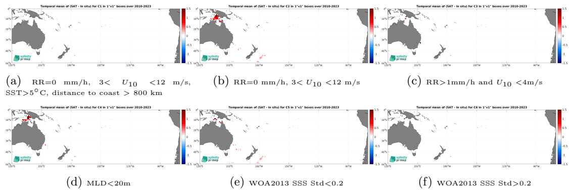
Figure 14: Temporal mean gridded over spatial boxes of size 1^\circ \times 1^\circ of \Delta SSS (SMOS SSS L4 v1 - Daily (CMEMS-CNR) - Marine mammals) for 6 different subdatasets corresponding to:RR=0 mm/h, 3 < U_{10} < 12 m/s, SST >5^\circ C, distance to coast > 800 km (a), RR=0 mm/h, 3 < U_{10} < 12 m/s (b), RR >1 mm/h and U_{10} < 4 m/s (c),MLD <20 m (d),WOA2013 SSS Std <0.2 (e),WOA2013 SSS Std >0.2 (f).
