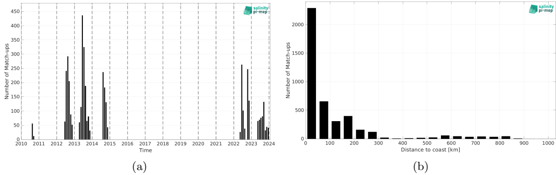
Figure 2: Number of match-ups between Marine mammals and SMOS SSS L4 v1 - Daily (CMEMS-CNR) SSS as a function of time (a) and as function of the distance to coast (b) over the South Pacific Ocean Pi-MEP region and for the full satellite product period.
