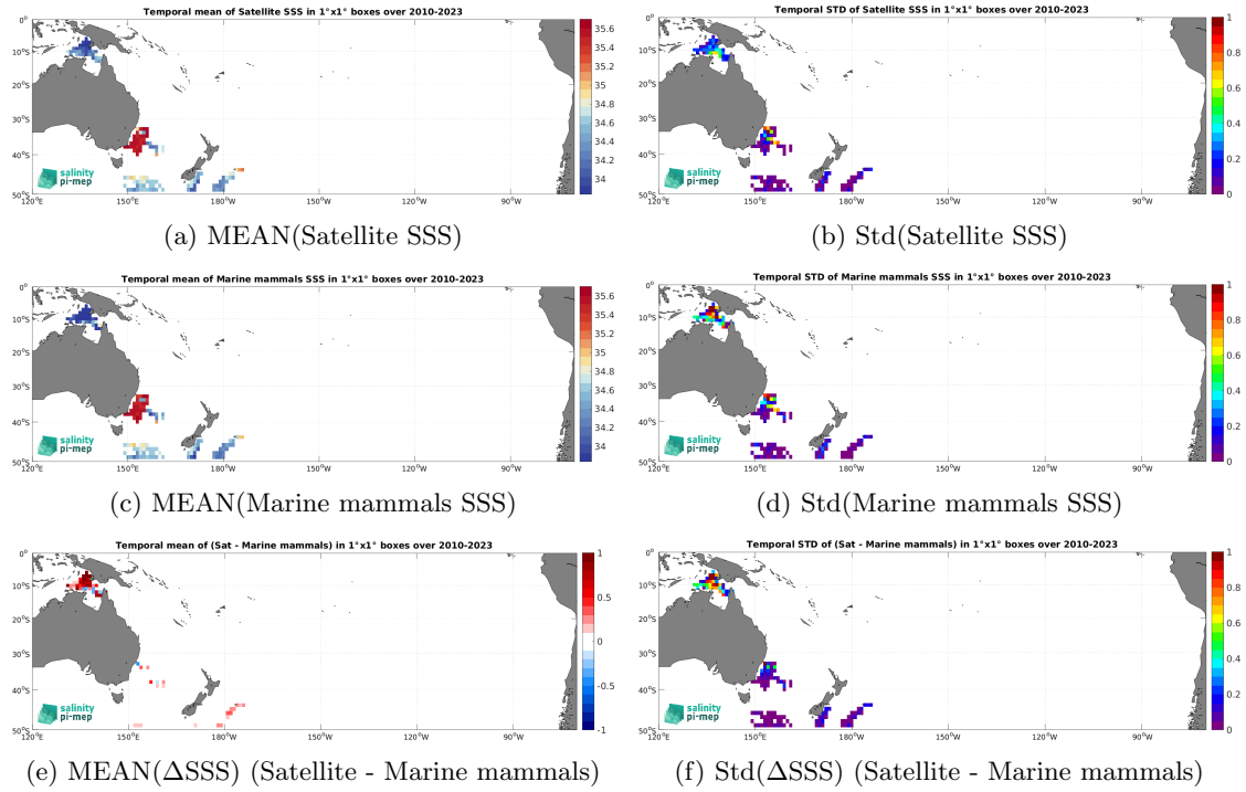
Figure 7: Temporal mean (left) and Std (right) of SSS from SMOS SSS L4 v1 - Daily (CMEMS-CNR) (top), Marine mammals (middle), and of \Delta SSS (Satellite - Marine mammals). Only match-up pairs are used to generate these maps.
